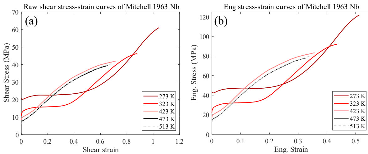
Figure 4.23: (a) Raw shear stress-shear strain curves and (b) calculated engineering stress-strain curves at different testing temperature and at a strain rate of 4.5 \times 10^{-5} \text{ s}^{-1} from [145].
