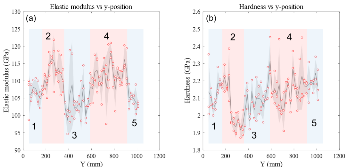
Figure 5.41: (a) Elastic modulus and (b) hardness as function of the vertical position in specimen 5-34 QS deformed at a nominal strain rate of 1.28 \times 10^{-2} \text{ s}^{-1} , with respect to the bottom of the indented area. The black line represents the median value at each height, the grey area is the standard deviation, and the red and blue areas are the approximate locations of the five bands.
