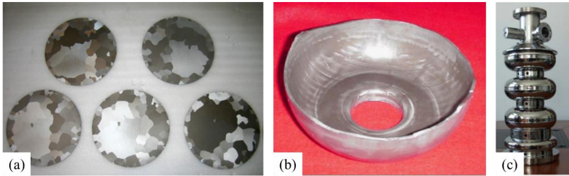
Figure 1.5: Large-grain niobium (a) disks produced at Tokyo Denkai, (b) half-cell deep drawn at JLab with earring defects and (c) 3.5-cell 1.3 GHz cavity manufactured at PKU [21], [29], [32].
