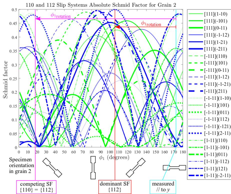
Figure 3.3: Schmid factors for all possible tensile orientations and 24 slip systems of a tensile test in grain two. The specimen orientation for the measured orientation (parallel to y in Figure 3.2b) and examples of orientations with competing or dominant Schmid factors are shown.
