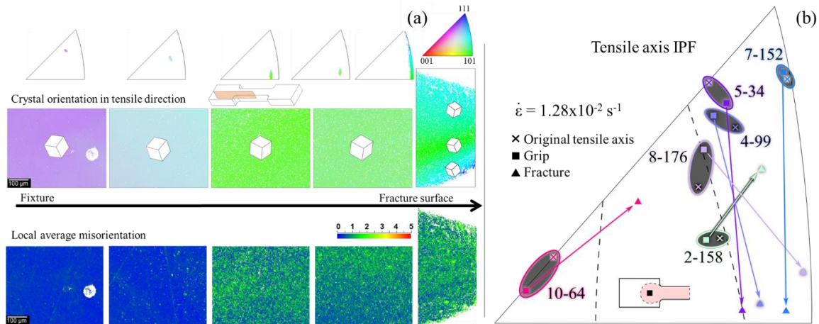
Figure 5.14: (a) EBSD orientation map in the tensile direction and misorientation of specimen 8-176 with an initial crystallographic orientation near the center of the IPF deformed in tension at 1.28 \times 10^{-2} \text{ s}^{-1} . (b) Orientations in the grip (square), near the fracture surface (triangle) and theoretical (crosses) for six specimens deformed at low strain rates. A half-specimen schematically shows the location of the grip measurement and possibly deformed region within the grip in light red [176].
