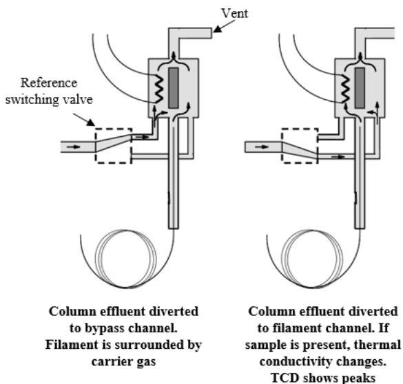
Figure 3.10: TCD principle
