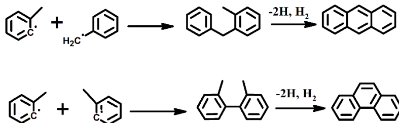
Scheme 4.11: Reaction pathways starting from toluene radicals leading to C_{14}H_{10} isomers
