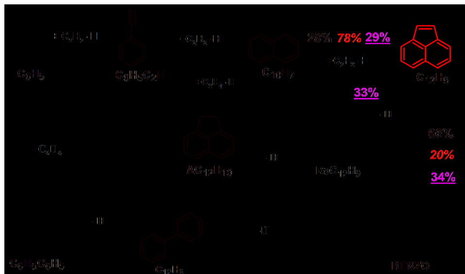
Scheme 5.4: The reaction pathways leading to acenaphthylene formation at T_5 of 1500 K in the pyrolysis of benzene and benzene/ C_2 binary mixtures. The percentage numbers (B: black normal; BA: red italic; BE: purple underlined) represent the contributions of the corresponding reactions in naphthalene formation. The dashed arrows represent multi-step reactions.
