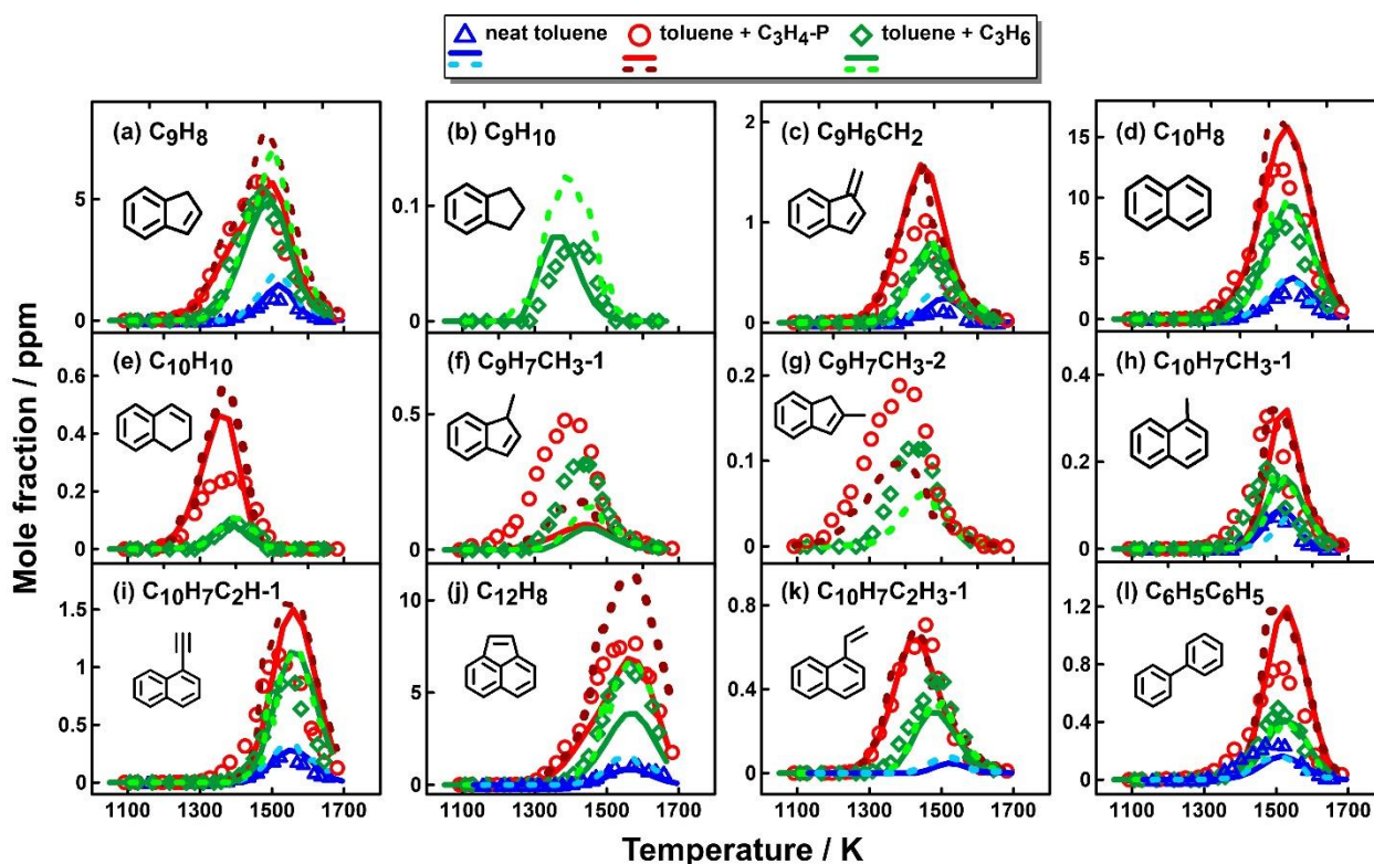
Figure 5.69: C 9 -C 12 PAH mole fraction profiles as a function of the post-shock temperature T 5 in neat toluene, toluene + C 3 H 6 and toluene + C 3 H 4 -P pyrolysis. Symbols: measurements; solid lines: simulations with a constant pressure of 20 bar within a reaction time of 4.0 ms; dashed lines: simulations with measured pressure histories up to 10 ms.
