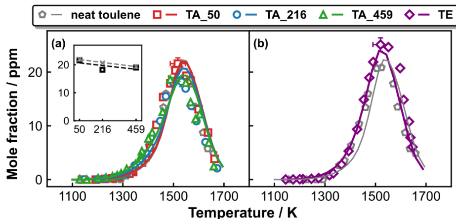
Figure 5.50: Experimental (symbols) and modeling (solid lines) benzene ( C_6H_6 ) mole fractions as a function of the post-shock temperature T_5 in (a) toluene/ C_2H_2 pyrolysis and (b) toluene/ C_2H_4 pyrolysis. The inset in (a) plots the measured (dark open square) and simulated (gray cross) C_6H_6 peak concentrations against the initial C_2H_2 contents; linear regressions (the dashed lines) of the data points are shown as a visual guide. Simulated and experimental C_6H_6 mole fractions in neat toluene (105 ppm in argon) pyrolysis are also shown as a reference.
