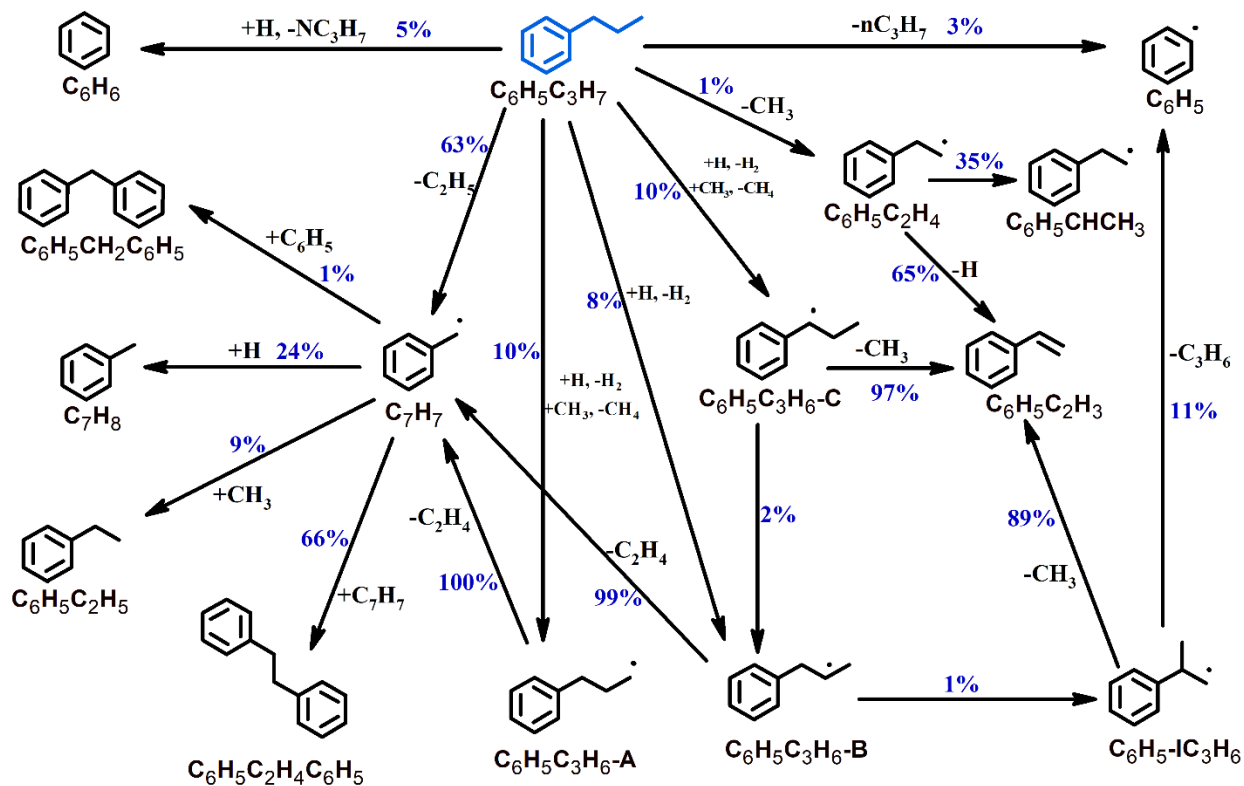
Scheme 5.16: Fuel consumption pathways in n-propylbenzene pyrolysis based on integrated ROP analysis at 1150 K. The percentage numbers are the contributions by the corresponding reactions to the consumption of the species on the source side.
