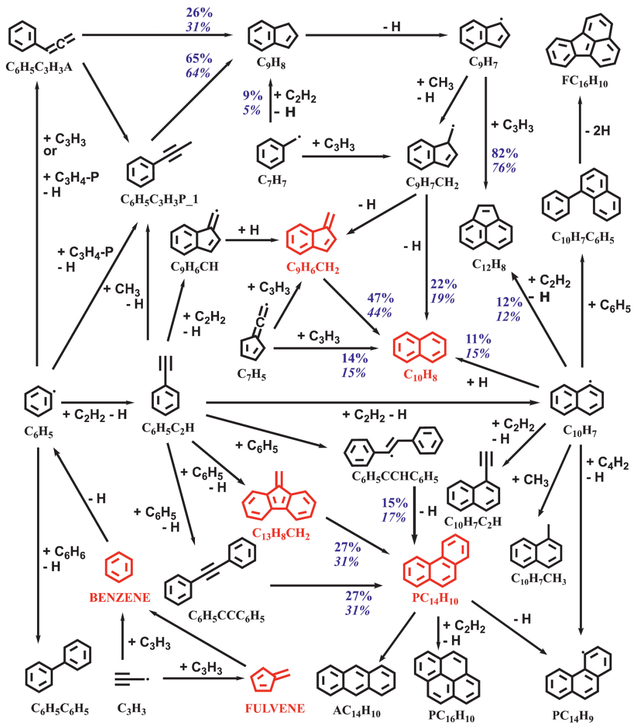
Scheme 5.2: Major PAH formation pathways in propylene and propyne pyrolysis based on ROP analyses at 1550 K. The percentage numbers (normal font: in propylene pyrolysis; italic font: in propyne pyrolysis) represent the contribution of corresponding reactions to the formation of important PAHs.
