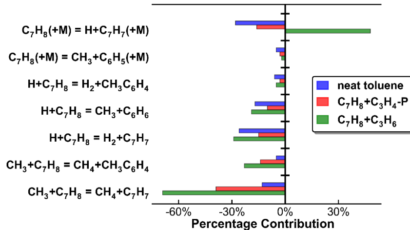
Figure 5.66: Integrated ROP-analyzed percentage contributions of toluene consumption in the pyrolysis of neat toluene and toluene/ C_3 binary mixtures at 1400 K.
