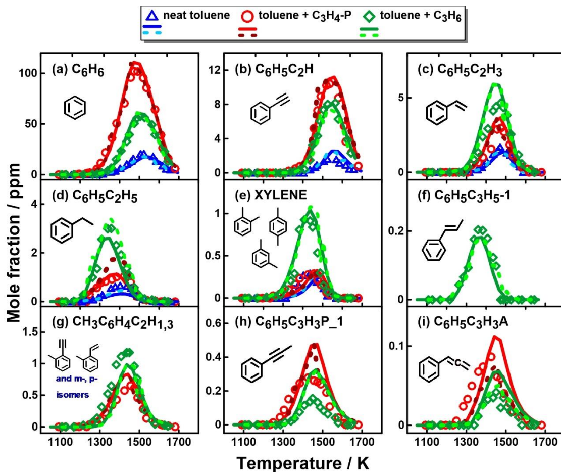
Figure 5.68: MAH mole fraction profiles as a function of the post-shock temperature T_5 in neat toluene, toluene + C_3H_6 and toluene + C_3H_4-P pyrolysis. Symbols: measurements; solid lines: simulations with a constant pressure of 20 bar within a reaction time of 4.0 ms; dashed lines: simulations with measured pressure histories up to 10 ms.
