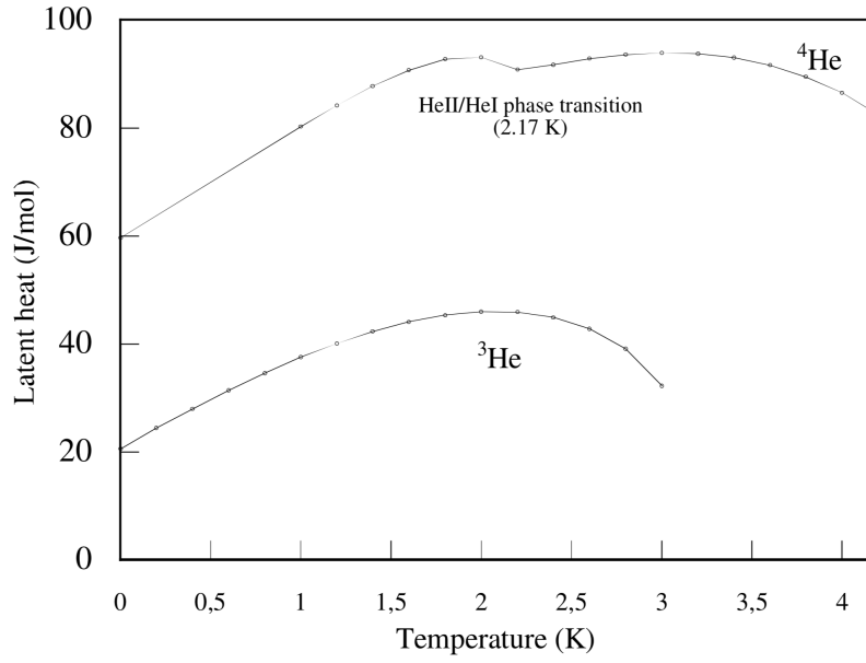
Figure 2.2: Variation of the latent heat of 4 He and 3 He at low temperature. [73]
