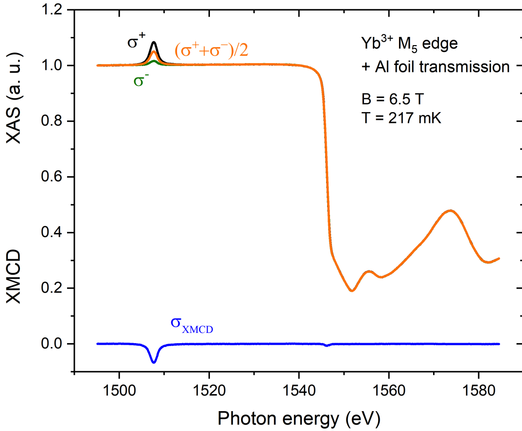
Figure 6.10: XAS-XMCD measurements of Yb- M_5 edge (1507.5 eV) at T = 217 mK and B = 6.5 T. The structure from 1550 eV to 1580 eV is the Al-K edge measured in transmission of the inserted aluminum foil between the beam and the sample served as a normalization reference between different series of measurement.
