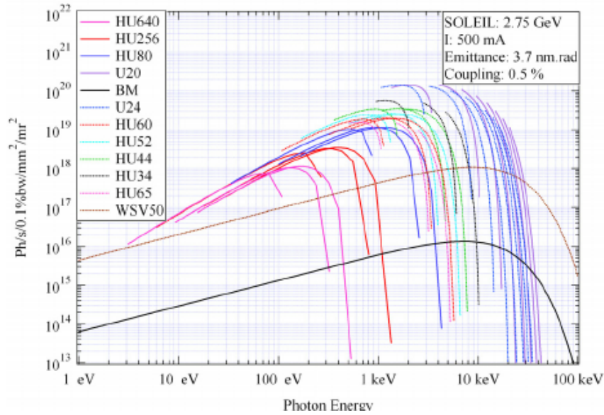
Figure 3.1: SOLEIL synchrotron radiation spectral range for the various insertion devices. BM for bending magnets, HU and U for undulators and WSV for wigglers. (Figure from [103].)
