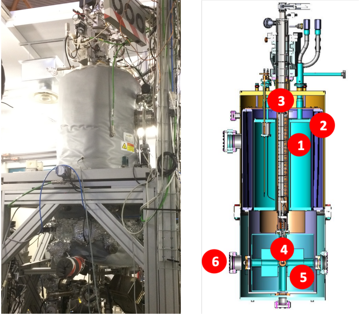
Figure 2.8: (Left) The CroMag cryomagnet on endstation of DEIMOS beamline. (Right) Scheme of the CroMag cryomagnet. (1) Main reservoir of ^4\text{He} liquid. (2) Anti-cryostat of liquid nitrogen. (3) Dilution VTI. (4) Still, mixing chamber and sample holder. (5) Superconducting magnet. (6) Entrance of the X-ray. (DEIMOS - Synchrotron SOLEIL)
