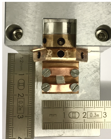
Figure 5.4: \text{Er}_{0.025}\text{Pd}_{0.975} sample mounted on the sample holder of DEIMOS beamline with the measures of the dimension.
