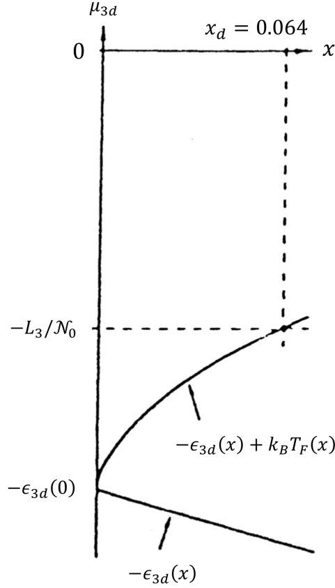
Figure 2.5: Variation of the chemical potential \mu_{3d} as a function of the ^3\text{He} mole fraction x at T = 0 K. [89]
