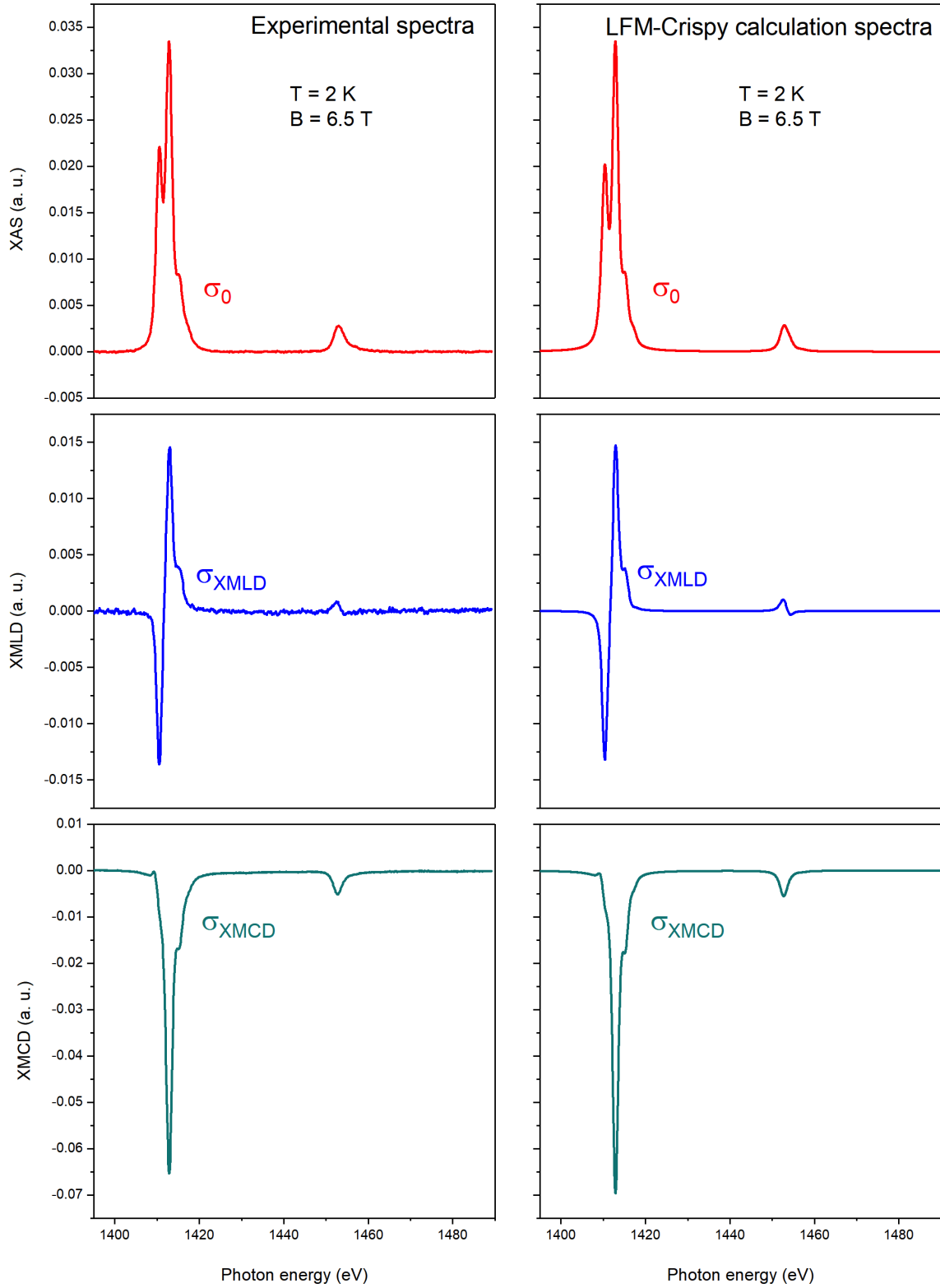
Figure 5.11: Experimental isotropic, XMMLD and XMCD spectra recorded at T = 2 K and B = 6.5 T compared to the LFM-Crispy calculations with crystal parameters B_{40} = 11.3 meV and B_{60} = -3 meV at the same temperature and magnetic field.
