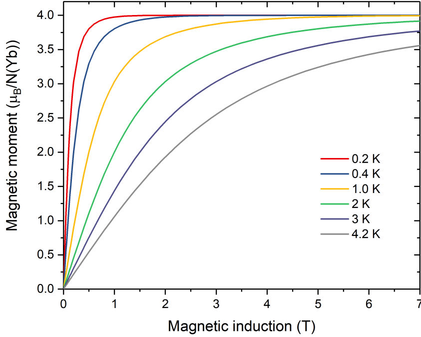
Figure 6.1: Evolution of the magnetic moment of a spherical \text{Yb}^{3+} ion as a function of an external magnetic induction and for temperatures between 0.2 K and 4.2 K.
