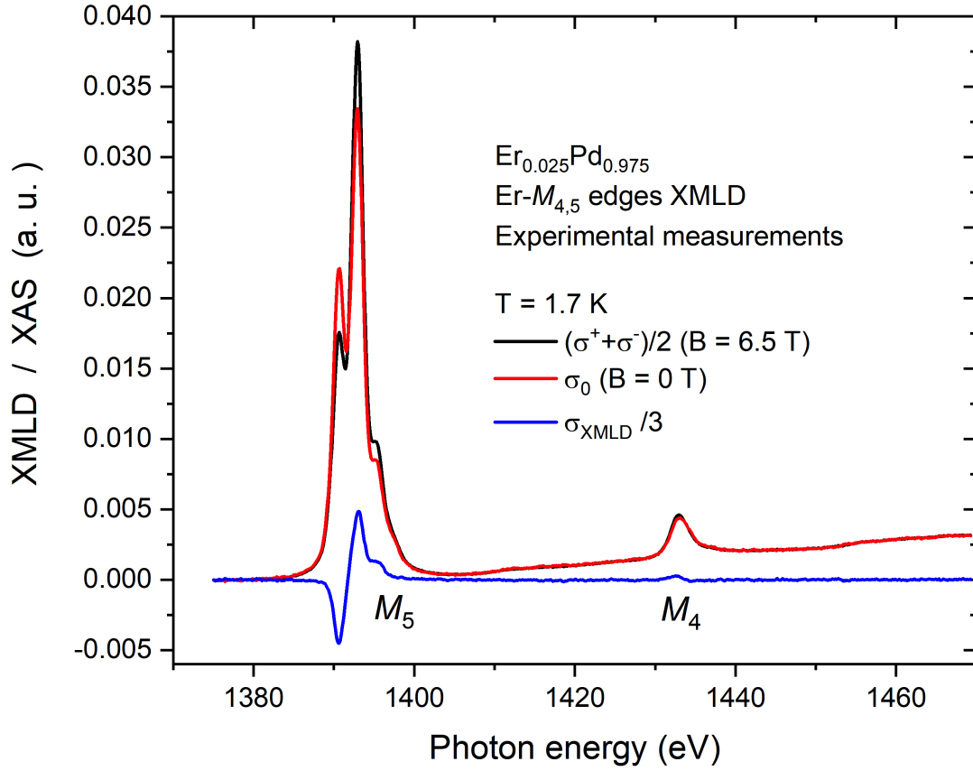
Figure 5.8: Er 3+ -M 4,5 XAS and XMLD spectra at 1.7 K. The black spectrum is the average of the two phase \sigma^+ and \sigma^- and the isotropic (red) spectrum is recorded without magnetic field. The blue spectra is the difference between the black and the red spectrum applying (Eq. 5.11) which is, by definition, one third of the XMLD signal.
