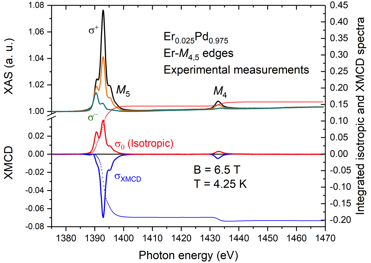
Figure 5.7: XAS-XMCD measurement of the \text{Er-M}_{4,5} of the \text{Er}_{0.025}\text{Pd}_{0.975} sample at 4.25 K with an external magnetic field of 6.5 T. The black spectrum is the average of the spectra \sigma^+ , the green spectrum is the average of the spectra \sigma^- . The average of the green spectrum and the black one gives the \frac{\sigma^+ + \sigma^-}{2} spectrum in orange. The red isotropic spectrum \sigma_0 is recorded without magnetic field and the background baseline has been removed. The green spectrum minus the black spectrum gives the XMCD spectrum in blue. The red dotted line is the integral of the red isotropic spectrum and the blue dotted line is the integral of the XMCD spectrum. The two integrals start from zero and stabilize at the end which prove a good deletion of the background.
