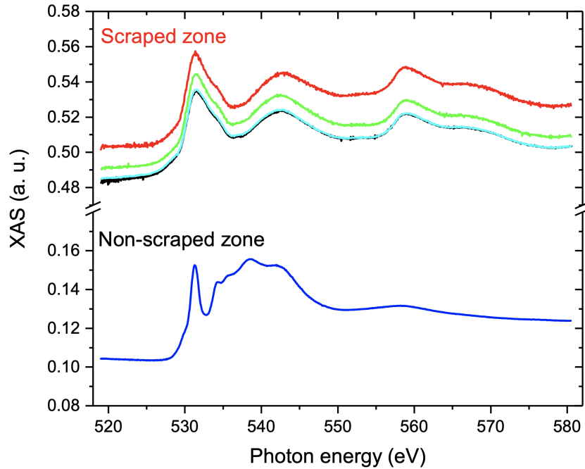
Figure 5.6: XAS measurements at \text{Pd-M}_{2,3} edges in different points of the scraped zone compared to a measure in a non-scraped zone.
