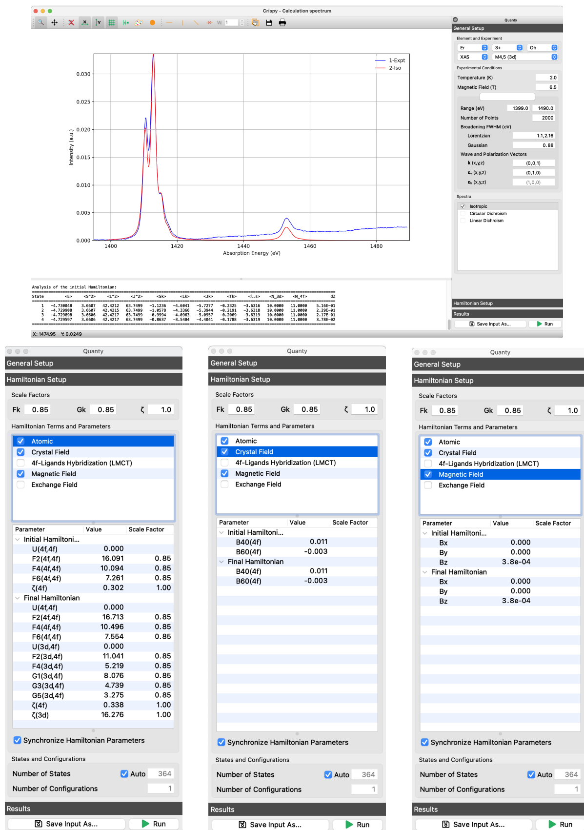
Figure 4.1: In using Crispy for LFM calculations. (Top) Crispy main window showing the experimental data (Spectrum 1-Expt) compared to the simulated XAS spectrum (spectrum 2-Iso) of \text{Er}^{3+} with the configurations displayed (Bottom).
