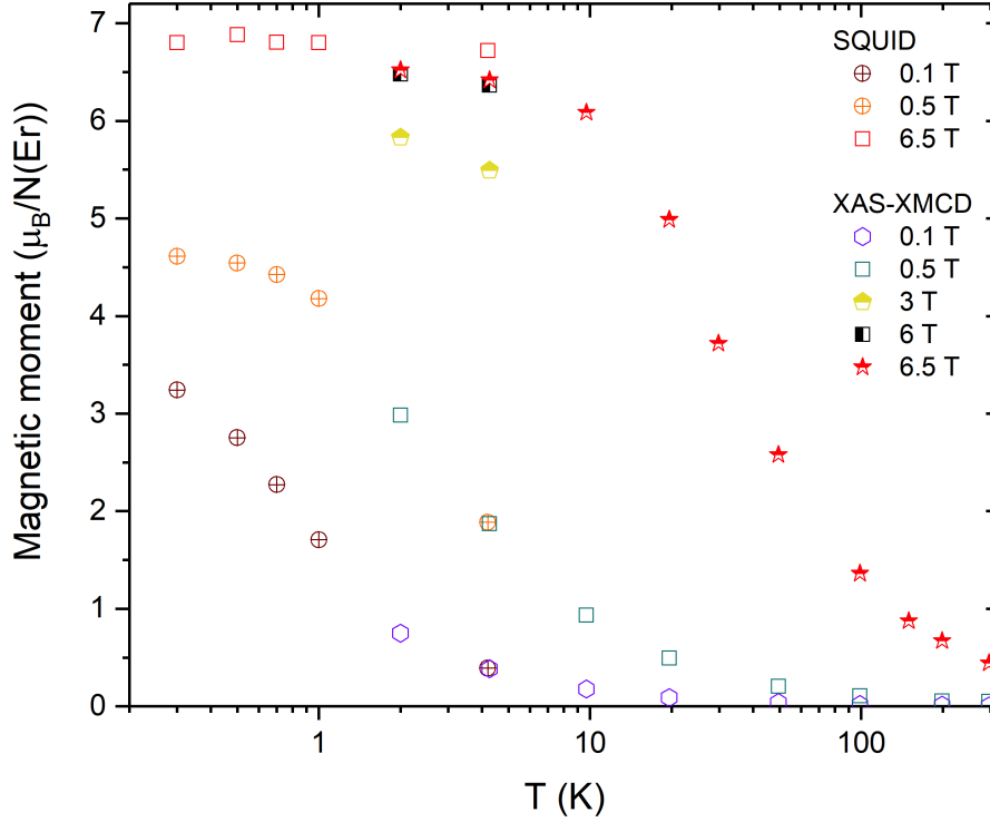
Figure 5.12: Evolution of the magnetic moment as a function of temperature for Er 3+ ion measured by SQUID and XAS-XMCD. T is presented in a logarithmic axis.
