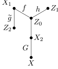
Figure 3.6: The adjacency of the homothety classes constructed in the first case of Lemma 3.4.7.
