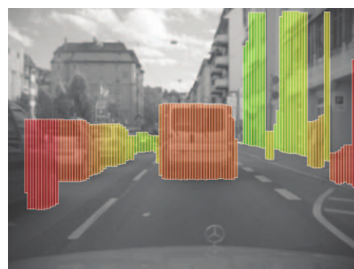
(c) Stixel representation from [Pfeifer and Franke - 103].
