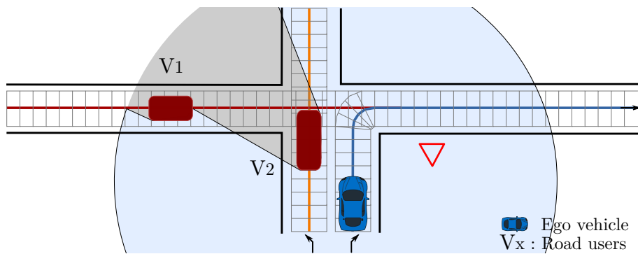
Figure 3.19: LGM example with perception occupancy information. Occupancy is represented by a polygon approach: free space (blue), objects (red).
