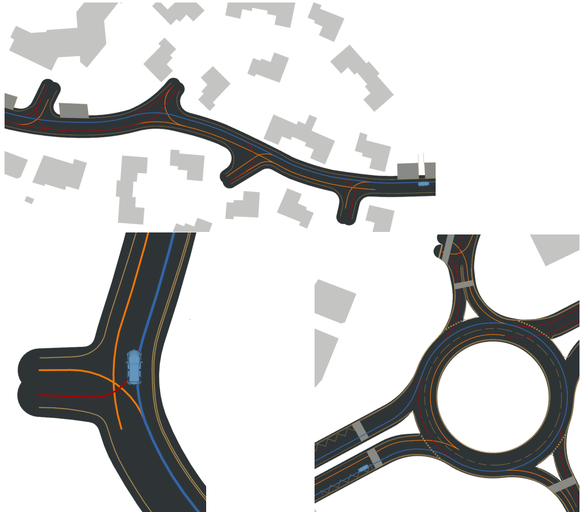
Figure 3.6: Interaction Graph models in a real-time experiment led in Compiègne. The ego-vehicle is represented in blue. The primary order lane keeping paths is represented by the blue center-line. Other primary order paths are shown in red. Secondary order paths are in orange. For visual convenience, lane changing primary order paths are not displayed. Furthermore, some paths may be both primary and secondary but are represented with only one color. (The buildings are displayed in gray)
