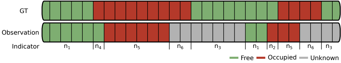
Figure 3.12: Correspondence between evaluation parameters and the LGM of both the observation and the ground truth (GT).
