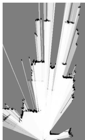
(a) Occupancy grid from [Negre et al. - 97].
