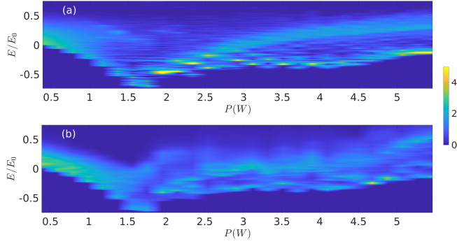
Figure 9.13 – Energy distribution map a for simulation (top) and the experiment (bottom). The energy axis is in units of E_0 = (2\pi\kappa) / (\alpha\beta k_0 P) .
