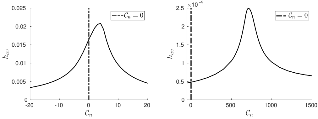
Figure 6.1 – Average time-step h_{av} = \frac{1}{N_h} \sum_{n=1}^{N_h} h_n with a constant C_n for the IF method applied to the one dimensional NLS (left) and SN (right) equations.
