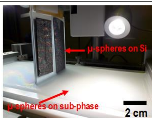
Figure II-16: Langmuir-Blodgett deposition process.
