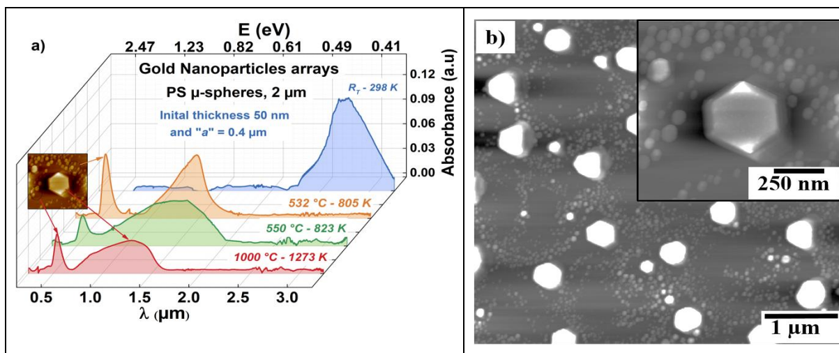
Figure III-13: Effect of the thermal treatment on Au nanoparticle arrays deposited on an Al_2O_3 -c substrate and made with 2 \mu m polystyrene microspheres. a) Absorbance spectrum pointing out the wavelength blue shift. b) Au nanoparticle array made with 2 \mu m polystyrene microspheres and thermally treated at 1000^\circ C ( 1273 K ).
