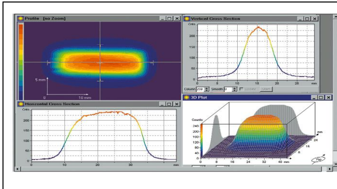
Figure Appendix 9 : Near field beam profile of an excimer laser [205].
