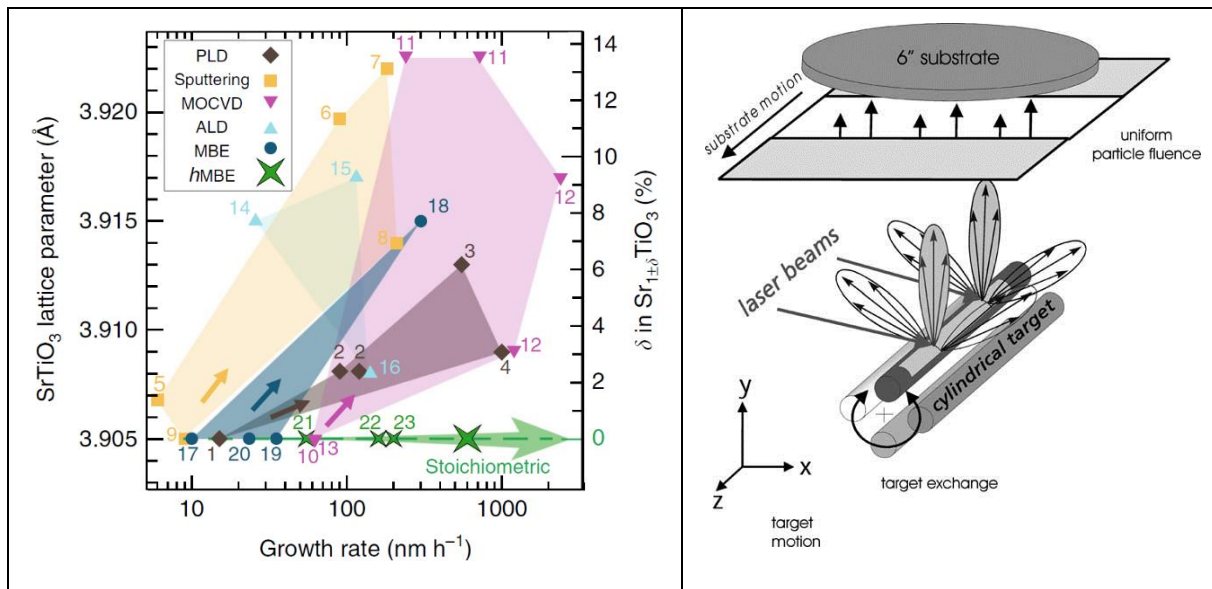
Figure II-3: Control of thin film stoichiometry and growth rate by different deposition techniques. The number close to data points shown refer to references, for more details see [87].
