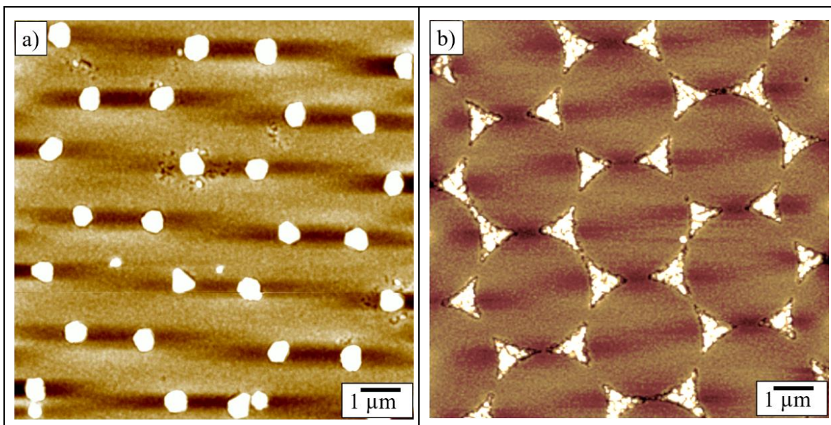
Figure IV-4: AFM image of metallic nanoparticle array embedded into a 200nm- \text{VO}_2 matrix. a) gold nanoparticle arrays. b) Iridium nanoparticle arrays. The initial thickness of the Au and Ir made with 3 \mu\text{m} polystyrene microspheres nanoparticles is 50 nm.
