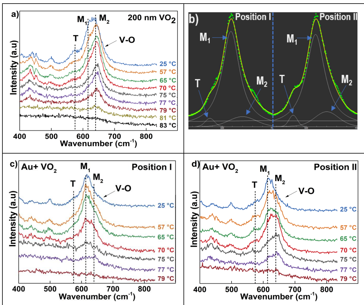
Figure V-16: The evolution of Raman spectra as a function of temperature. a) Temperature dependence of Raman spectra of 200 nm VO 2 thin films. b) Example of a fit used to extract the VO 2 phases from Raman measurements. c) Temperature dependence of Raman spectra from Position “I” of 200 nm of VO 2 containing Au nanoparticle arrays. d) Temperature dependence of Raman spectra from Position “II” of 200 nm of VO 2 containing Au nanoparticle arrays. The Raman data are acquired during heating up.
