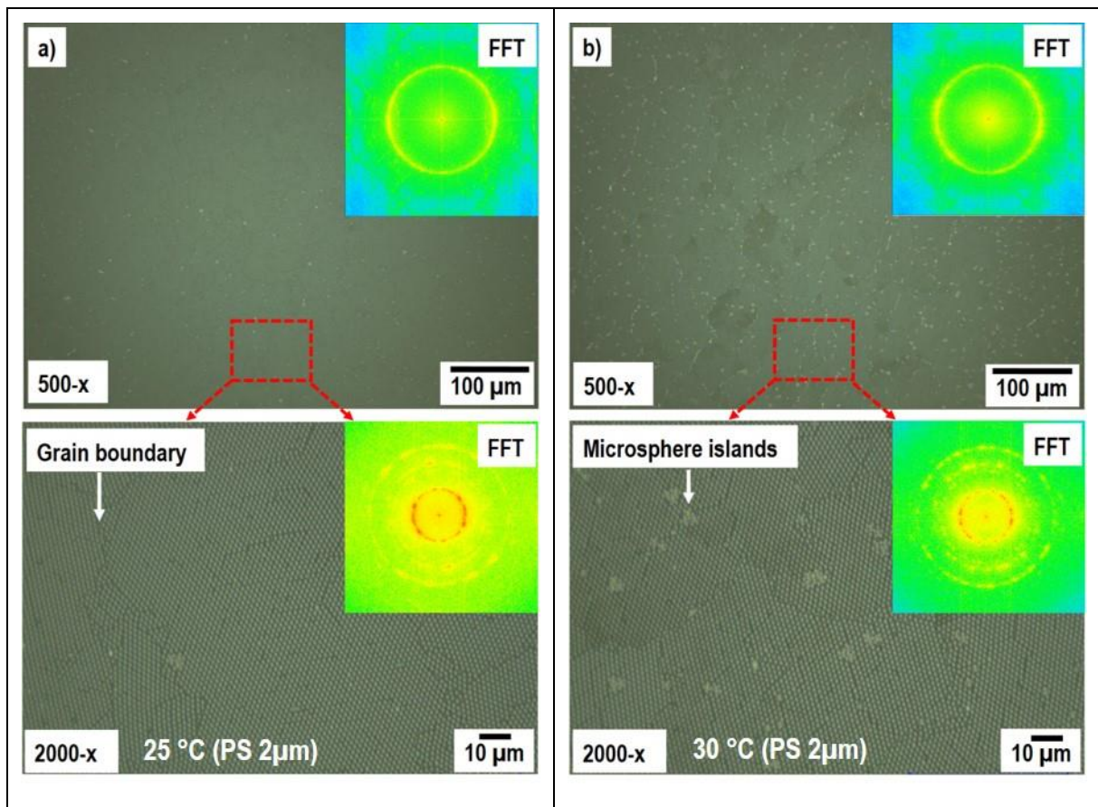
Figure II-25: Optical images at 500-x and 2000-x magnification of polystyrene microspheres 2 µm deposited on Al_2O_3 -c at a) 25 °C, b) 30 °C. The inserts represent the FFT (for 500 -x and 2000-x respectively).
