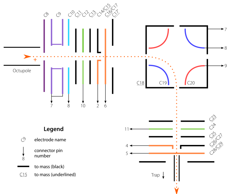
FIGURE II.2: Electrical layout of guiding elements from the exit of octupole until the tube separating the creation chamber at 10^{-6} mbar to the GICD vessel at 10^{-9} mbar.
