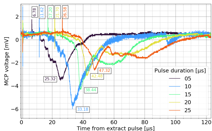
FIGURE 7.4: MCP signal for several extraction pulse durations. The framed numbers indicate the time for specific points. The pulses are triggered 0.9 μs after time origin. The molecular ion is TRP.
