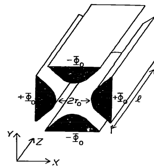
FIGURE 1.1: Linear trap design from Campana [Cam80], with hyperbolic surfaces. \Phi_0 is the applied electric voltage, r_0 the inscribed radius between the electrodes, and l the length of the rods.
