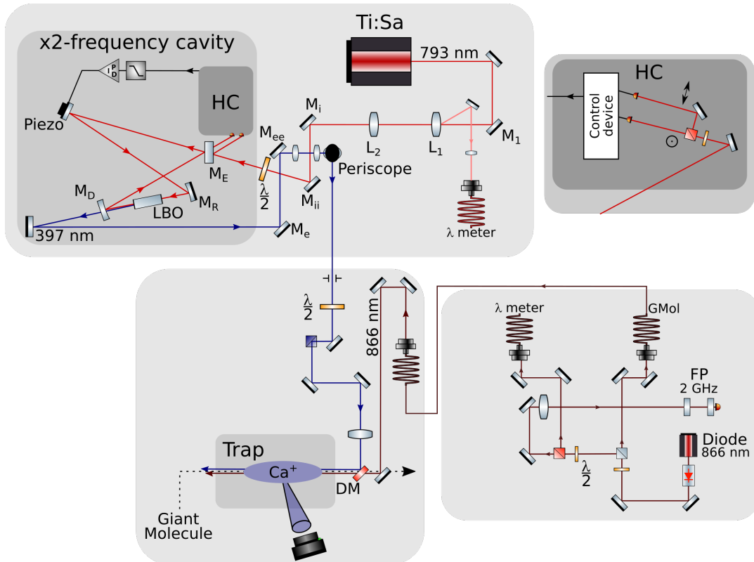
FIGURE 4.7: Schematics of the optical part of the experiment. M is for mirror, L for lens, DM for dichroic mirror, \lambda/2 and yellow rectangles are for half-wave plates. HC is for Hänsch-Couillaud, \lambda meter for the wavelength measuring device. FP is for Fabry-Pérot interferometer with 2 GHz FSR. ComponentLibrary by Alexander Franzen is licensed under a Creative Commons Attribution-NonCommercial 3.0 Unported License.
