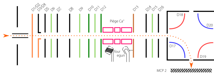
FIGURE II.3: Electrical layout of guiding elements in the detection chamber at 10^{-9} mbar.
