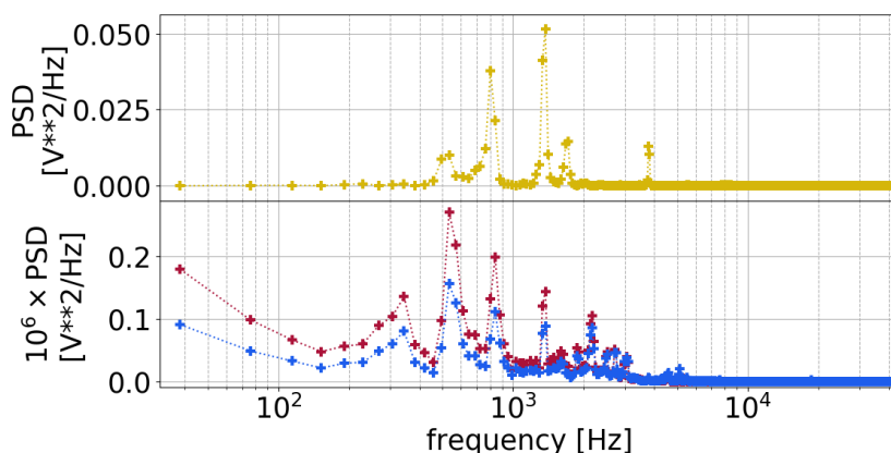
FIGURE 4.10: Power spectral density of the three signals from error signal and laser photodiodes.
