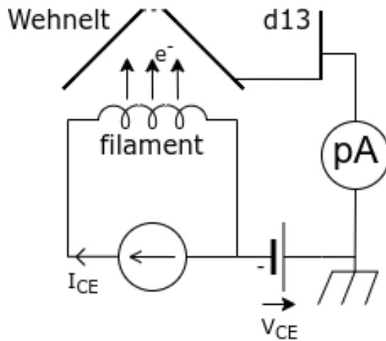
FIGURE 4.12: Electrical layout of the electron gun, and position of the picoAmperemeter during the characterisation of the electron gun. The Wehnelt is a conical shaped electrode with an aperture along its main axis for the accelerated electrons to go through. d13 refers to an electrode according to the layout presented in part II, it is connected to the Wehnelt.
