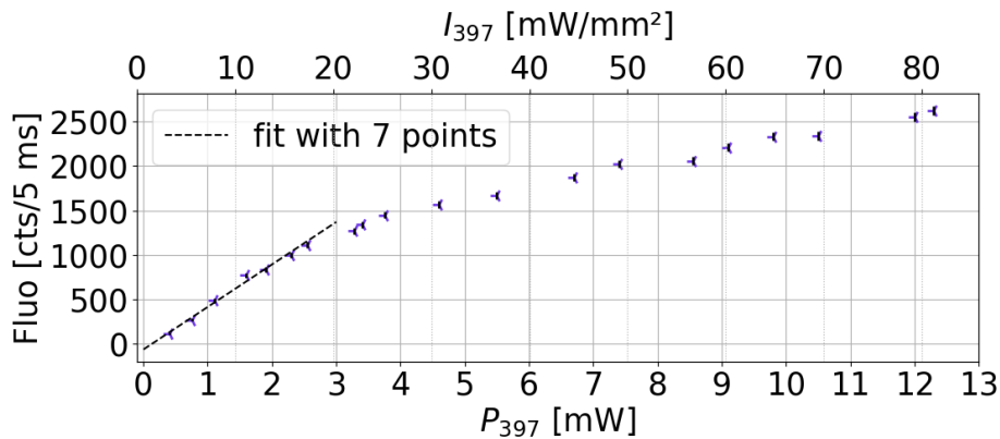
FIGURE 4.14: Fluorescence of an ion cloud against 397 nm cooling laser power, error bars in black. The 866 nm laser power is P_{866} = 1 \text{ mW} . A linear fit is done with the first seven points satisfying a linear variation at sight, before saturation sets in.
