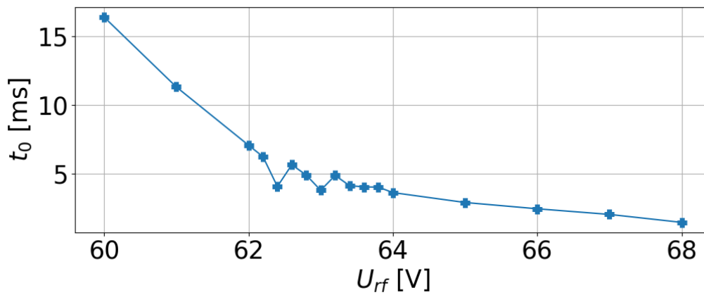
FIGURE 9.16: Critical timing t_0 deduced from the fit, as a function of U_{RF} for 17 conditions, using computer program RF HEATING, U_{DC} = 7 V, 1024 ions. The blue line only links the neighbour data points.
