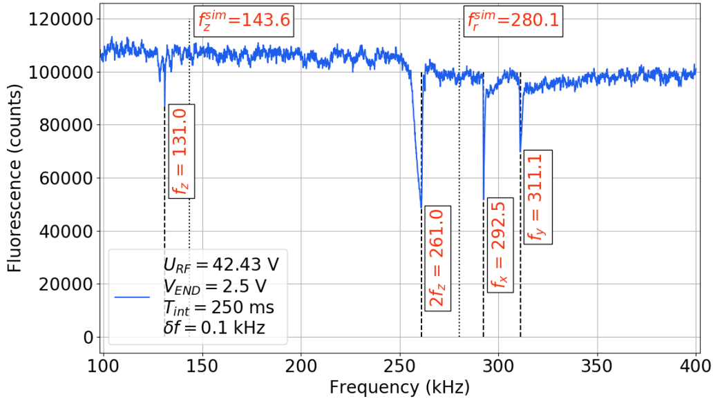
FIGURE 2.2: Tickle frequency response of a trapped ion cloud under constant trapping field amplitude. The fluorescence is integrated over 250 ms, the background light level is at 13000 counts at this integration time. The frequency resolution is \delta f_{\text{tickle}} = 0.1 kHz.
