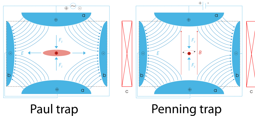
FIGURE I.2: Left : Paul Quadrupole ion trap of classical setup with a particle of positive charge (dark red), surrounded by a cloud of similarly charged particles (light red). The electric field E (blue) is generated by a quadrupole of end caps (a, positive) and a ring electrode (b). Right : Penning Trap for the storage of charged particles by the use of a constant electric field (blue), generated by a quadrupole (a, end caps) and (b, ring electrode) and a superposed constant and homogeneous magnetic field (red), generated by a surrounding cylinder magnet (c). A particle, indicated in red (here positive) is stored in between caps of the same polarity.
