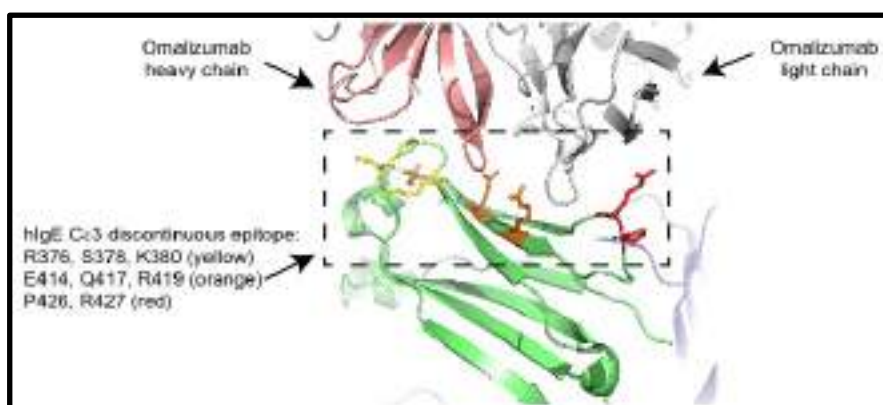
Figure 9. The IgE C \epsilon 3 epitope for Omalizumab (analysis of the crystal structure PDB 5HYS)
