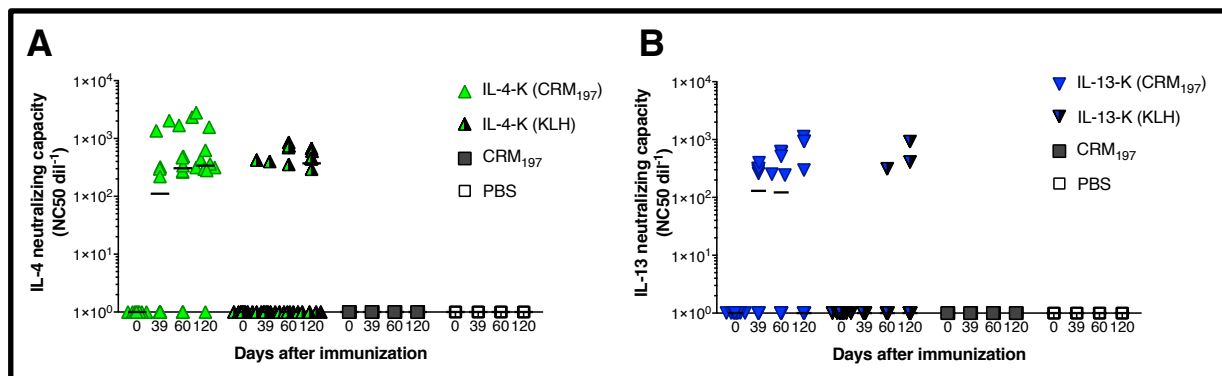
Figure 7. Immunogenicity study using different carrier proteins. (A) Anti IL-4 neutralizing capacity and (B) anti IL-13 neutralizing capacity in sera from mice immunized with IL-4-K or IL-13-K respectively prepared with CRM 197 or KLH as carrier protein. Intramuscular injections were done at days 0, 7, 28 and 48 in emulsion with SWE adjuvant. Two control groups were included where mice were immunized with CRM 197 in emulsion (1:1) with SWE or PBS, following the same immunization schedule. 10 mice/group or 5 mice/control groups.
