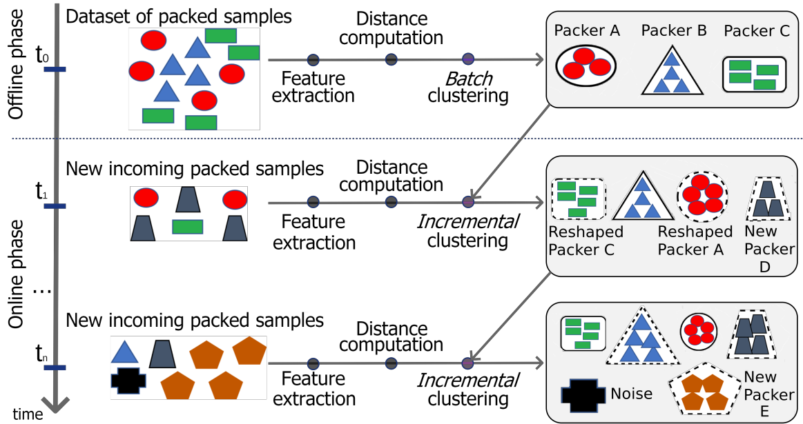
Figure 4.1 – Overall toolchain.
