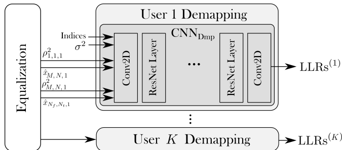
Figure 5.11: CNN-based uplink demapper.
