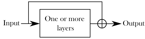
Figure 2.14: A residual connection.
