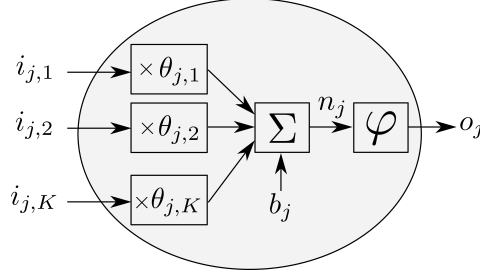
Figure 2.10: Representation of an artificial neuron.
