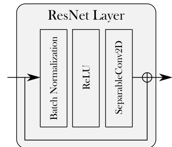
Figure 5.12: ResNet layer.
