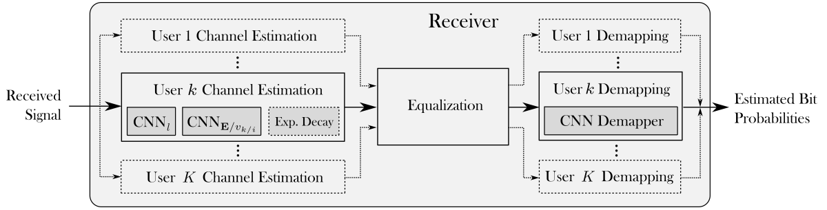
Figure 5.6: DL-enhanced receiver architecture. The dotted elements are only present in the uplink, where the BS jointly processes all users. The dark gray elements are trainable components.
