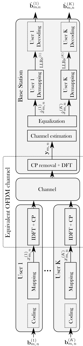
Figure 2.6: An uplink MU-MIMO system.
