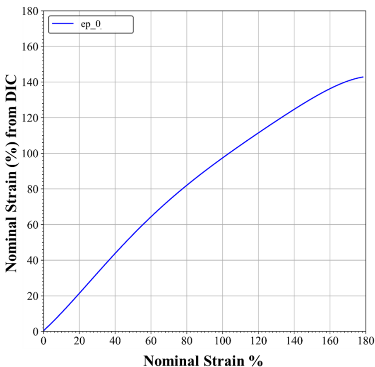
Figure 8 a): Comparison of Nominal strain obtained using DIC vs nominal strain obtained by mechanical extensometer.
