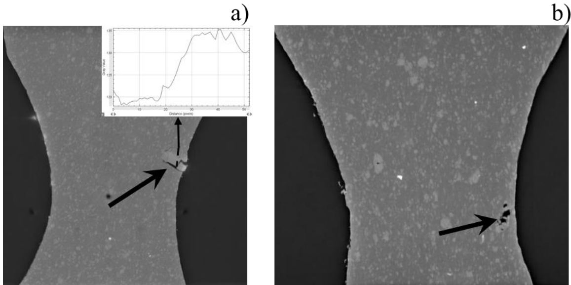
Figure A8: Slice images showing critical defects. The defects pointed in the images are \text{CB}_{\text{aggl}}
