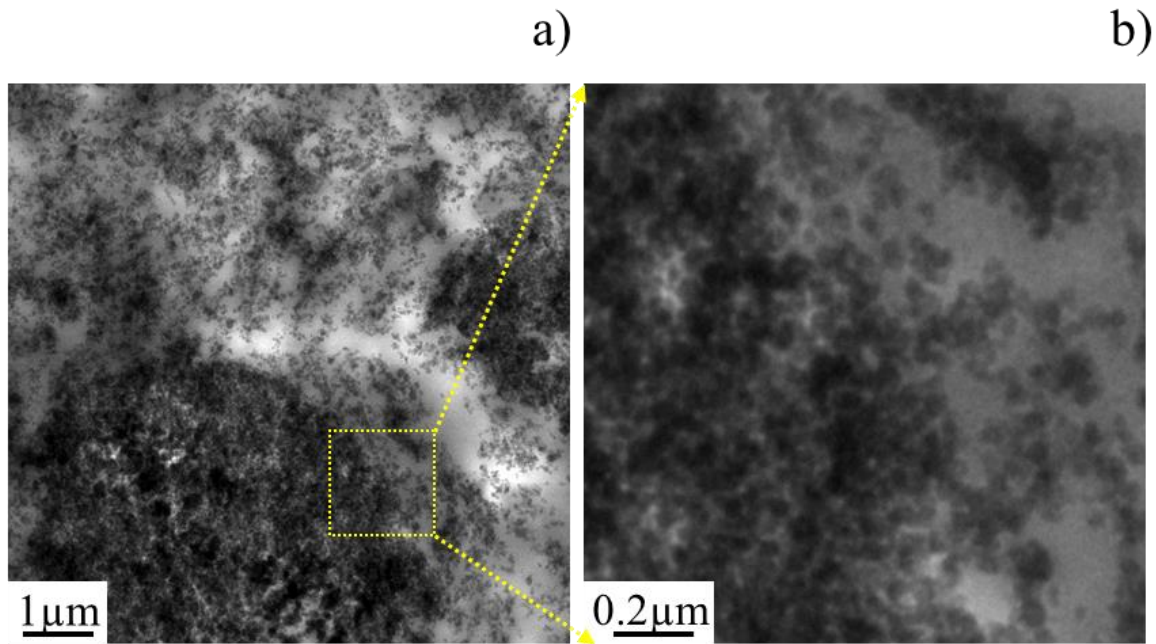
Figure 3: a) TEM image of a slice of CB_{aggl} in F1 at a resolution of 1\mu\text{m} , b) zoomed portion of the yellow square in 'a)' at a resolution of 200\text{nm} .
