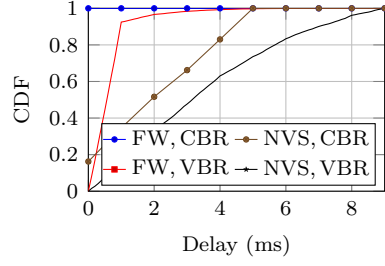
(a) CDF for CBR and VBR traffic.
