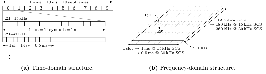
Figure 2.5 – The 5G/NR physical layer structure.
