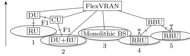
(a) Underlying RAN network functions below FlexVRAN.
