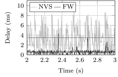
(b) Packet delays over 1 s simulated time for VBR traffic.
