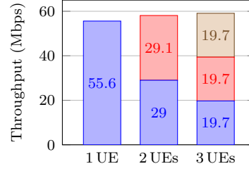
Figure 6.22 – 5G DL throughput fairness for multiple UEs.
