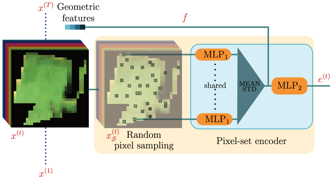
Figure 1.6: Pixel-Set Encoder. First, a fixed number of pixels is randomly drawn from the input image x^{(t)} . These pixels, x_s^{(t)} , are encoded with the shared \text{MLP}_1 . The resulting set of vectors is pooled into a single vector that is in turn encoded by \text{MLP}_2 , which outputs the final embedding e^{(t)} of the input image. We also concatenate some geometrical descriptors f of the parcel’s shape before \text{MLP}_2 , as it can be a relevant information for crop type classification.
