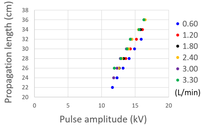
Figure 3.21 The TR plasma propagation length versus pulse amplitude with given argon gas flow rate (pulse width: 1500ns and frequency: 265 Hz).
