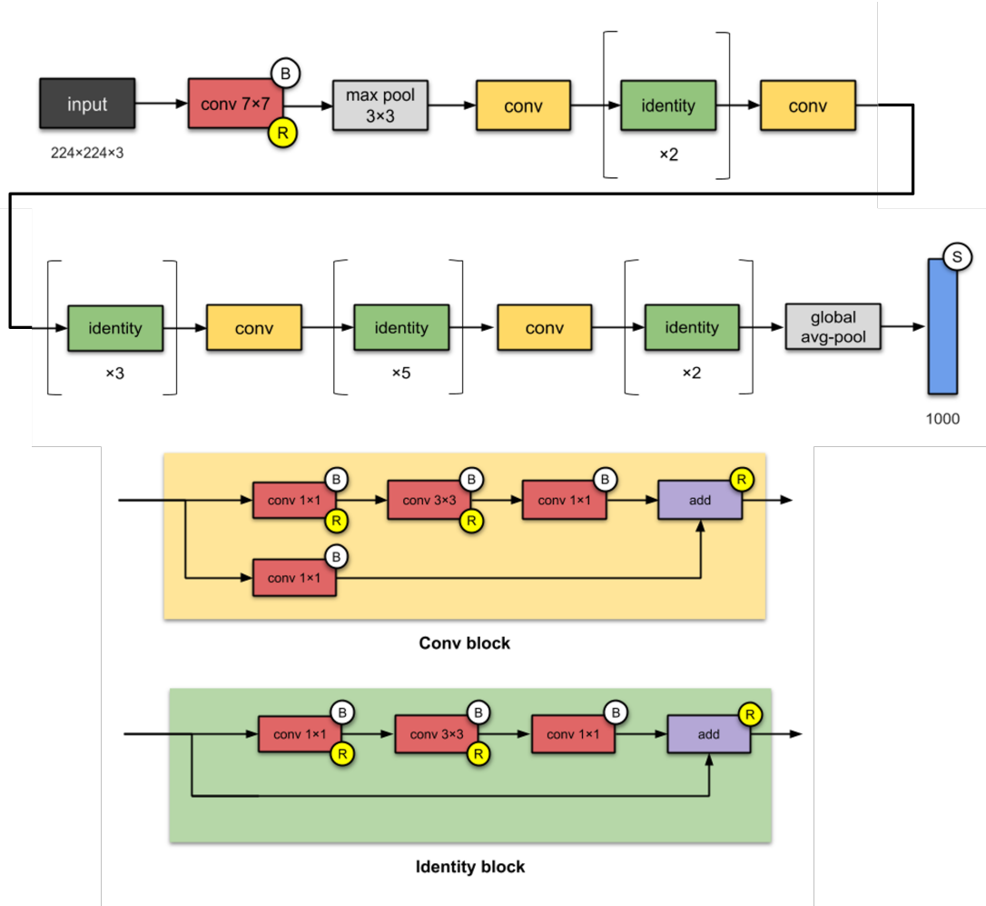
Figure 4.2: Illustration of ResNet50's architecture from [Karim, 2019]. Symbol B stands for Batch-norm layer, R stands for ReLU activation function and S represents Softmax.
