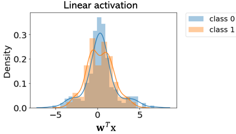
Figure 7.6: The distribution of \mathbf{w}^T \mathbf{x} for each class for a network with a hidden linear layer. Note that the class 0 values have a higher p-value than class 1.
