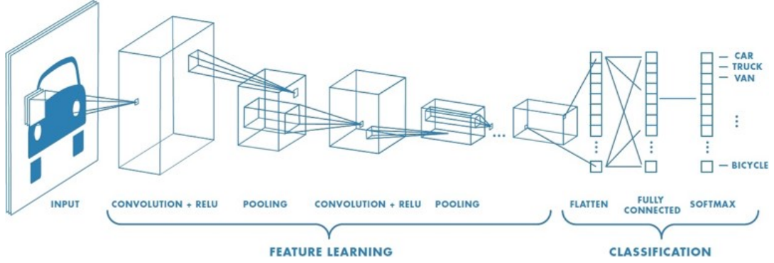
Figure 2.6: An example of a typical CNN. Convolutions are applied to images, and the output of each convolved image is used as the input to the next layer. Pooling layers are used to subsample the images. After obtaining the feature map, all the features are linked using an FC layer and softmax is applied to get the final results [Mathworks, 2021].
