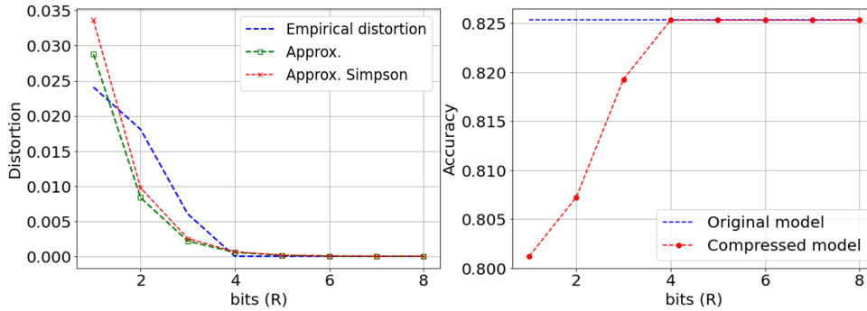
Figure 7.7: On the left, the rate distortion trade-off for one hidden linear layer. On the right, the accuracy for the original and compressed model.
