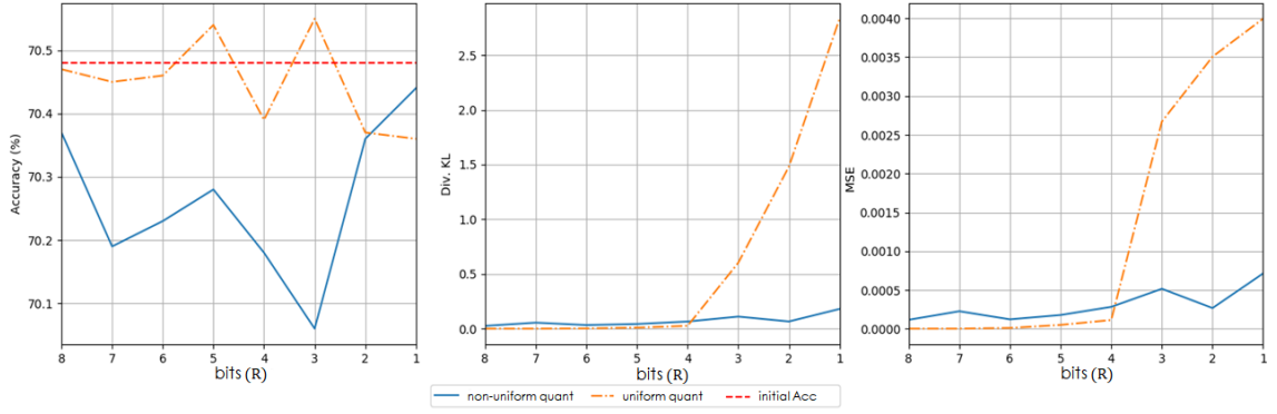
Figure 5.12: Accuracy, Div. KL and MSE for the last layer of VGG15
