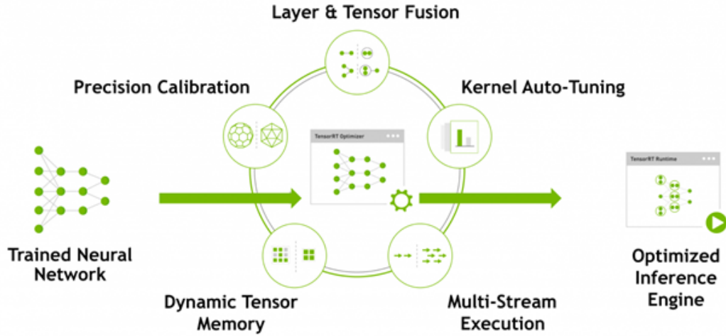
Figure A.1: Optimizations applied in TensorRT.
