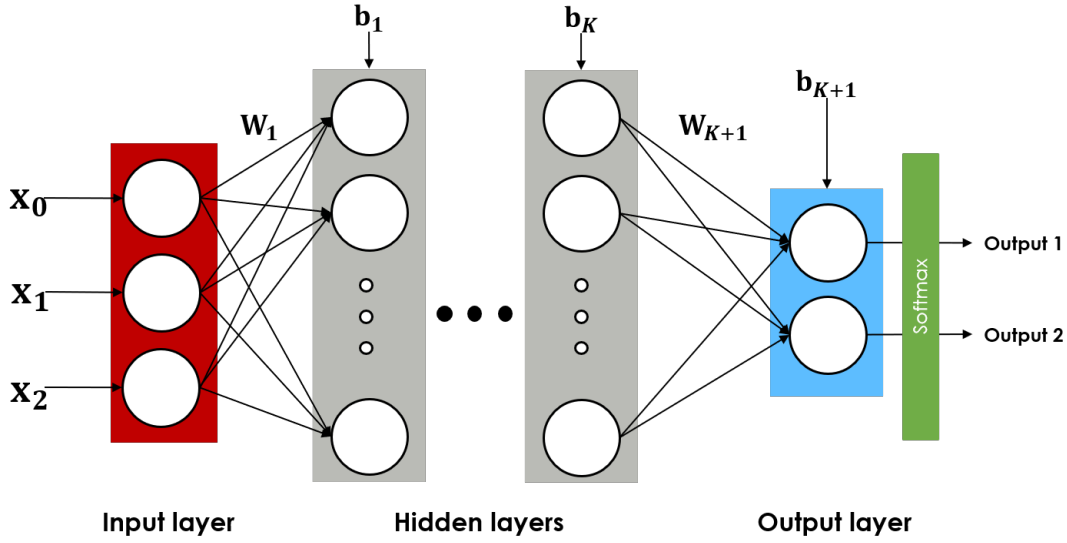
Figure 2.3: Architecture of a feedforward network with K hidden FC layers.
