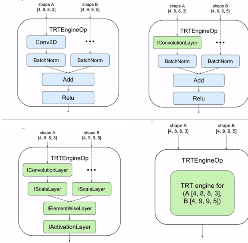
Figure A.3: Layer conversion and Engine built in TensorRT. The figure on the top left shows TensorFlow's subgraph before conversion to TensorRT layers. Phase 2 is done first. Second graph on the top right, TensorFlow operations are converted to TensorRT layer (indicated in green). The third graph (bottom left) shows the result after the conversion phase, where all TensorFlow operations are converted to TensorRT layers. Phase 3 creates a TensorRT engine from the graphs.
