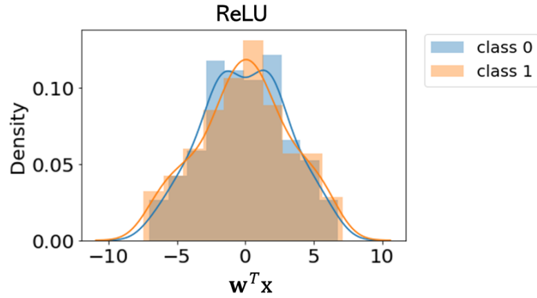
Figure 7.9: The distribution of w^T x for each class in the case of a hidden ReLU layer.
