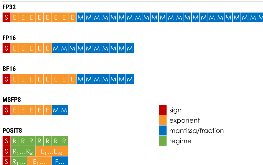
Figure 6.3: Visual comparison of formats. Standard formats FP32 and FP16 are shown on top. BF16 has the same size as FP16, but the same exponent size as FP32. MSFP8 has a 5-bit exponent size, the same as FP16, but only a 2-bit mantissa. Posits have variable sized fields. In this figure, we illustrate the composition of the Posit and the priority of each component: regime, exponent and the fraction (or mantissa).
