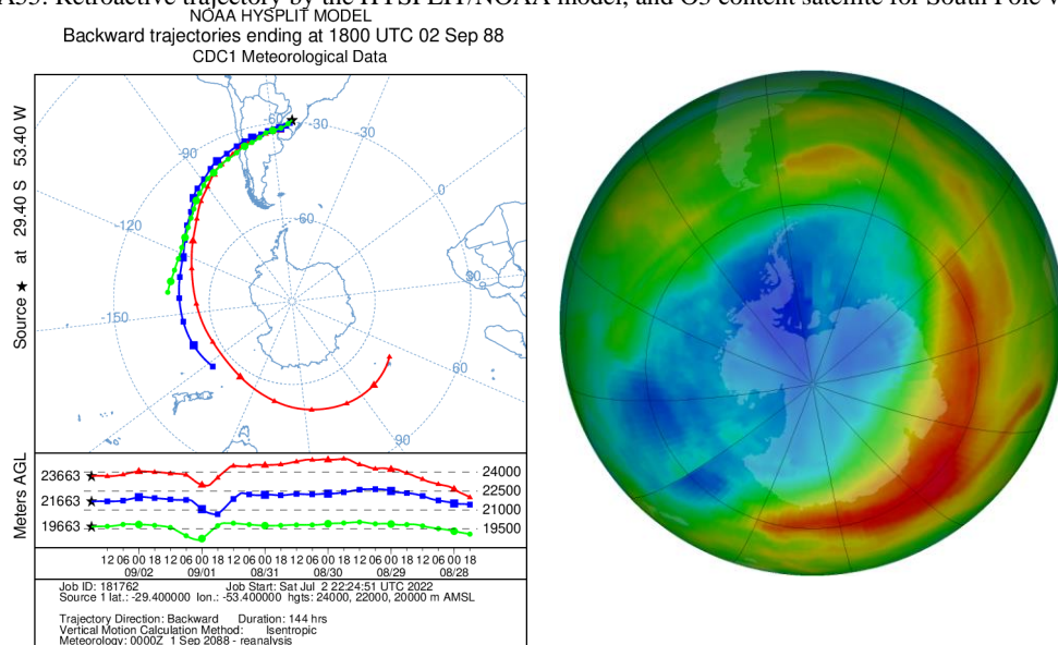
Figure A55: Retroactive trajectory by the HYSPLIT/NOAA model, and O3 content satellite for South Pole view.
