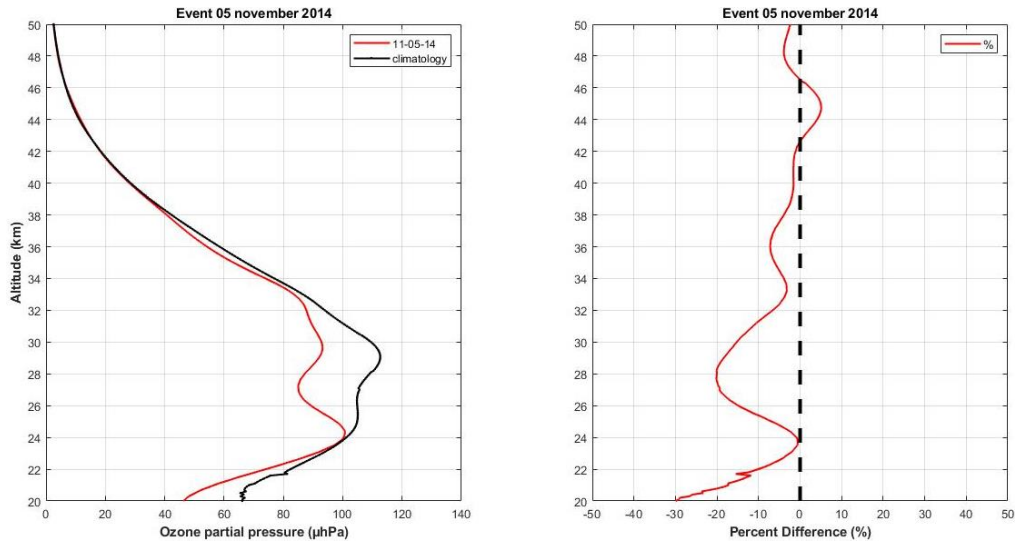
Figure A257: Vertical profile of O 3 by the SABER satellite for the November 05, 2014 (in red) and climatology for the month of October (in black).
