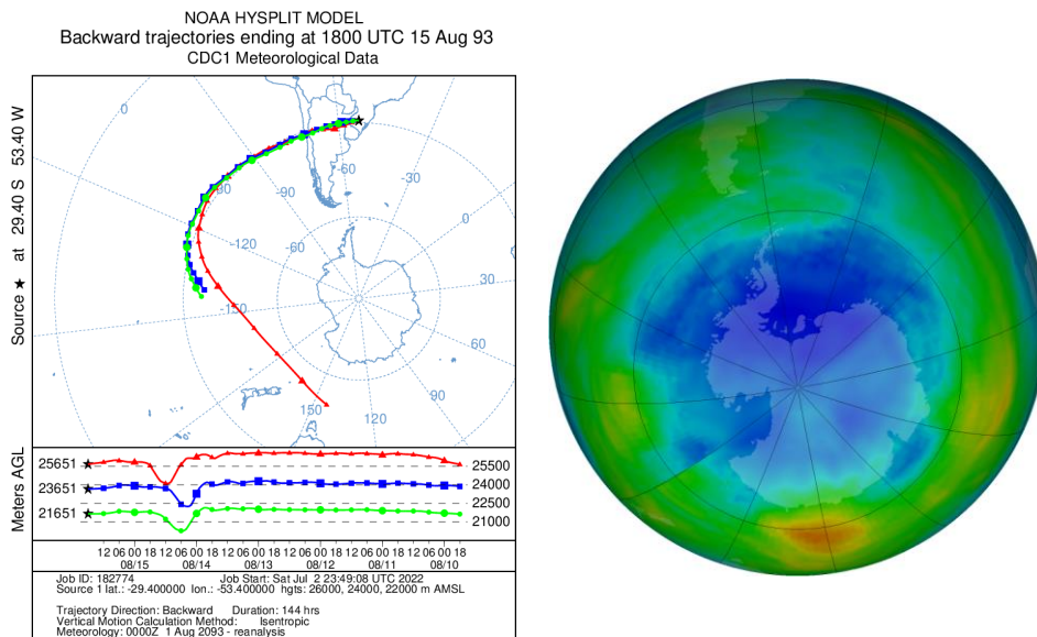
Figure A79: Retroactive trajectory by the HYSPLIT/NOAA model, and O3 content satellite for South Pole view.
