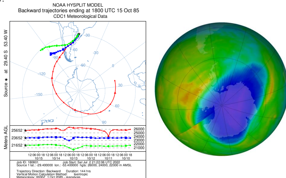
Figure A40: a) Retroactive trajectory by the HYSPLIT/NOAA model, b) O3 content OMI satellite for South Pole view.
