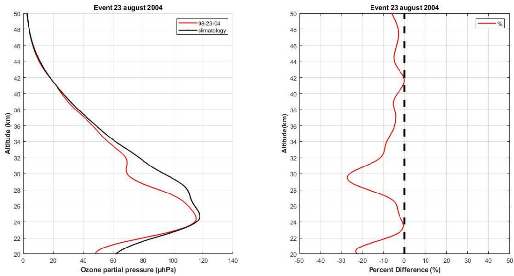
Figure A143: Vertical profile of O 3 by the SABER satellite for the August 23, 2004 (in red) and climatology for the month of October (in black).
