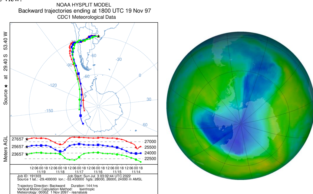
Figure A109: Retroactive trajectory by the HYSPLIT/NOAA model, and O3 content satellite for South Pole view.
