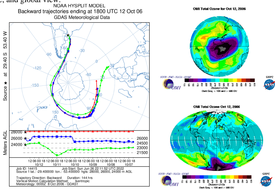
Figure A184: Retroactive trajectory by the HYSPLIT/NOAA model, and O3 content OMI satellite for South Pole, and global view.
