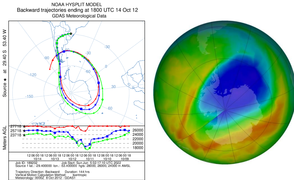
Figure A241: Retroactive trajectory by the HYSPLIT/NOAA model, and O3 content OMI satellite for South Pole, and global view.
