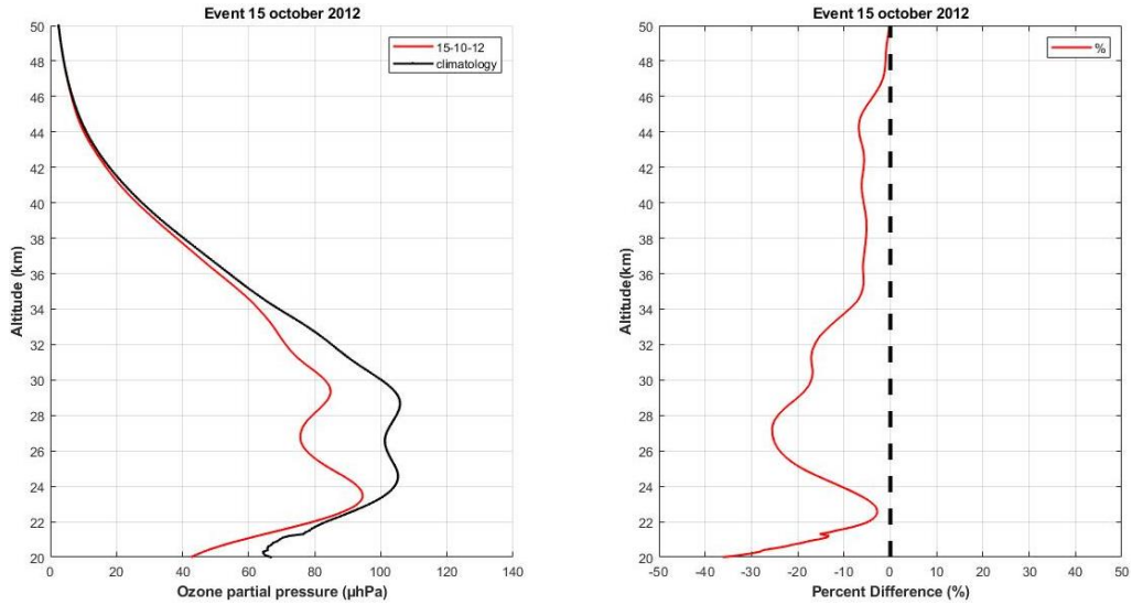
Figure A242: Vertical profile of O 3 by the SABER satellite for the October 15, 2012 (in red) and climatology for the month of October (in black).
