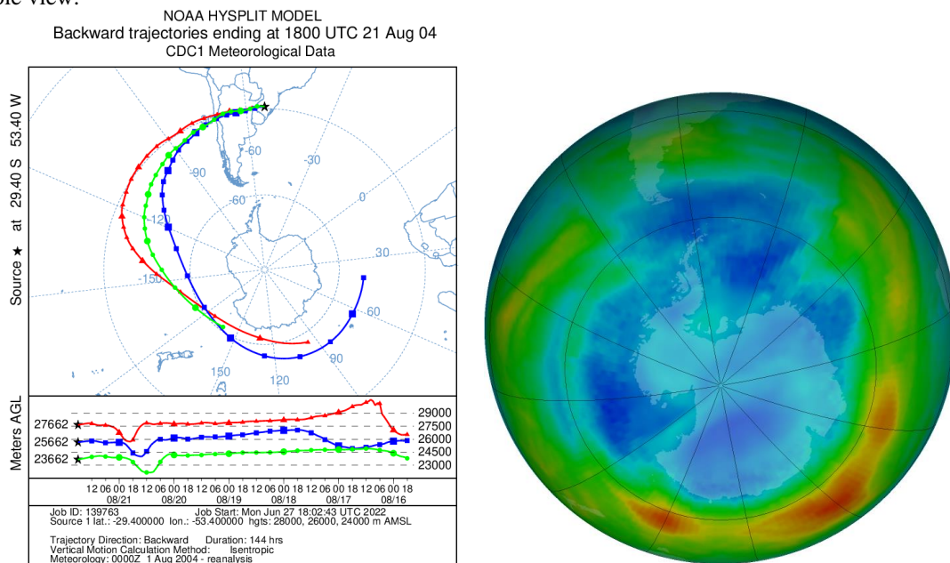
Figure A142: Retroactive trajectory by the HYSPLIT/NOAA model, and O3 content satellite for South Pole view.
