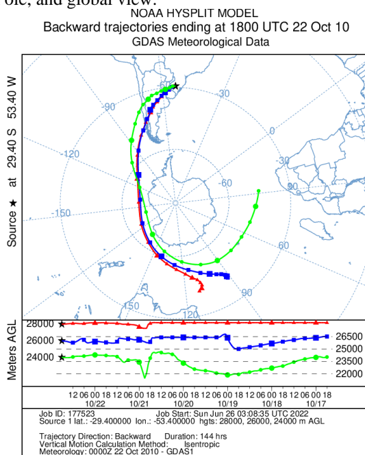
Figure A229: Retroactive trajectory by the HYSPLIT/NOAA model, and O3 content OMI satellite for South Pole, and global view.
