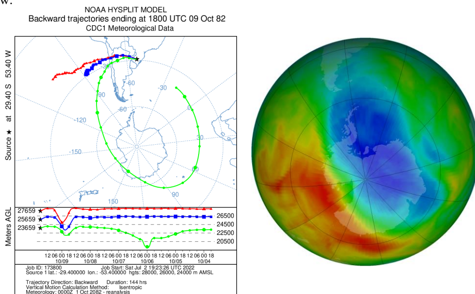
Figure A14: a) Retroactive trajectory by the HYSPLIT/NOAA model, b) O3 content OMI satellite for South Pole view.
