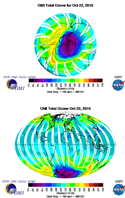
Figure A229: Retroactive trajectory by the HYSPLIT/NOAA model, and O3 content OMI satellite for South Pole, and global view.
