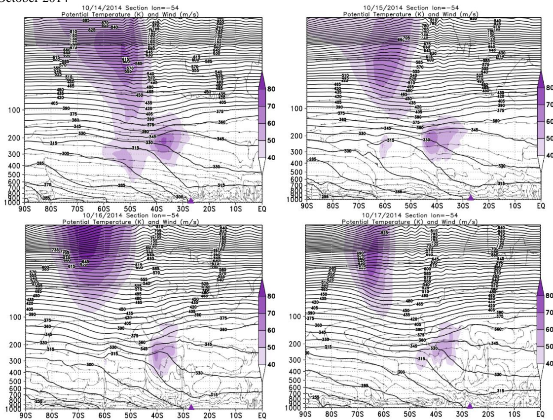
Figure A254: Vertical section of the atmosphere between 1000 and 5 hPa for the days of the event in October 2014
