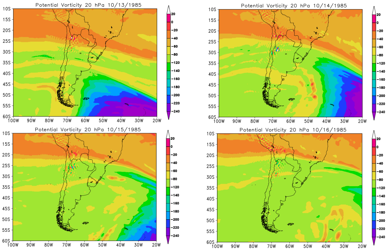
Figure A39: PVA fields for the 20 hPa in pressure levels, days 10/13/1985 to 10/16/1985.
