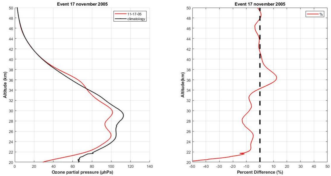
Figure A166: Vertical profile of O 3 by the SABER satellite for the November 17, 2005 (in red) and climatology for the month of October (in black).
