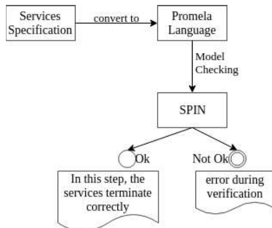
FIGURE 3.4: Processus de vérification
