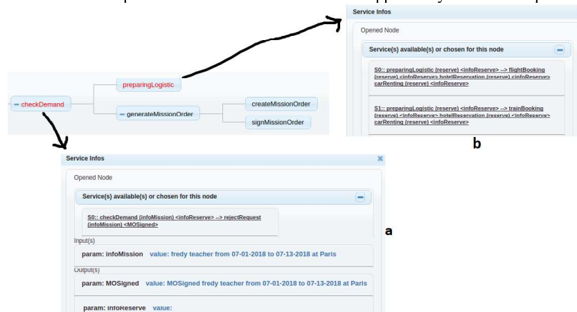
Figure 2. A runtime instance of the CheckDemand service
