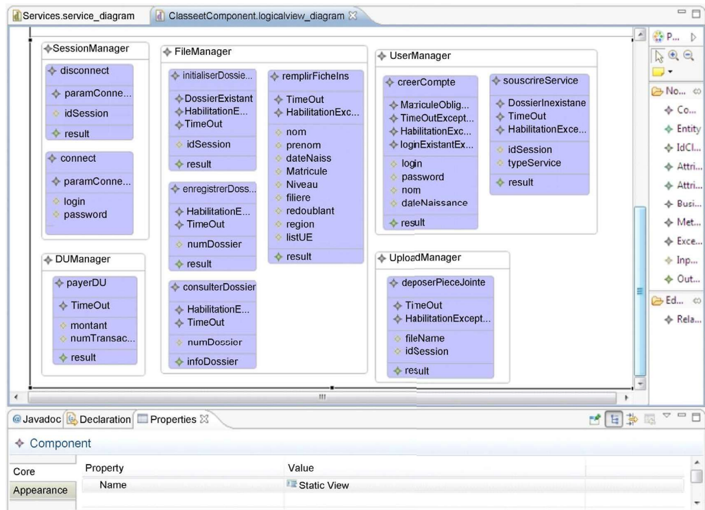
Figure A2. Business components represented by an Instance of the PIM.
