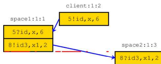
FIGURE 3.8: Services non correspondants
