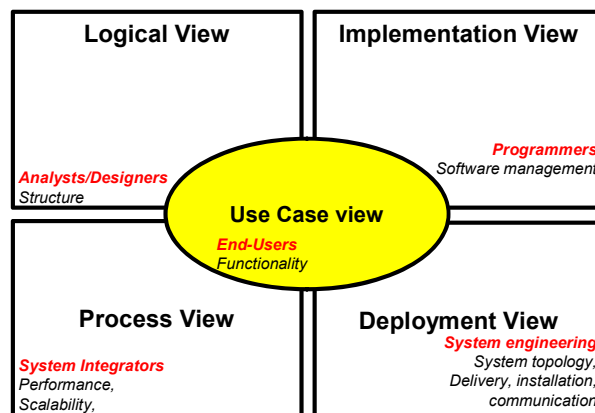
Figure 1. The 4 + 1 views model.
