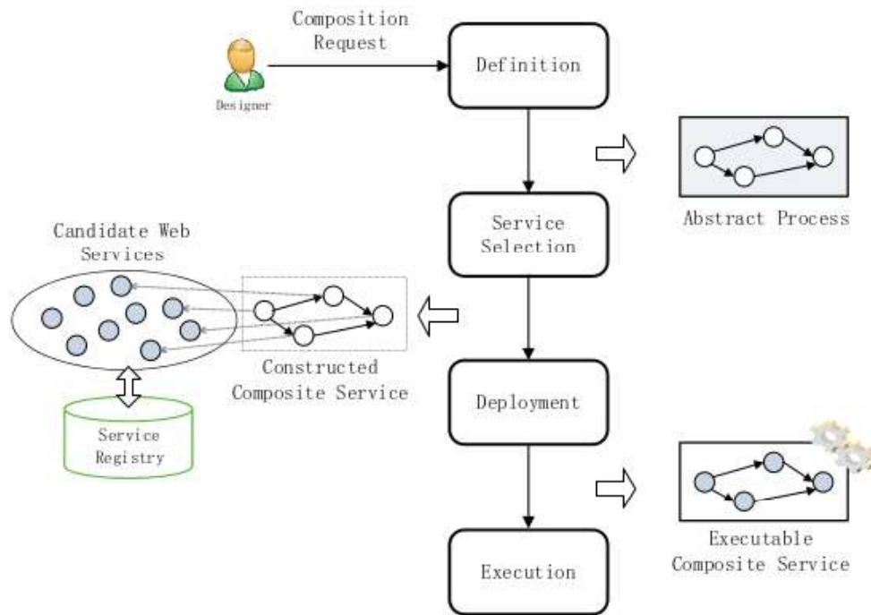
FIGURE 1.1: Processus de composition [2]
