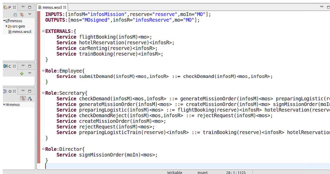
Figure 11. Modeling in the Editor : The variables, the external services and the defined services of each role are presented.
