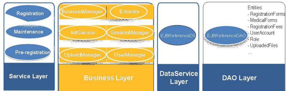
Figure 5. Architecture of the generated application.
