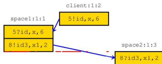
Figure 4. Not matching service: service parameters do not match. This implies the call of the client process does not execute until the end.
