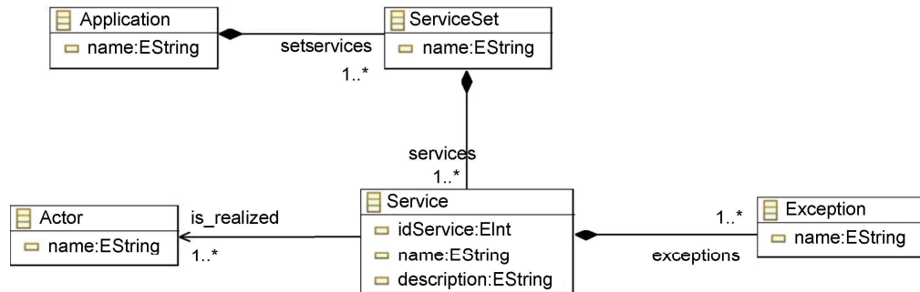
Figure 2. Service meta model.
