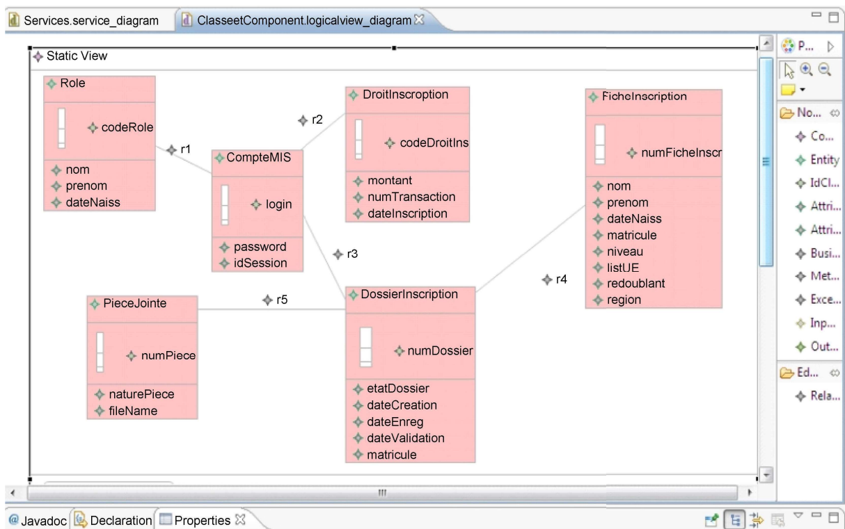
Figure A3. Data models from persistent classes.
