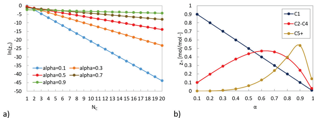
Figure 1.31: a) ASF distribution of compounds C 1 -C 20 : logarithm of the mole fraction of compounds with carbon number n as function of carbon number; b) Mole percentage of C 1 , C 2 -C 4 and C 5+ hydrocarbons fraction as functions of \alpha , estimated from the ideal ASF distribution.
