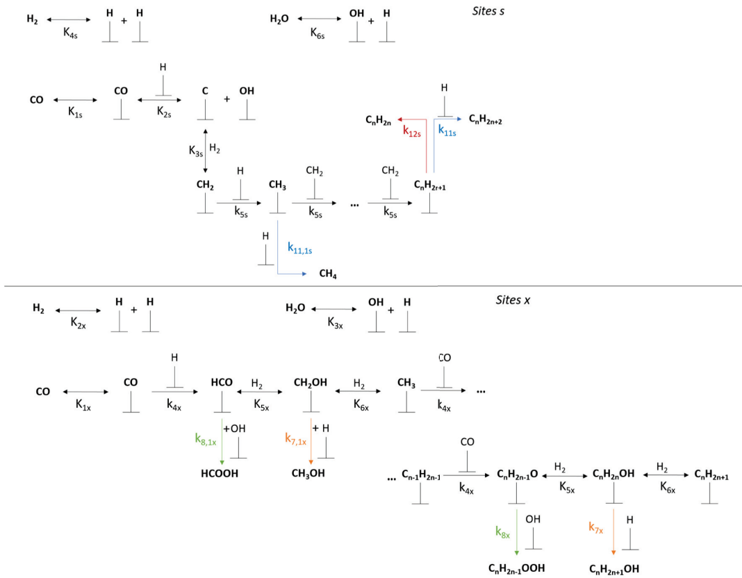
Figure 5.5: Reaction mechanism assumed for the formation of olefins, paraffins, alcohols and acids via FT when the presence of two types of active site is assumed (FT-B).
