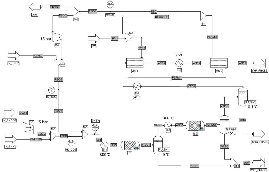
Figure 6.22: Schematic diagram of the process configuration with two reactors in series and separation of unreacted gases from light hydrocarbons via membrane filters.
