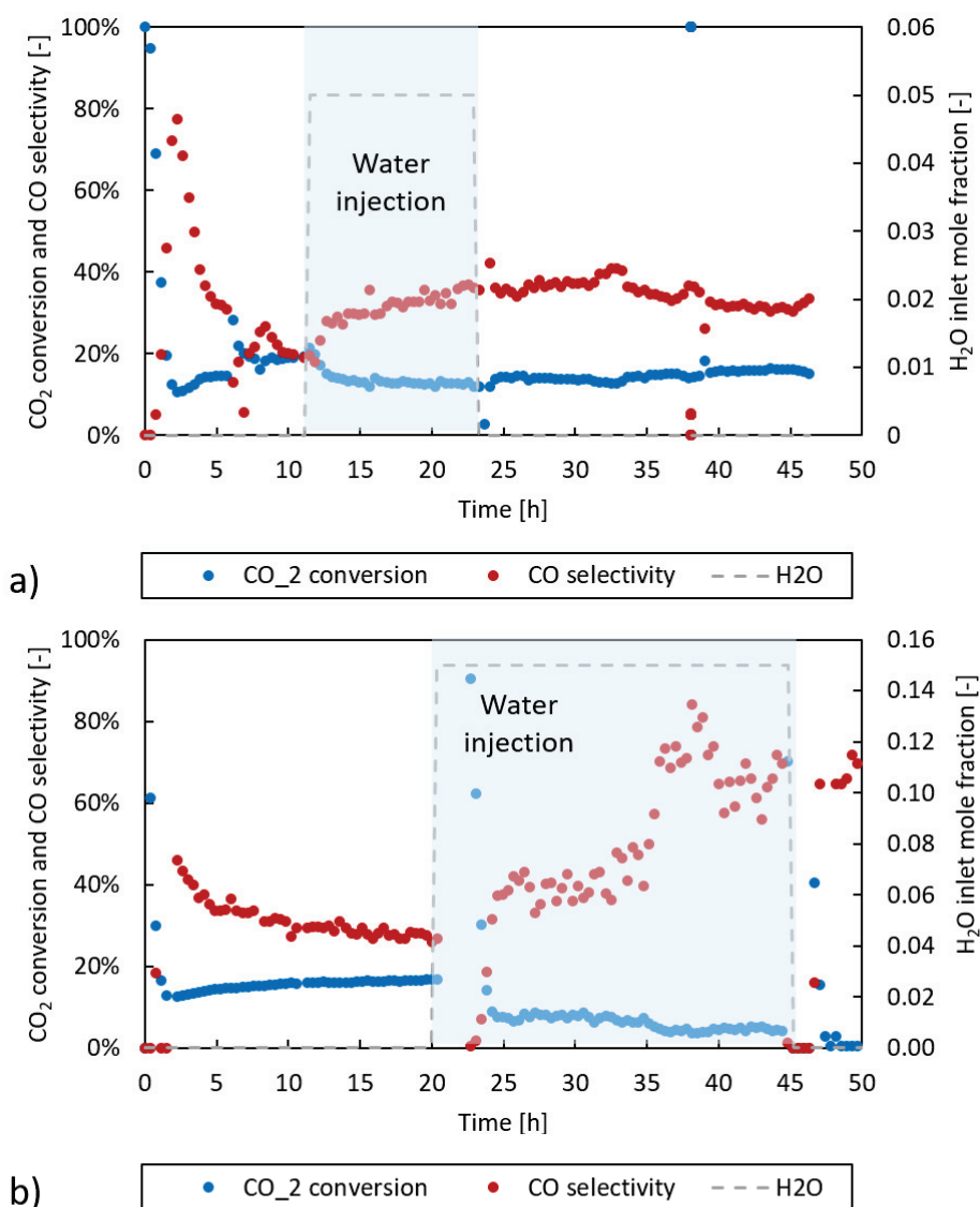
Figure 3.20: Effects of water co-feeding on CO 2 conversion and CO selectivity. a) molar fraction of water in the feed of 5%; b) molar fraction of water in the feed of 15%.
