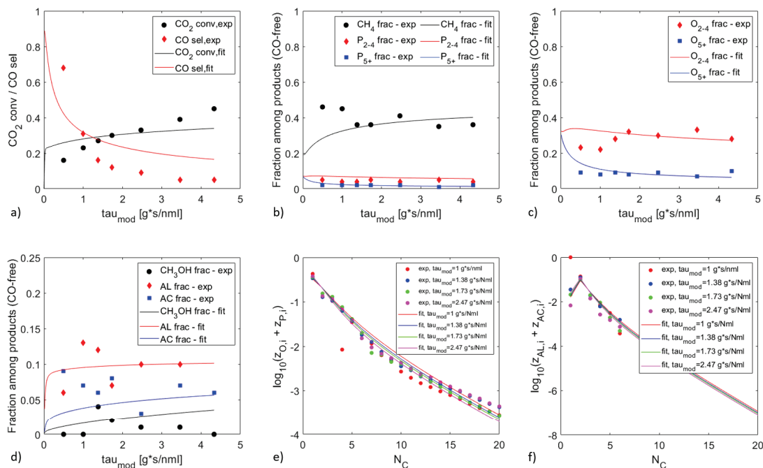
Figure 5.12: Results of the multi-site kinetic model as function of \tau_{mod} . Evolution of: a) \text{CO}_2 conversion and CO selectivity; b) fractions of \text{CH}_4 , \text{C}_2 - \text{C}_4 paraffins and \text{C}_{5+} paraffins; c) fractions of \text{C}_2 - \text{C}_4 olefins and \text{C}_{5+} olefins; d) fractions of methanol, \text{C}_2 - \text{C}_6 alcohols and \text{C}_2 - \text{C}_6 acids; e) ASF distribution for olefins and paraffins; f) ASF distribution for alcohols and acids. Model predictions are represented by solid lines, points represent experimental data.
