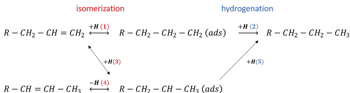
Figure 1.28: Description of the formation of secondary products. Adapted from Schulz et al. (2005).
