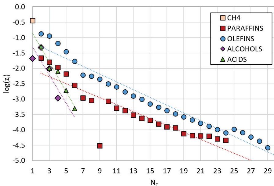
Figure 3.14: ASF distribution of C_1 - C_{30} olefins, paraffins, alcohols and acids for the reaction in reference conditions (2000 Nml/ g_{cat} /h, H_2/CO_2 ratio of 3, 15 bars and 300^\circ C ). z_i is the mole fraction of products with i carbon number among all hydrocarbons. Dashed lines represent the ideal ASF fit of the experimental points.
