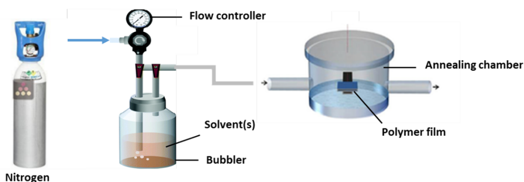
Figure 17. Solvent Vapor Annealing (SVA) setup. Adapted from [93,94].
