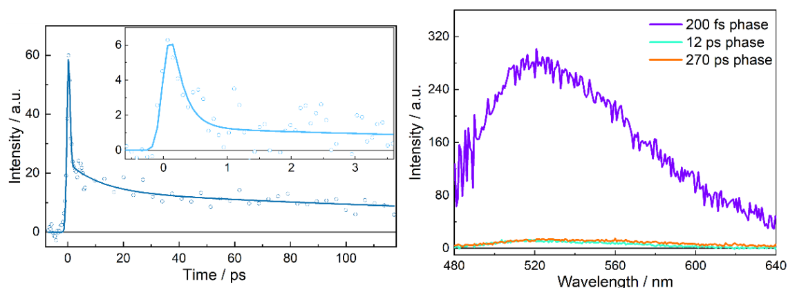
Figure 6.4 Fluorescence decays of uncomplexed \text{FAD}_{\text{ox}} in MSOX monitored at 520 nm with \text{CS}_2 or suprasil (inset) as Kerr medium (left), and the corresponding DAS from the global analysis (right).
