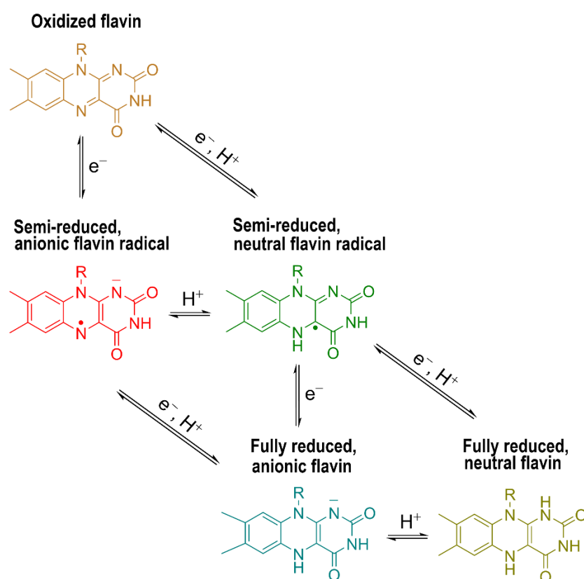
Scheme 1.2 Five redox and protonation states of flavins involved in the functional processes of flavoproteins. Flavin is represented by the isoalloxazine moiety.
