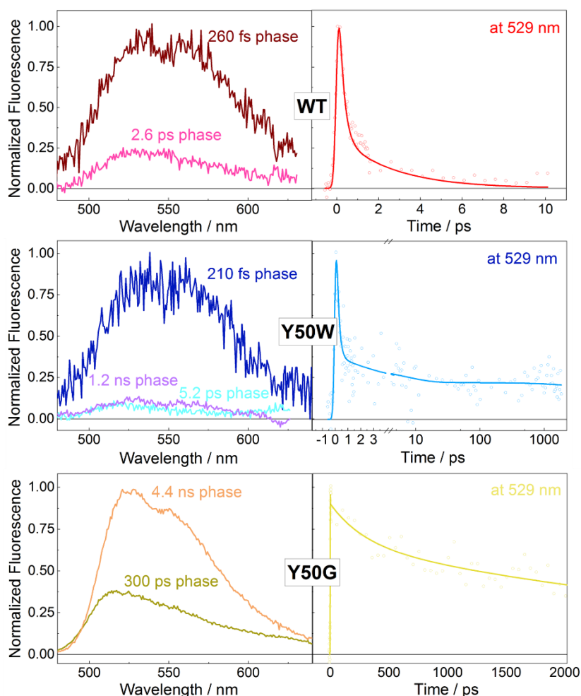
Figure 3.6 Decay associated spectra (DAS) from the global analysis of fluorescence decays ( left ) and kinetic traces at 529 nm ( right ) of WT, Y50W (on linear-logarithmic timescale) and Y50G BsfFNR .
