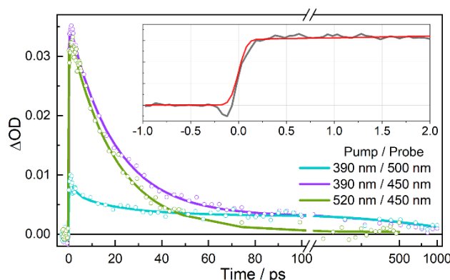
Figure 4.6 Isotropic transient absorption kinetics of \text{FAD}^{\bullet-} in GOX at selected wavelengths upon excitation at 390 nm or 520 nm. Inset panel: the rise of induced absorption signal (grey) at 433 nm (at the minimum of the probe dispersion curve) under 390 nm excitation. The red curve represents an instrument-response limited rise.
