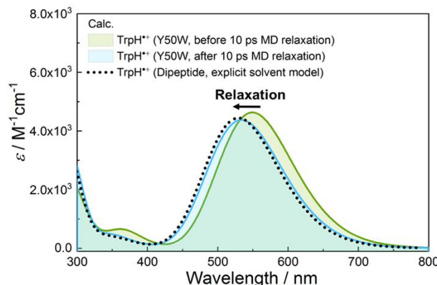
Figure 3.16 Calculated spectral charges of \text{TrpH}^{\bullet+} following the relaxation process after the initial ET (averaged over 50 snapshots). As a reference, the calculated \text{TrpH}^{\bullet+} absorption spectrum in solution (explicit solvent model, structures of dipeptide for spectral calculations were taken from MD simulations with radical cationic geometry; the calculated spectrum corresponds to the average over 100 snapshots) is shown as the dotted line.
