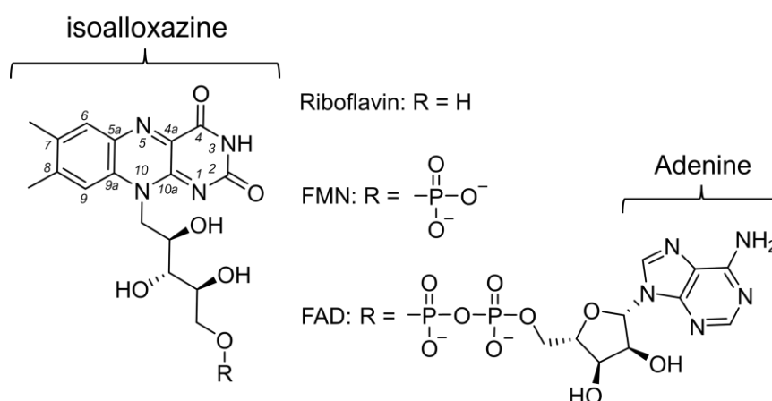
Scheme 1.1 Chemical structure of biologically important flavins.
