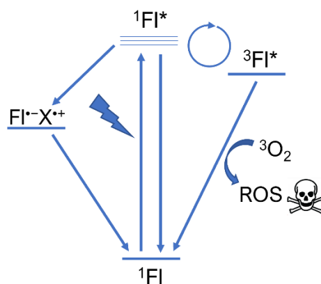
Scheme 1.3 Simplified scheme of photochemical reactions involving (singlet) oxidized flavins ( ^1\text{Fl} ).
