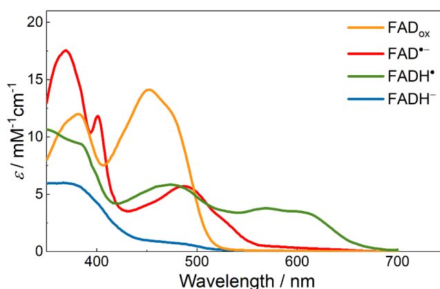
Figure 1.1 Steady-state absorption spectra of flavins in different redox and protonation states in GOX. The spectrum of \text{FADH}^\bullet is reproduced from ref. 5. The color coding corresponds to that in Scheme 1.2.
