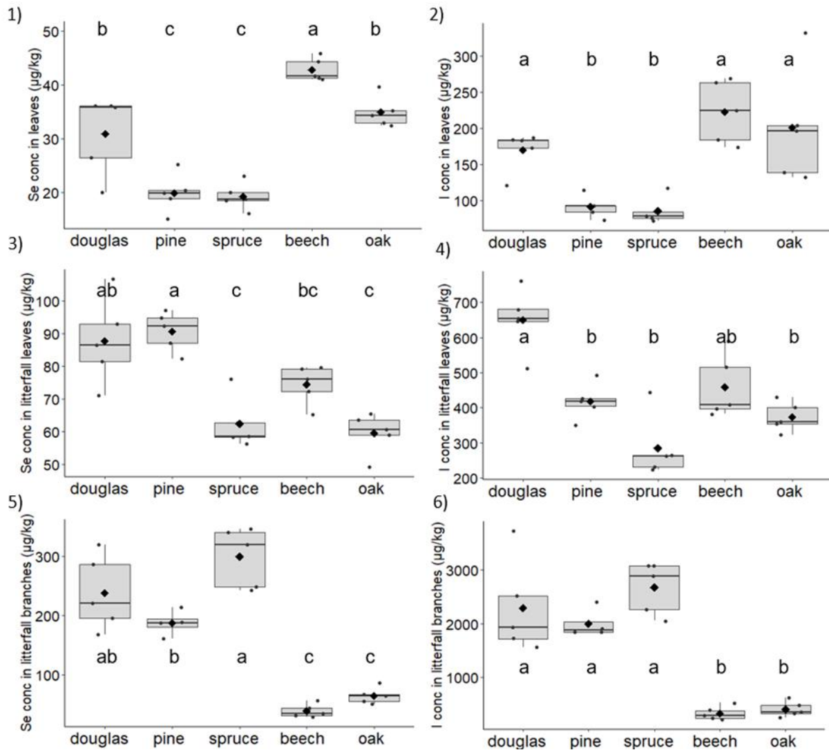
Figure art.2 – 1 Selenium and iodine concentrations (dots) in (1), (2) leaves; (3), (4) litterfall-leaves and (5), (6) litterfall-branches in forest stands (n = 5/stand). Box plots show the first quartile (Q 1 ), third quartile (Q 3 ) and median of the data. Black diamond symbols indicate average element concentrations in groups. Upper and lower whiskers extend from the hinges by Q_1 - 1.5 \times IQR ( IQR - interquartile range) and Q_3 + 1.5 \times IQR , respectively. Letters above the boxes correspond to significant differences between the groups according to Wilcoxon or Tukey tests.
