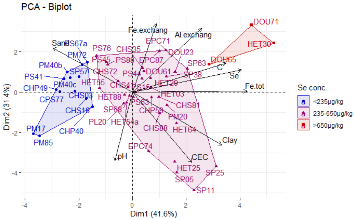
Figure art.1 – 6 PCA biplot representation of soil composition data on the first two PC axis. Individual soils (48 samples) are colored according to their Se concentration range: <235 µg kg -1 - blue, 235–650 µg kg -1 - violet, >650 µg kg -1 - red. Arrows represent contribution of soil geochemical numerical variables on principal component axes. (For interpretation of the references to color in this figure legend, the reader is referred to the web version of this article.)
