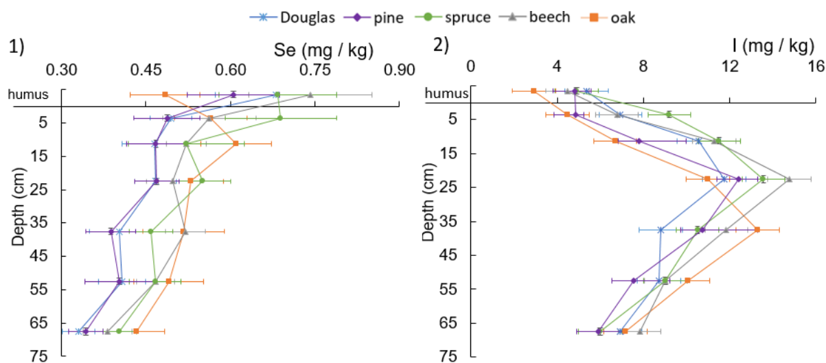
Figure art.2 – 3 Soil profiles of selenium (1) and iodine (2) in forest stands (mean value \pm standard deviation).
