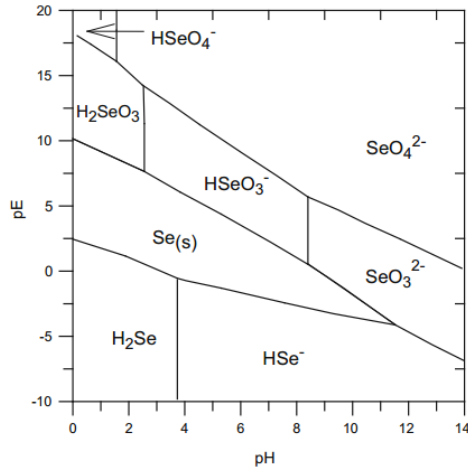
Figure chap.1 – 3 Selenium pE-pH diagram at 25°C, 1 bar pressure, and zero ionic strength for Se activity of 10^{-10} mol L -1 (Sharma et al., 2015).
