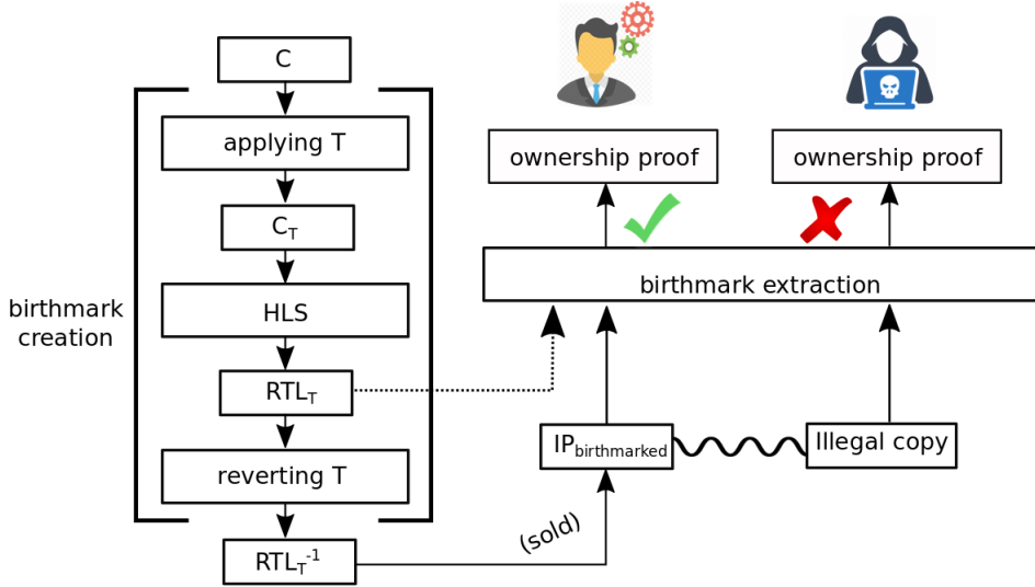
Figure 3.2 – Watermarking Flow.
