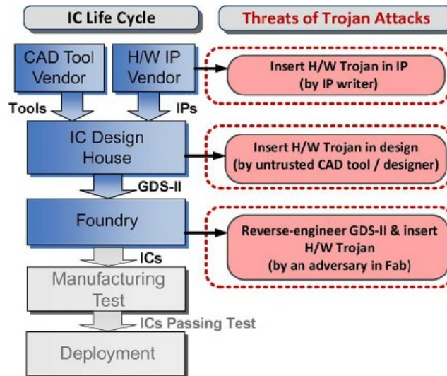
Figure 1.4 – HT attacks at different design stages. (from [Bhu+14])
