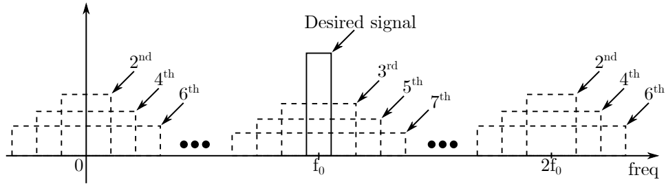
Figure 1.37 – Illustration of intermodulation modes showing 2 nd to 7 th order distortions
