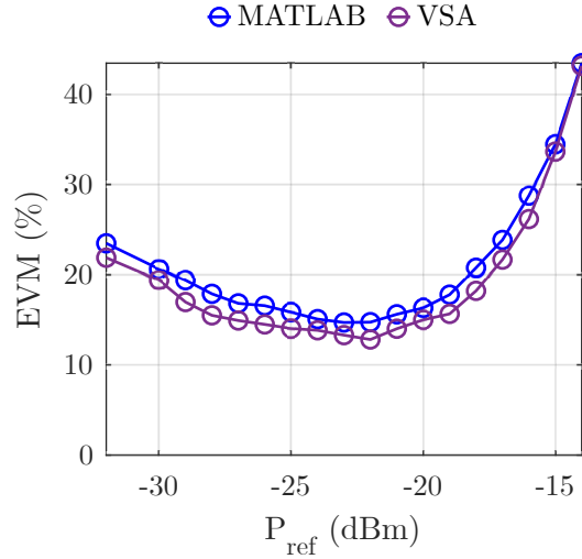
Figure 4.14 – Average EVM of the VSA and MATLAB receivers at different input powers into the SOA for five measurements of an 8 GHz OFDM frame. I_{\text{bias}} = 200 mA
