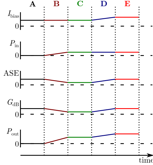
Figure 1.26 – Evolution of SOA operating point when I_{bias} and P_{in} vary. I_{bias} : bias current, P_{in}/P_{out} : signal input/output power, G_{dB} : gain, ASE: amplified spontaneous emission
