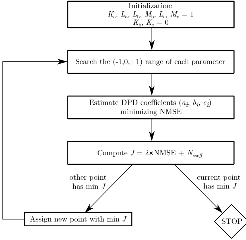
Figure 2.6 – Hill-Climbing algorithm
