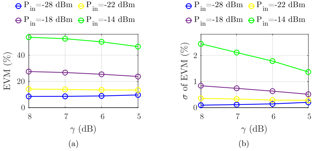
Figure 2.4 – (a) Average EVM and (b) standard deviation \sigma of the EVM taken from 10 different simulation runs vs. clipping ratio \gamma at different input powers into the SOA
