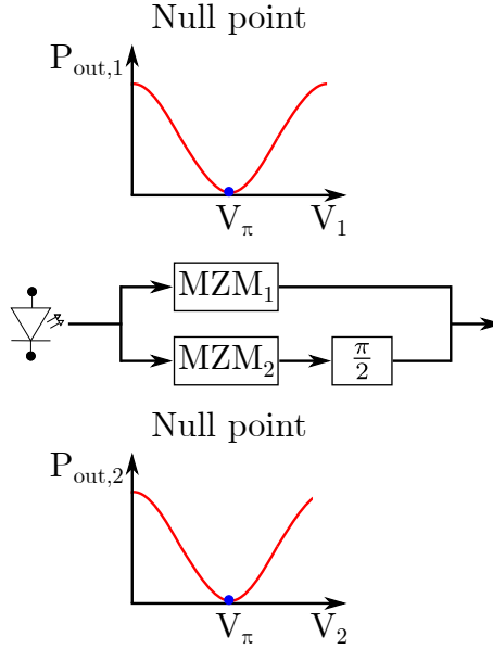
Figure 4.5 – Setting of the IQ modulator operating point. The two MZMs are operated at null point so that the IQ modulator can operate at the point where the optical field is most linear
