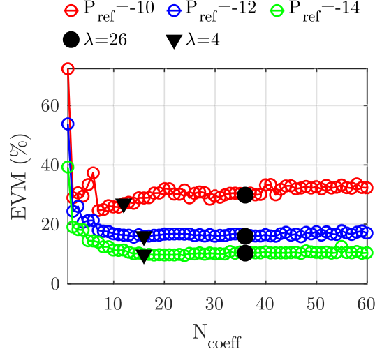
Figure 2.9 – GMP at the validation phase for different P_{\text{ref}} . Best EVM is the minimum EVM for each P_{\text{ref}} , and \lambda = 4 and \lambda = 26 are the EVM obtained using predistorters found with Hill-Climbing
