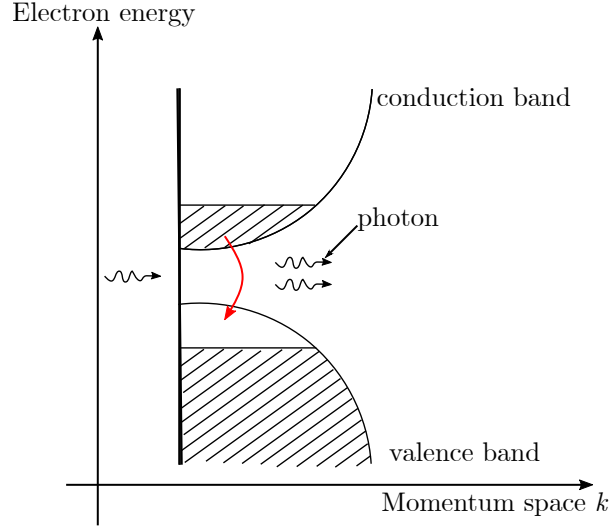
Figure 1.25 – Amplification in the SOA through stimulated emission
