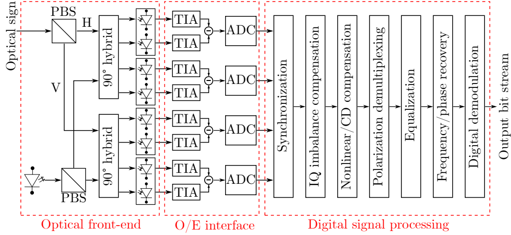
Figure 1.32 – Outline of an optical digital coherent receiver. PBS: polarization beam splitter, H: horizontal polarization, V: vertical polarization, TIA: transimpedance amplifiers, ADC: analog to digital conversion, CD: chromatic dispersion, O/E: optical/electrical
