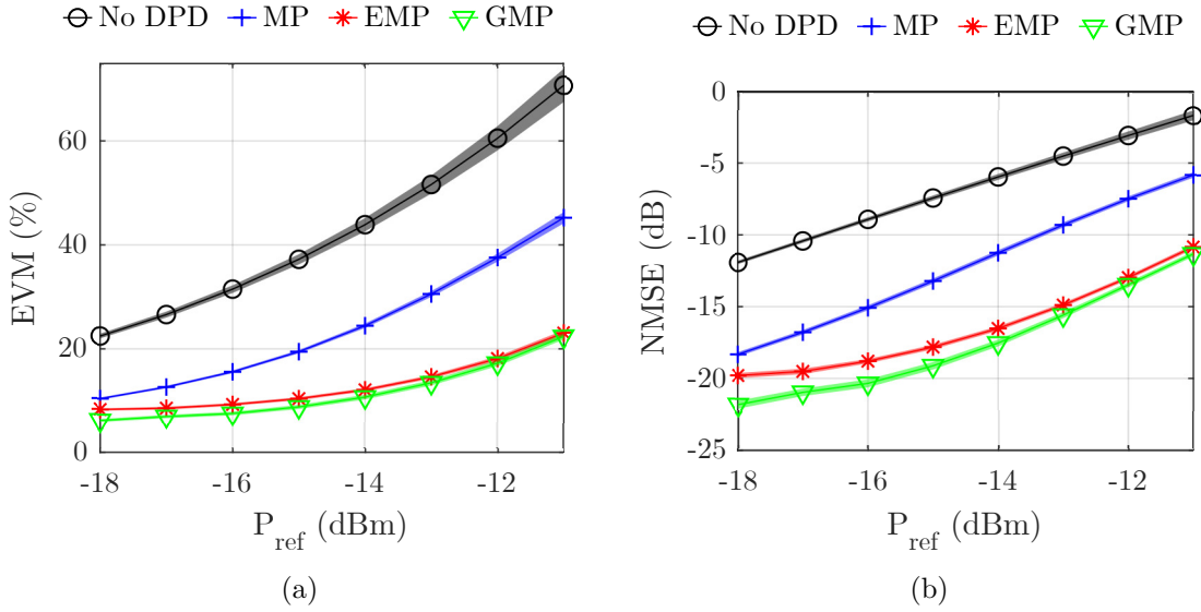
Figure 2.12 – (a) EVM and (b) NMSE for different predistorters at different P_{ref}
