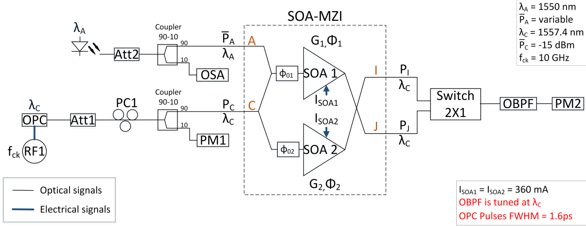
Figure 4.4: Experimental setup for the quasi-static characterization with pulses of Modulation architecture. Reproduced from [1] (© 2020 IEEE).
