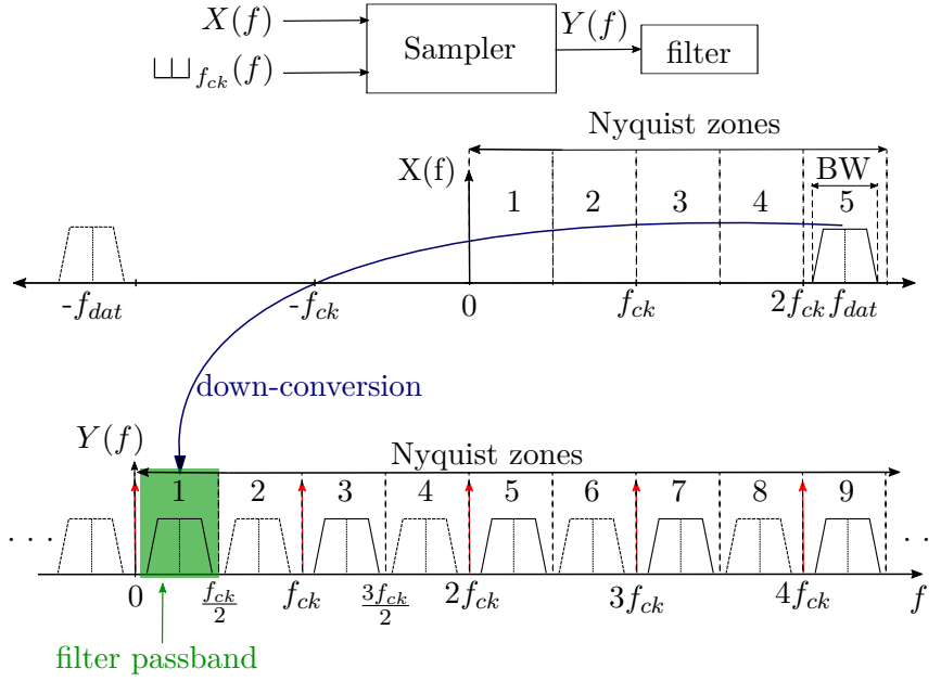
Figure 2.7: Conceptual diagram of band-pass sampling for the purpose of down-conversion. The original band-pass signal spectrum is X(f) . The sampled signal spectrum is Y(f) . BW is the bandwidth of the band-pass signal. The filter lets only the first Nyquist zone of Y(f) to pass, whereas it discards the higher order Nyquist zones.
