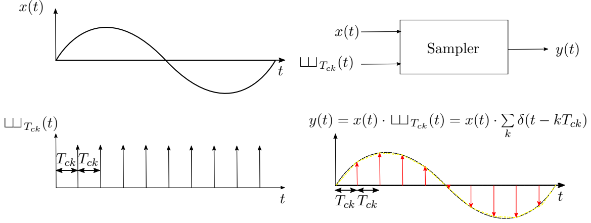
Figure 2.1: Sampling of sinusoidal signal x(t) . The sampling process mathematically consists of multiplying analog x(t) by Dirac comb, \sqcup\sqcup_{T_{ck}}(t) . The envelope of the sampled signal y(t) , denoted by the dashed black line, is the original signal x(t) .
