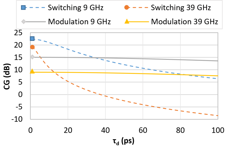
Figure 4.18: Comparison between theoretically calculated CG values of the Switching and Modulation frequency up-conversion at 9 GHz and 39 GHz as a function of \tau_d .
