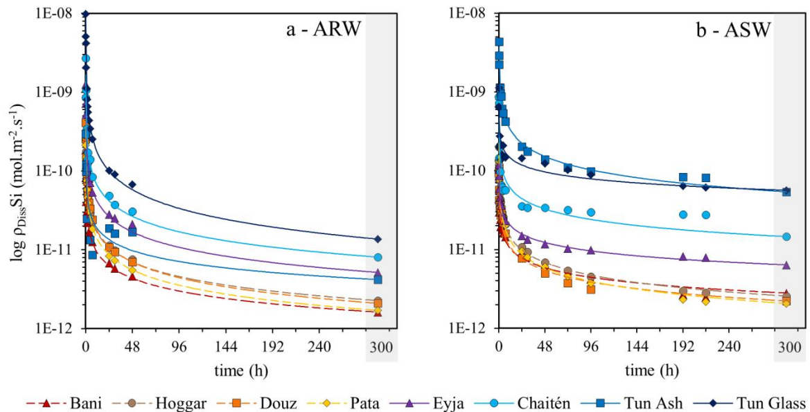
Figure II-7: Silicon dissolution rate ( \text{mol dSi.m}^{-2}.\text{s}^{-1} ) of aerosols in artificial (a) rain (ARW) and (b) seawater (ASW) in log scale. The data points at t_{300} h (shaded) are calculated from a power fit extrapolation of the steady state.
