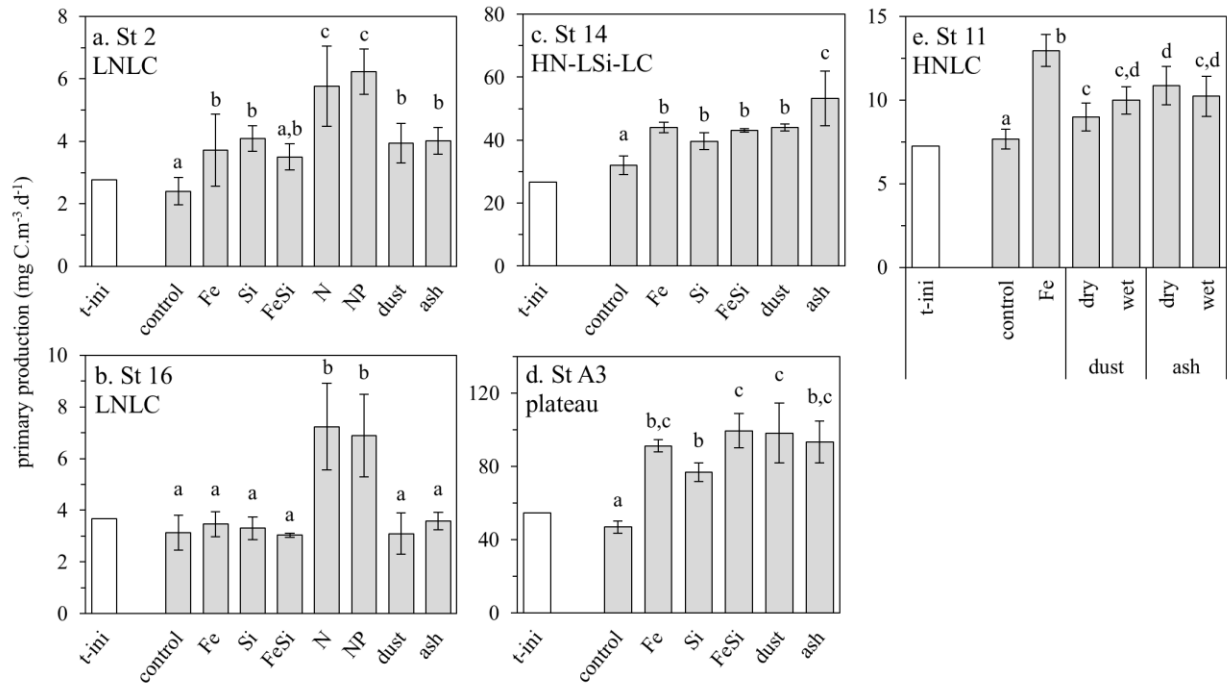
Figure V-2. Primary production (PP, \text{mg C}\cdot\text{m}^{-3}\cdot\text{d}^{-1} ) at the beginning of the experiment (t-ini, white bars) and after 48 h of incubation for each treatment at the stations LNLc St 2 (a) and 16 (b), HN-LSi-LC St 14 (c), plateau St A3 (d) and HNLC St 11 (e). Error bars indicate standard deviation of triplicates. Means that are not significantly different ( p > 0.05 ) are labeled with the same letter within a station.
