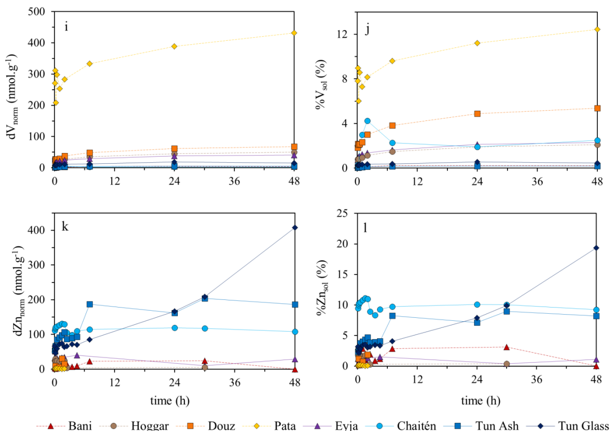
Figure IV-3: Dissolution (in \text{nmol.g}^{-1} , left panels) and solubility ( \% , right panels) of additional micronutrients in artificial rainwater: dCd (a,b), dCu (c,d), dMo (e,f), dNi (g,h), dV (i,j) and dZn (k,l). Warm colors and dashed lines represent desert dust, cold colors and plain lines represent volcano ash.
