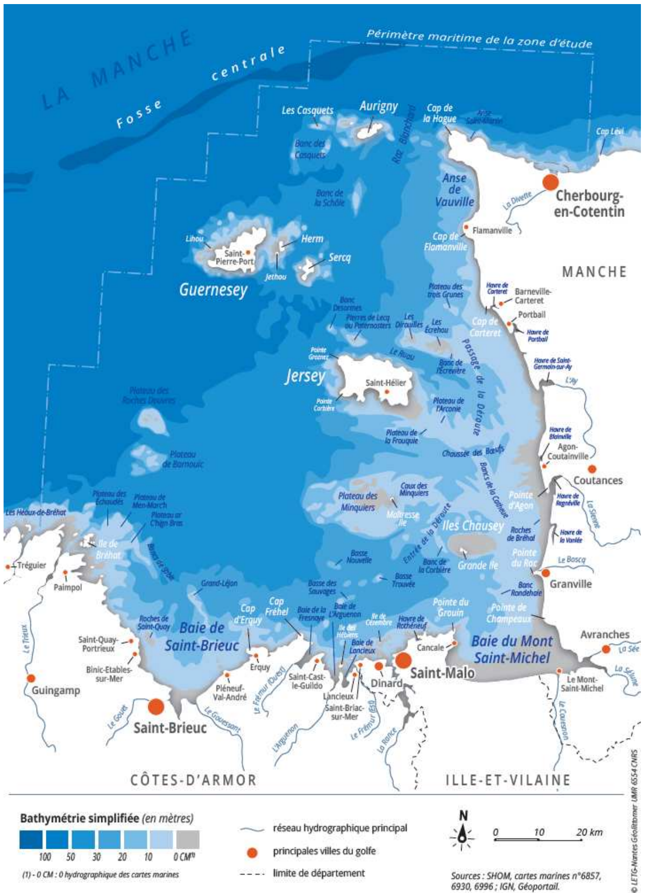
Figure 19: Bathymetry and toponymie of the English Channel, from Le Mao et al. (2019). ©LETG-Nantes Géolittomer UMR 6554 CNRS. https://archimer.ifremer.fr/doc/00612/72370/71329.pdf
