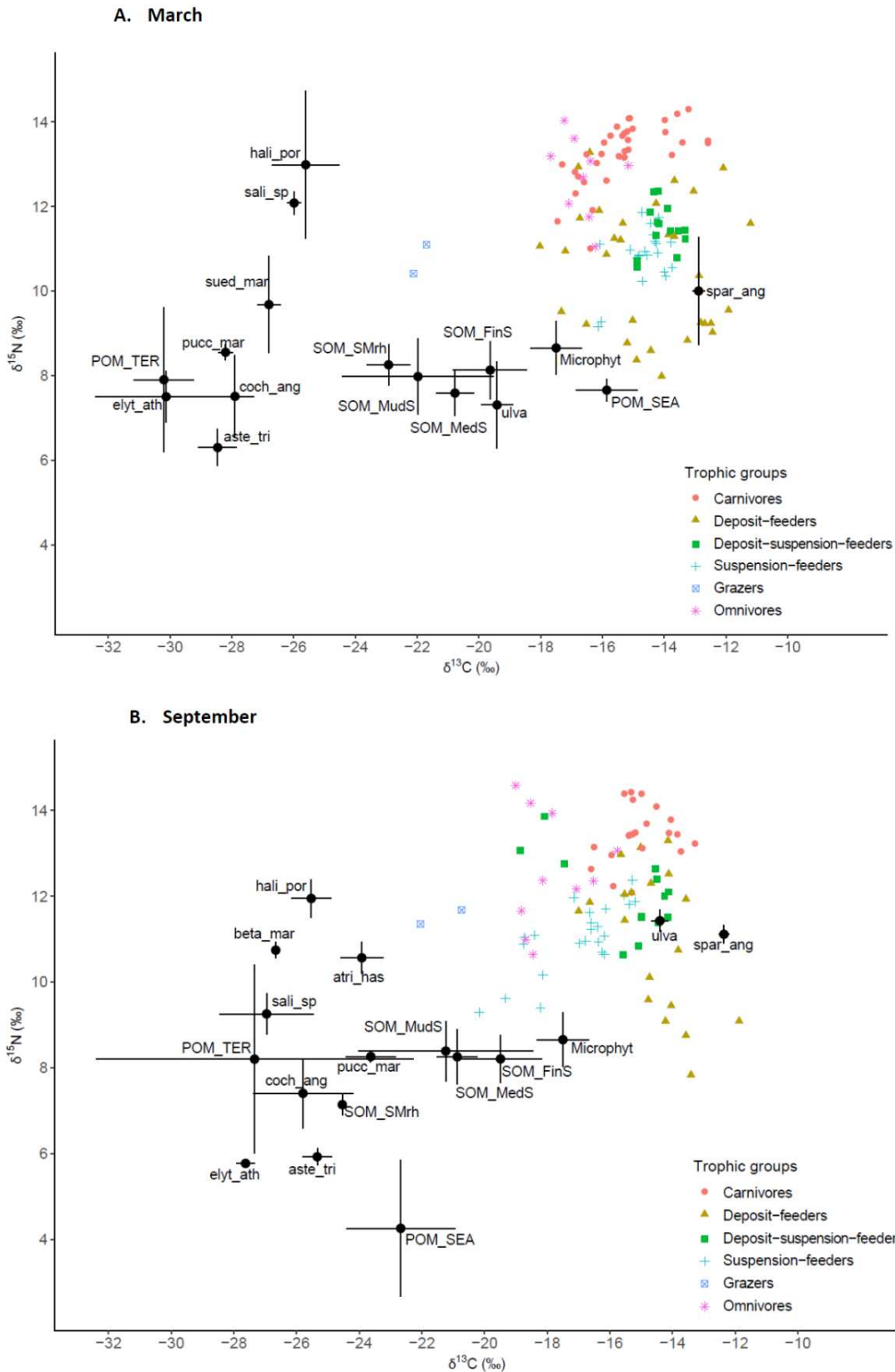
Figure 39: \delta^{13}\text{C} and \delta^{15}\text{N} of consumers and potential dietary sources in March (A) and September (B) in intertidal soft-bottom sediments of the bay of Saint-Brieuc. \delta^{13}\text{C} and \delta^{15}\text{N} values are plotted for each individual of consumers. Colors and shapes represent trophic groups. Mean \delta^{13}\text{C} and \delta^{15}\text{N} values of potential dietary sources are represented with black dots with error bars. Marine and terrestrial particulate organic matter (POM_SEA, POM_TER). Sedimentary organic matter in the different habitat from salt marsh to muddy, fine and medium sands (SOM_SMrh, SOM_MudS, SOM_FinS, SOM_MedS). Microphytobenthos (Microphyt). C3 plants: Halimione protulacoides (hali_por), Beta maritima (beta_mar), Atriplex hastata (atri_has), Salicornia sp (sali_sp), Puccinellia maritima (pucc_mar), Cochlearia anglica (coch_ang), Elytrigia atherica (Elyt_ath), Aster Tripolium (aste_tri). C4 plant: Spartina anglica (spar_ang). Algae: Ulva sp (ulva).
