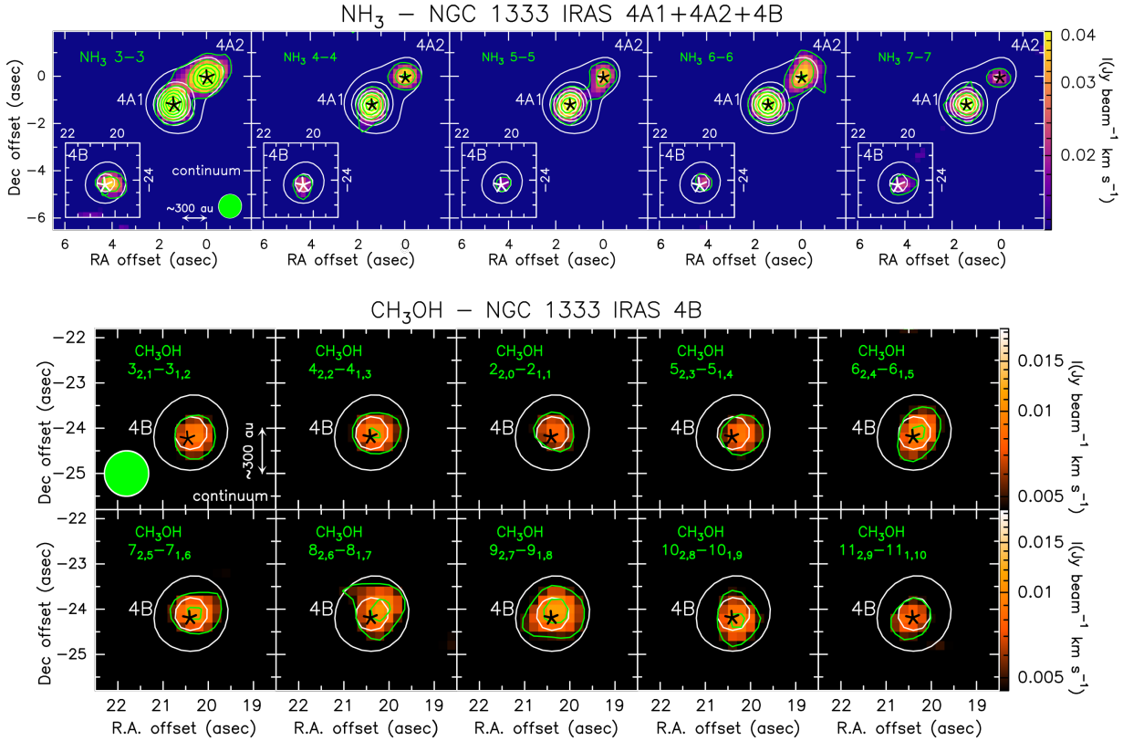
Figure 1. Top panels: \text{NH}_3 velocity-integrated maps toward IRAS 4A1, 4A2, and 4B in color scale, overlapped with the continuum white contours (from 50\sigma with steps of 100\sigma ). The emission is integrated from -30 to -11 \text{km s}^{-1} , -3 to +15 \text{km s}^{-1} , and +25 to +43 \text{km s}^{-1} , in order to include the main and the satellite hyperfine components. \text{NH}_3 first contour and steps (in green) correspond to 3\sigma ( \sigma=4.4 \text{mJy beam}^{-1} ). Bottom panels: \text{CH}_3\text{OH} velocity-integrated maps toward IRAS 4B in color scale overlapped with the continuum white contours (from 50\sigma with steps of 100\sigma ). The emission is integrated from -2 to +2 \text{km s}^{-1} with respect to the v_{\text{sys}} ( \sim +6.7 \text{km s}^{-1} Choi 2001). Methanol first contour and steps (in green) correspond to 3\sigma ( \sigma=1.6 \text{mJy beam}^{-1} \text{ km s}^{-1} ). The \text{CH}_3\text{OH} maps for IRAS 4A1 and IRAS 4A2 are reported in De Simone et al. (2020). The transition of the imaged line is reported in each panel. The black stars show protostars positions. Synthesised beams for continuum (white) and lines (green) are in the lower left corner.
