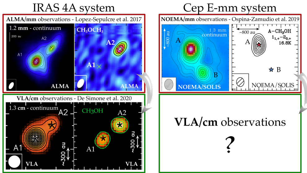
Figure 4.7: IRAS 4A binary system vs Cep-E binary system. Left: IRAS 4A system observed at mm wavelengths (red upper box) showing that the line emission comes from the source weaker in mm continuum emission, and at cm wavelengths (lower green box) showing that the line emission is actually coming from both sources: the dust was obscuring the hot corino in IRAS 4A1. Right: CepE-mm binary system at mm wavelengths (red upper box) showing that the line contribution is from the sources brighter in mm continuum emission. What will CepE look like at cm wavelengths?
