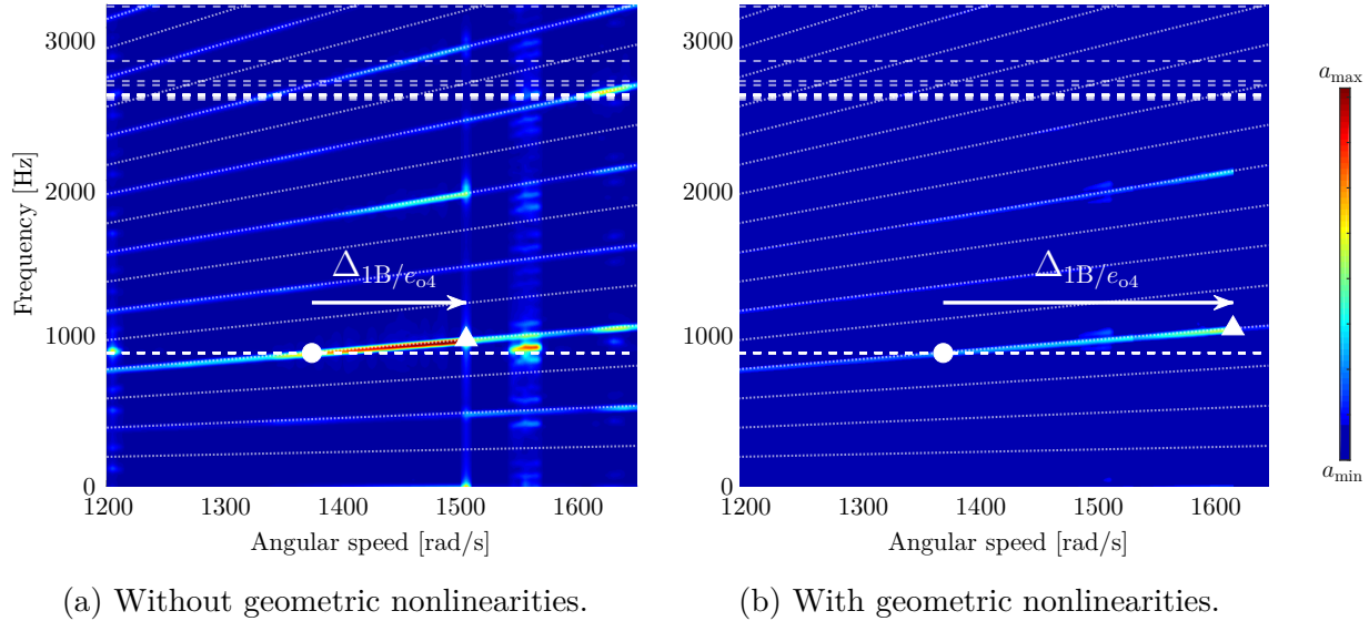
FIGURE 7.9 – Interaction maps of the radial displacement at node LE for the case with direct contact with eigenfrequencies (---), engine order lines (.....), predicted linear resonance ( \bullet ) and predicted nonlinear resonance ( \blacktriangle ).
