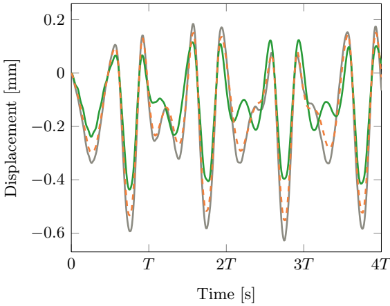
(a) With 10 randomly chosen MD (—), the 10 MD selected with criterion 1 (---).
