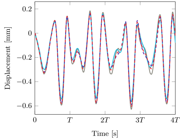
(b) With the 10 MD selected with criterion 2a (---), criterion 2b (---) and criterion 3 (—).
