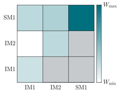
(c) Selection criterion 2b.
