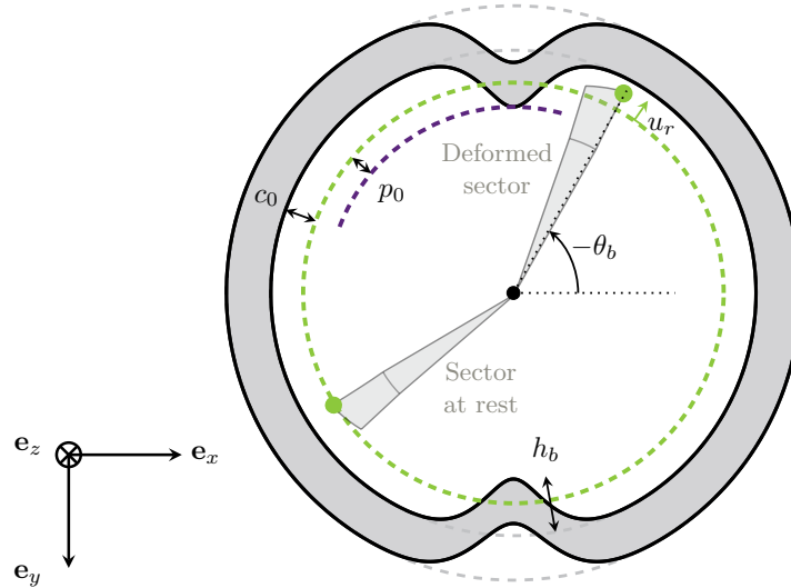
FIGURE 6.4 – Ovalization of the casing from (□) to (□), penetration of the casing profile (---) with respect to the circular trajectory (---) of a blade-tip node (●) of the sector at rest and definition of the parameters in Eq. (6.2) for the gap computation (not to scale).
