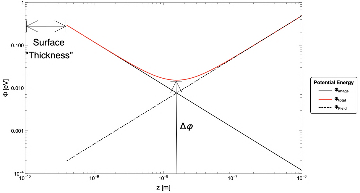
Figure 2.29 – The potential energy due to the electrostatic image of the charge (black solid line) and the potential energy due to the extraction field (black dashed line). Also is show the total energy (red solid line) as a function of the distance from the phase boundary. The extraction field cause a reduction of the potential barrier and the thickness of the surface is effectively defined by the order of magnitude of the interatomic distance.
