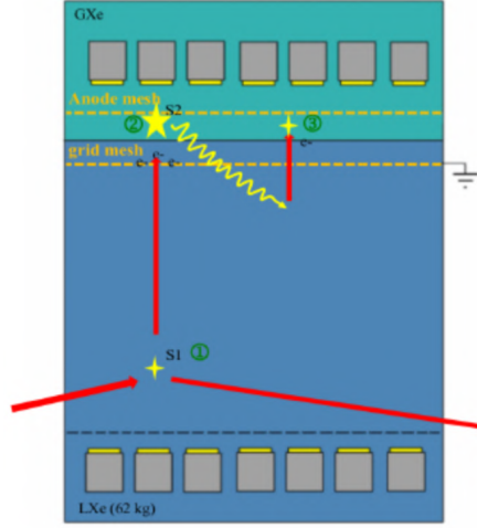
Figure 2.1 – Schematic representation of the main mechanism of production of the single electron background.
