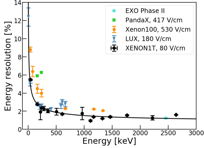
Figure 3.8 – The width of the peaks from energy deposits by various monoenergetic lines can be used in order to derive the energy resolution of the detector as a function of the deposited energy. Here the black points for XENON1T correspond to the isotopes listed in the text, while also shown are the energy resolutions for EXO Phase II, PandaX, XENON100 and LUX with the corresponding drift fields stated.
