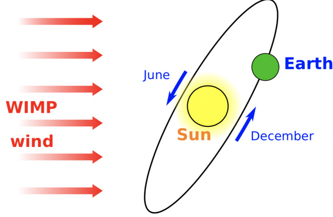
Figure 3.1 – Simplified depiction of the relative motion of the Earth in the galactic halo. Figure from [199].
