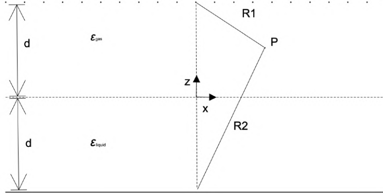
Figure 2.26 – Illustration of the 2D geometry of the electrostatic problem. Here the reference system is centered at the phase boundary surface, the x axis lies on the surface and the z axis is normal to the surface. LXe and GXe are dielectrics with dielectric constants \epsilon_l and \epsilon_g . The field is calculated at a point P(x, z) inside the space between the gate and the anode, solving the Poisson equation with the appropriate boundary conditions at the surfaces of the two electrodes.
