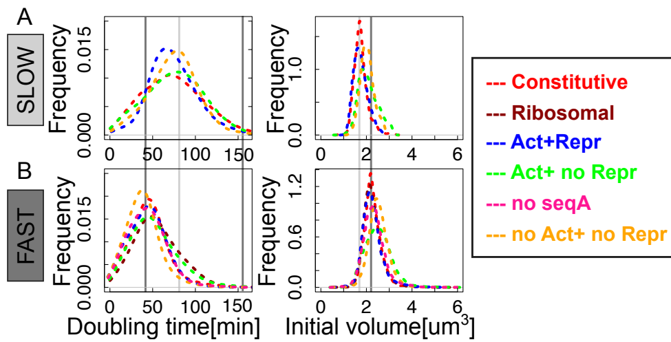
Figure H.5: Doubling time and initial size in consistent in all promoters in both fast and growth conditions A At slow growth average doubling time(left) is centered around 75 mins for all strain while initial size (right) is centered around 1.9 \mu\text{m}^3 B At fast growth average doubling time(left) is centered around 45 mins for all strain while initial size (right) is centered around 2.1 \mu\text{m}^3 .
