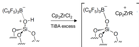
Scheme 5 – Formation of the active species by interaction of \text{Cp}_2\text{ZrCl}_2 with (\equiv\text{SiOH})^{\delta+}[\text{B}(\text{C}_6\text{F}_5)_3]^{\delta-} in presence of an excess of TiBA.
