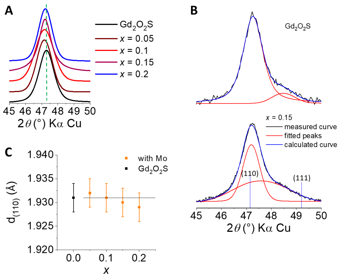
Figure 10 (A) Fitted curves of peak (110) from diffractograms of samples with x from 0 to 0.2. This peak is fitted separately to the rest of each pattern. (B) Peaks (110) and (111) after fitting, in comparison with the measured diffractogram and the calculated curve from the fits. Top: Fits for \text{Gd}_2\text{O}_2\text{S} nanoparticles. Down: fit for \text{Gd}_{1.7}\text{Mo}_{0.3}\text{O}_2\text{S} ( x = 0.15 ) sample, made with \text{Mo}(+I) precursor. The straight lines are from the reference \text{Gd}_2\text{O}_2\text{S} (JCPDS file 00-026-1422). (C) No peak shift between samples with Mo and \text{Gd}_2\text{O}_2\text{S} reference on the graph.
