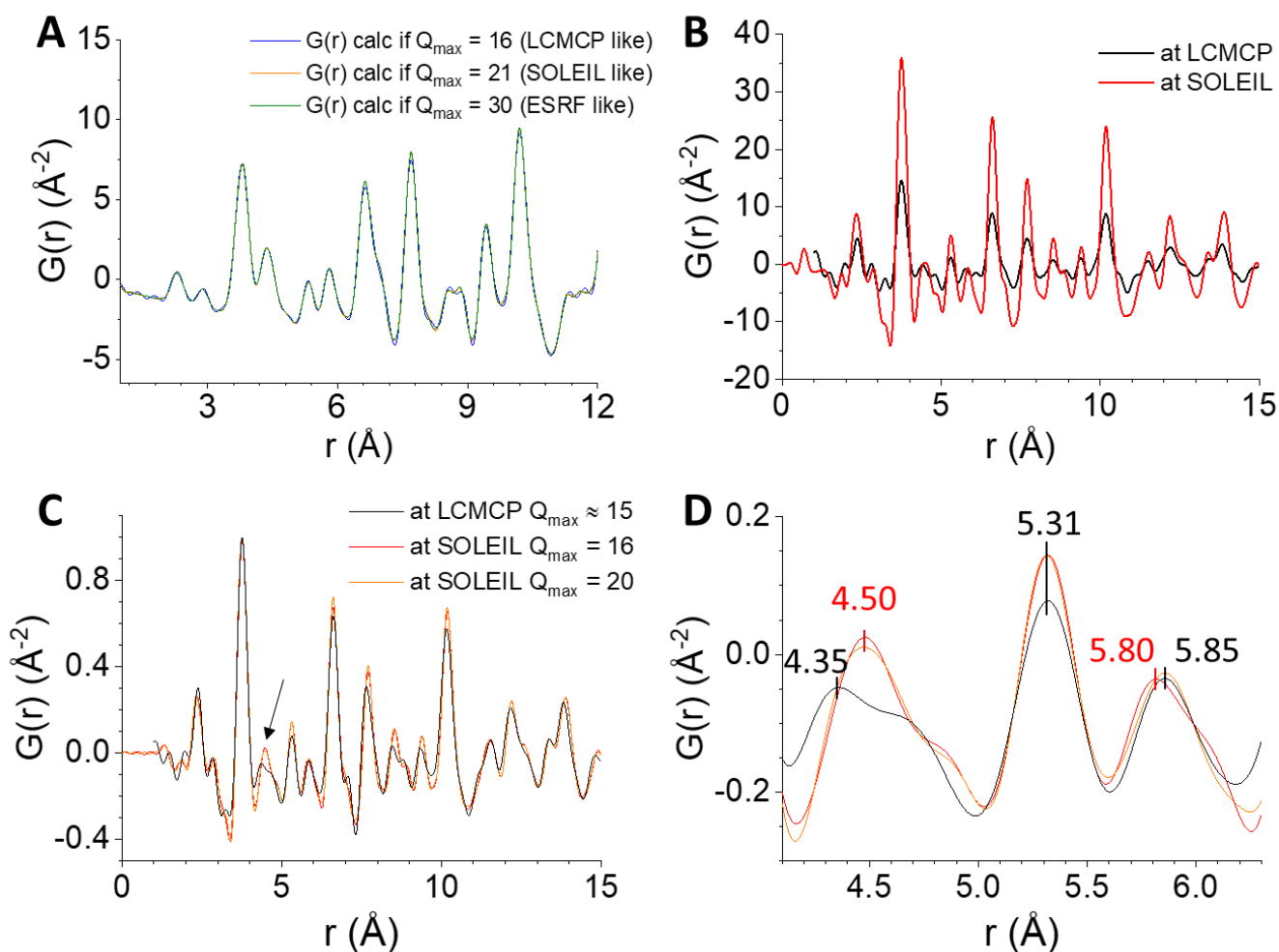
Figure 2 (A) Comparison between calculated G(r) of bulk Gd_2O_2S_{0.5} with different Q_{max} corresponding to the capacity of LCMCP, SOLEIL and ESRF. Comparison of experimental G(r) of the same Gd_2O_2S sample (not annealed) measured at LCMCP and at SOLEIL Synchrotron between: (B) raw data; (C) normalized data with 2 values of Q_{max} for SOLEIL pattern and (D) a zoom of (C) between 4.1 Å and 6.3 Å. The legend is common for (C, D).
