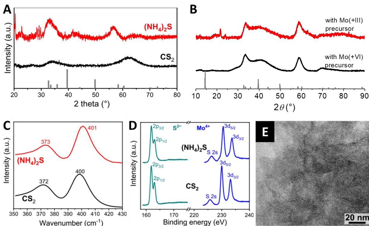
Figure 14 (A) Diffractograms of nanosheets MoS 2 made with MoCl 5 and two different S sources as indicated, compared to the pattern of the bulk MoS 2 (JPCDS 00-037-1492) in gray. (B) Diffractograms of our samples “MoS 2 ” made with S 8 and two different Mo precursors as
