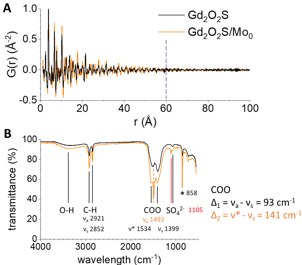
Figure 10 (A) Comparison of PDF patterns between \text{Gd}_2\text{O}_2\text{S} nanoparticles and \text{Gd}_2\text{O}_2\text{S}/\text{MoO}_3 , both measured at LCMCP, patterns extracted up to 100 Å with Q_{\max} = 15 . (B) Comparison of IR spectra measured in ATR mode between \text{Gd}_2\text{O}_2\text{S} nanoparticles and \text{Gd}_2\text{O}_2\text{S}/\text{MoO}_3 . The legend in (A) is common for both (A, B).
