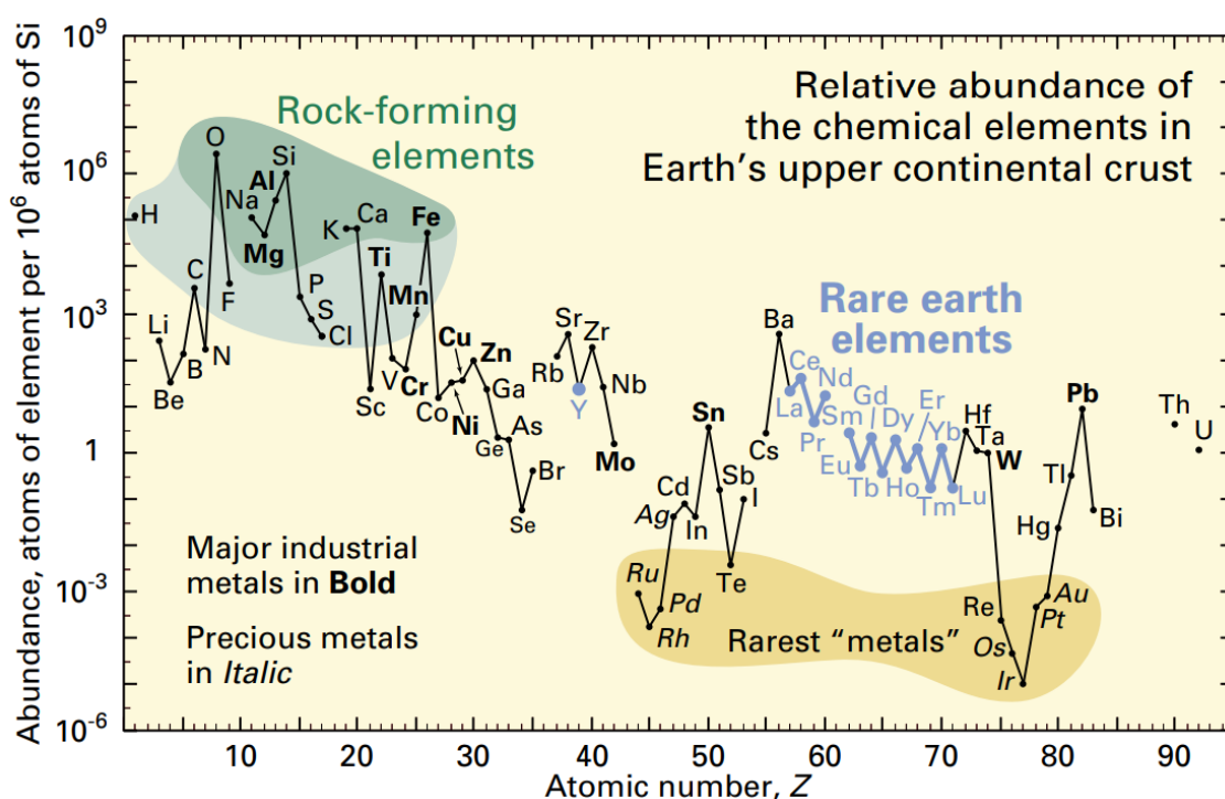
Figure 7 Figure from a fact sheet by USGS in 2002. 45 Abundance (atom fraction to 10^6 atoms of Si) of the chemical elements in Earth's upper continental crust as a function of atomic number. Many of the elements are classified into (partially overlapping) categories: (1) rock-forming elements (major elements in green field and minor elements in light green field); (2) rare earth elements (lanthanides, La–Lu, and Y; labeled in blue); (3) major industrial metals (global production > \sim 3 \times 10^7 kg/year; labeled in bold); (4) precious metals (italic); and (5) the nine rarest "metals"—the six platinum group elements plus Au, Re, and Te (a metalloid).
