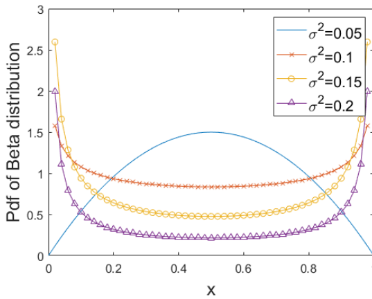
Figure 4.9: Pdf of p for different \sigma^2(p) . Figure 4.10: R_{X_\infty^p}(x|f_p) as a function of E[p] = 0.5 .
