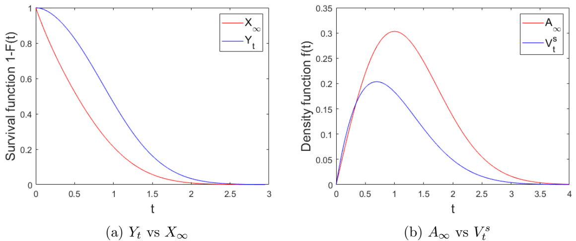
Figure 3.5: Y_t , X_\infty , V_t^s and A_\infty in a BP process.
