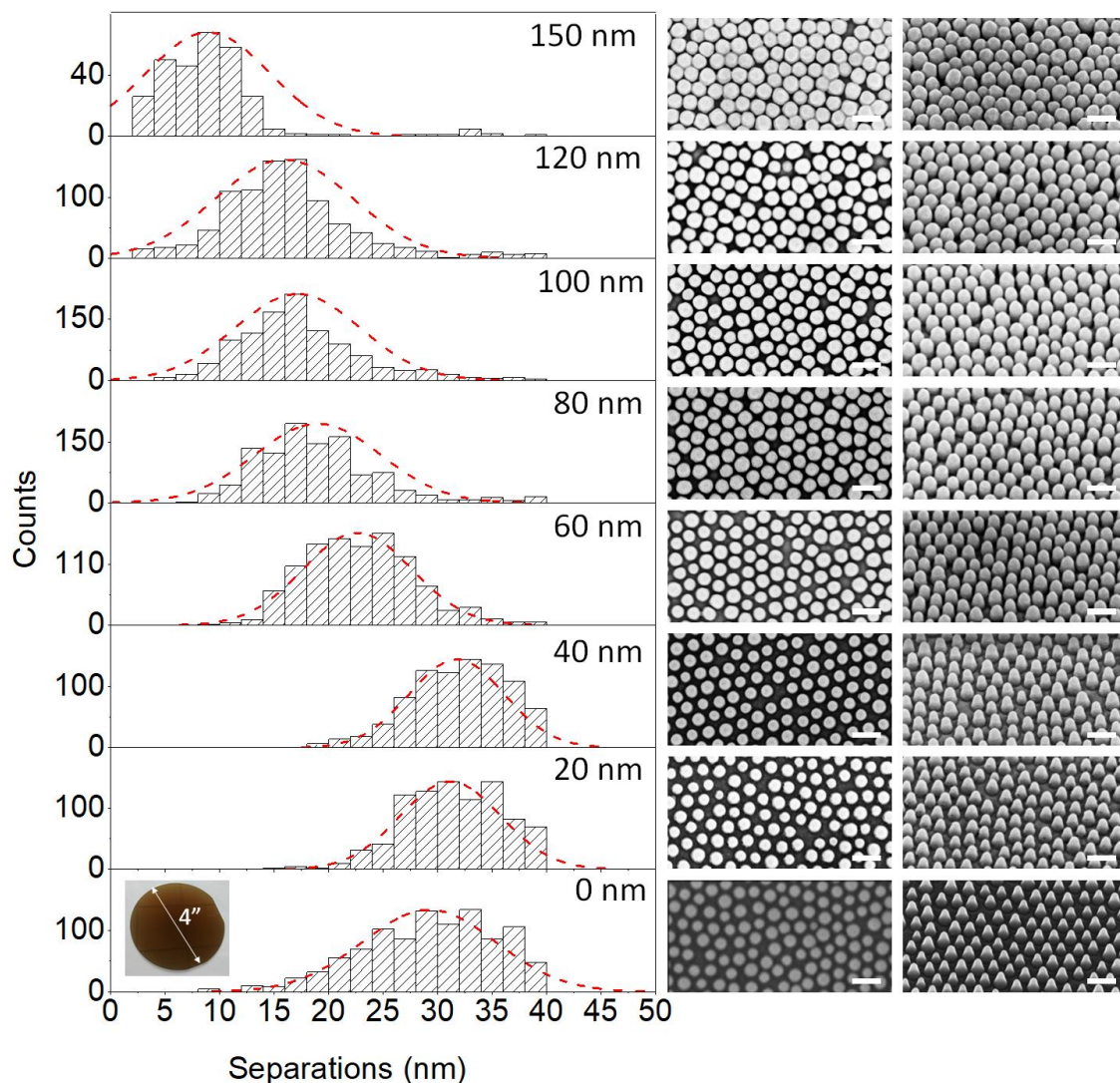
Figure 6.1. Histograms of inter-pillar gap distances as a function of the thickness of sputtered gold films, and the SEM images of the nanopillar arrays acquired in the top and tilt view ( 30^\circ inclination). The scale bars indicate 200 nm. Picture of 4" uniform nanopillar arrays on 4" Si wafers is shown as an inset.
