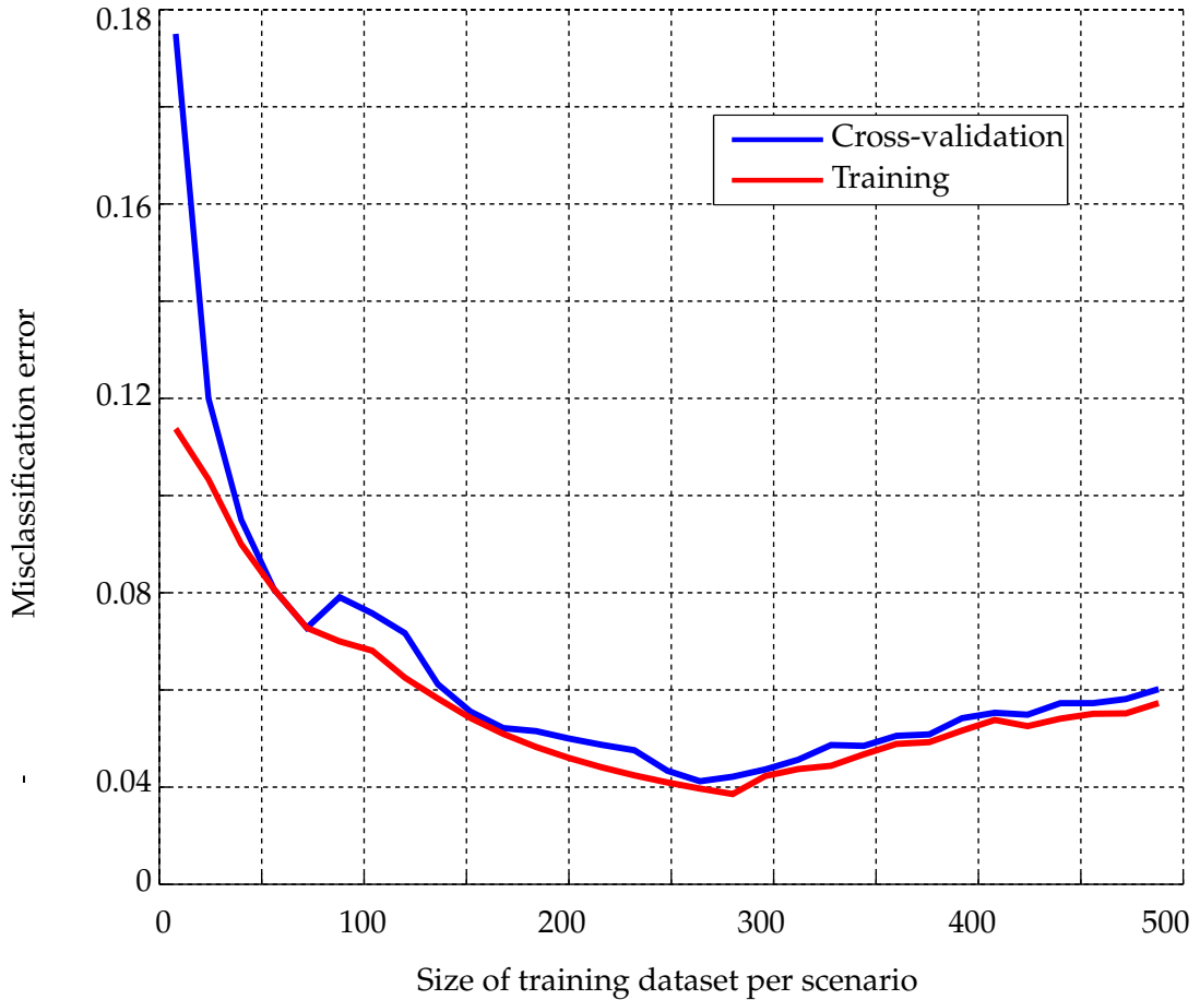
FIGURE 3.11: Learning curve of the proposed Bayesian Network
