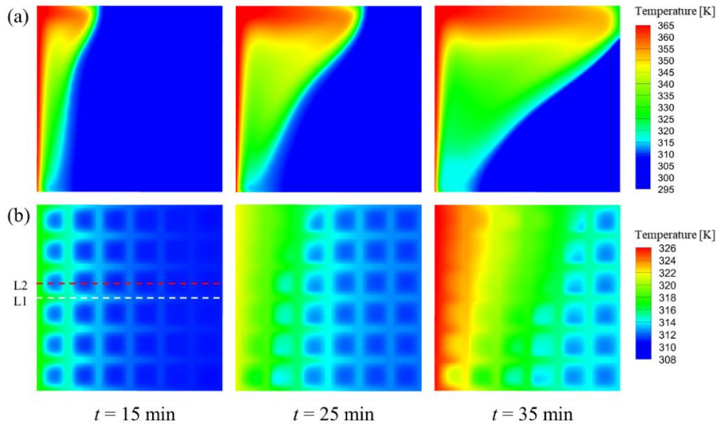
Fig. 3.11. Temperature field of (a) pure paraffin and (b) PCM composite
