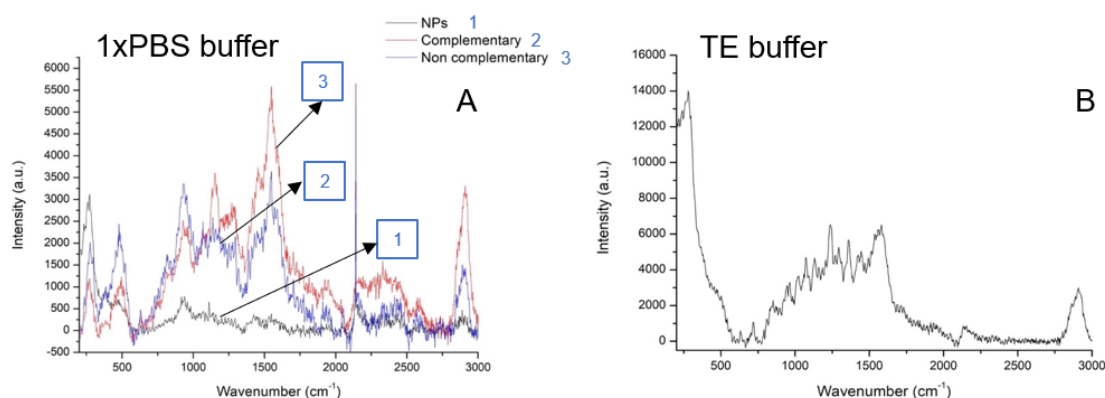
Figure 3. 13 SERS spectra of annealed AuNPs on the coverslips glass (A) after biofunctionalization with DNA-probe and complementary in 1xPBS buffer, 60 sec x 3 times filter D0.3 and (B) DNA-thiol probe in TE buffer after incubation with 10 \mu L overnight 4 ^{\circ} C, 10 sec x 3 times, filter D0. The in-set picture is the sample after biofunctionalization with Thiol-Probe in 1 x PBS buffer (a) and in TE buffer (b) on AuNPs.
