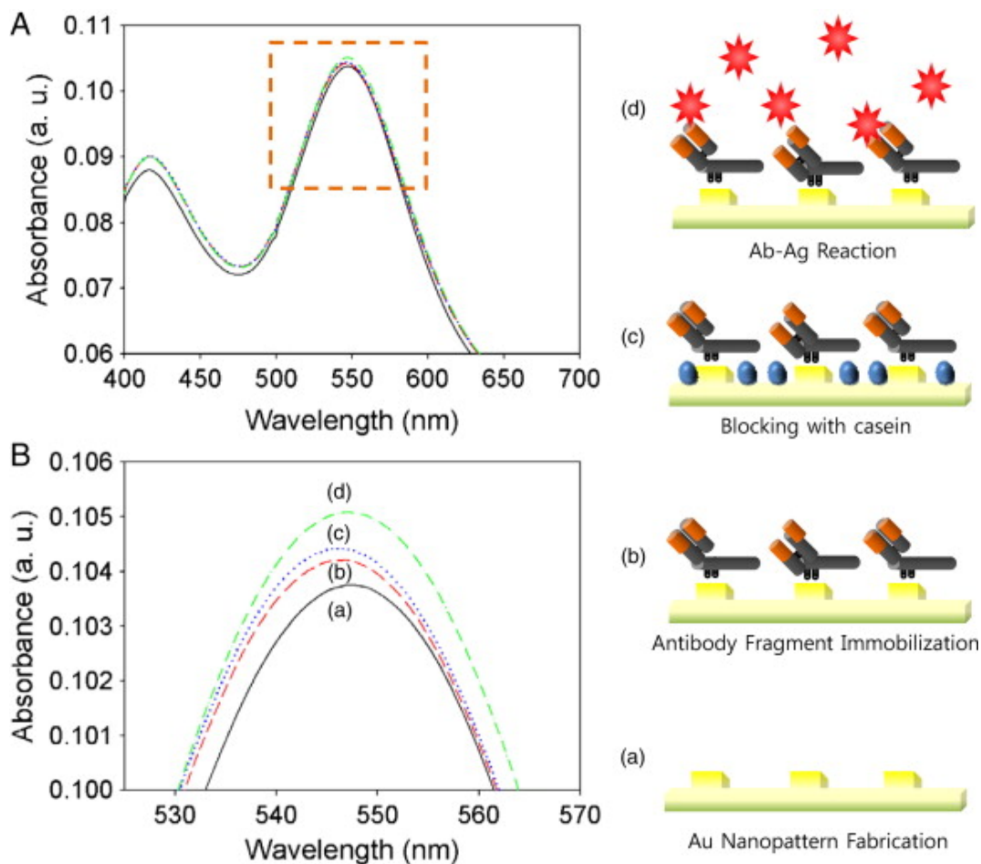
Figure 1.13 LSPR detection based on gold nanoparticle array platform. (A) Optical characteristics of the (a) bare Au nanopattern on ITO substrate, (b) fragmented antibody immobilized layer, (c) blocking with casein, (d) HIV-1 VLPs immuno reacted layer, respectively. (B) LSPR spectra of zoomed part. 155
