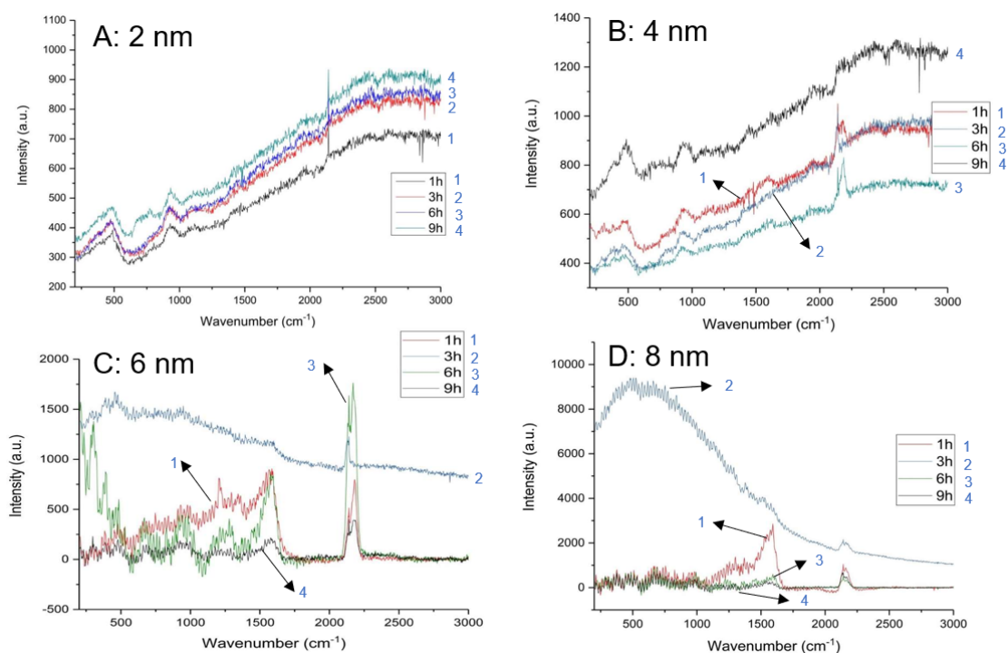
Figure 3.9 SERS signals of naked annealed gold films on coverslips at 550 °C for different periods with different thickness of evaporated gold film, 2nm (A), 4 nm (B), 6 nm (C) and 8 nm (D), respectively.
