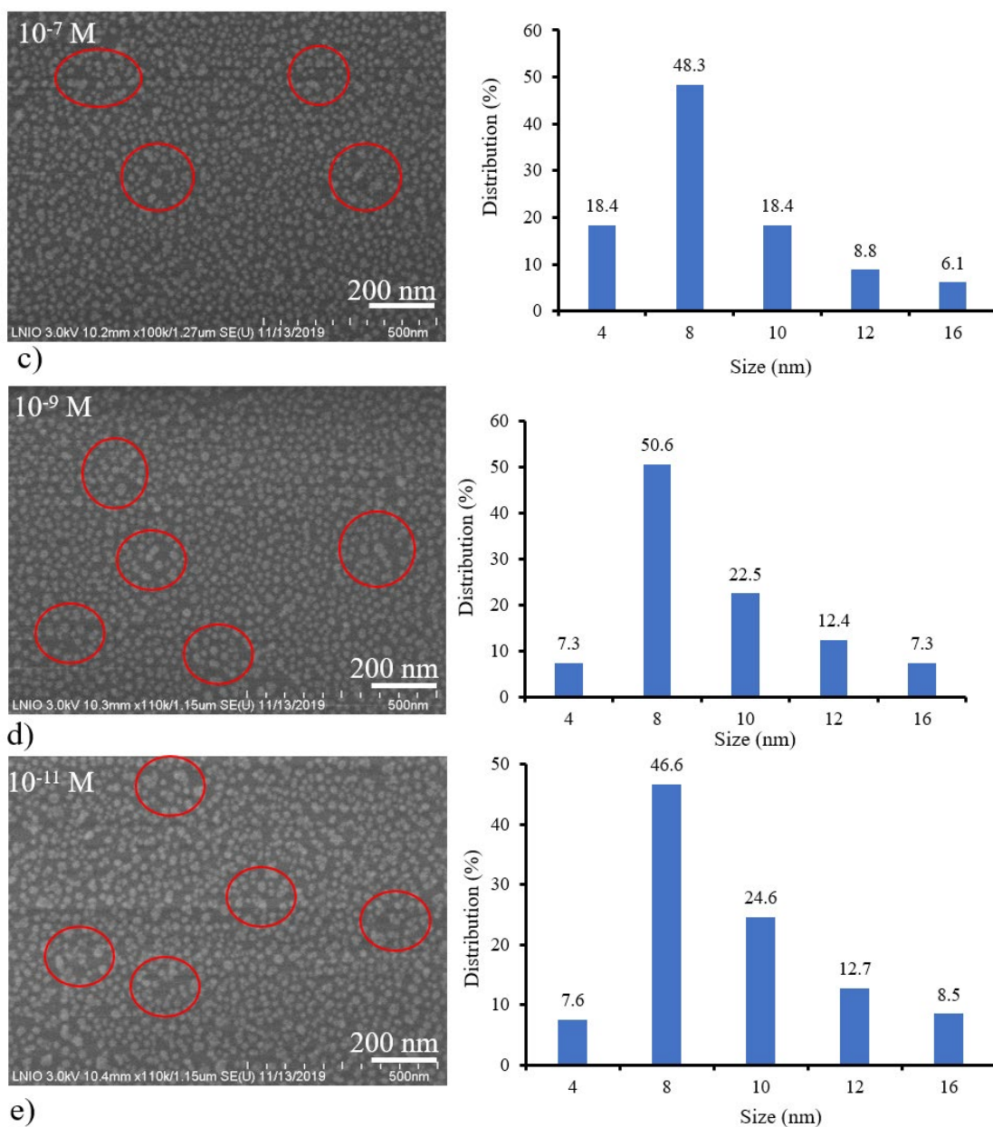
Figure 5. 7 SEM images and the size distributions of annealed gold nanoparticles modified by BPE molecules with 5 different concentrations, respectively. a) 10^{-3} M BPE; b) 10^{-5} M BPE; c) 10^{-7} M BPE; d) 10^{-9} M BPE; e) 10^{-11} M BPE. The SEM measurements were performed under cleanroom conditions at 21 °C.
