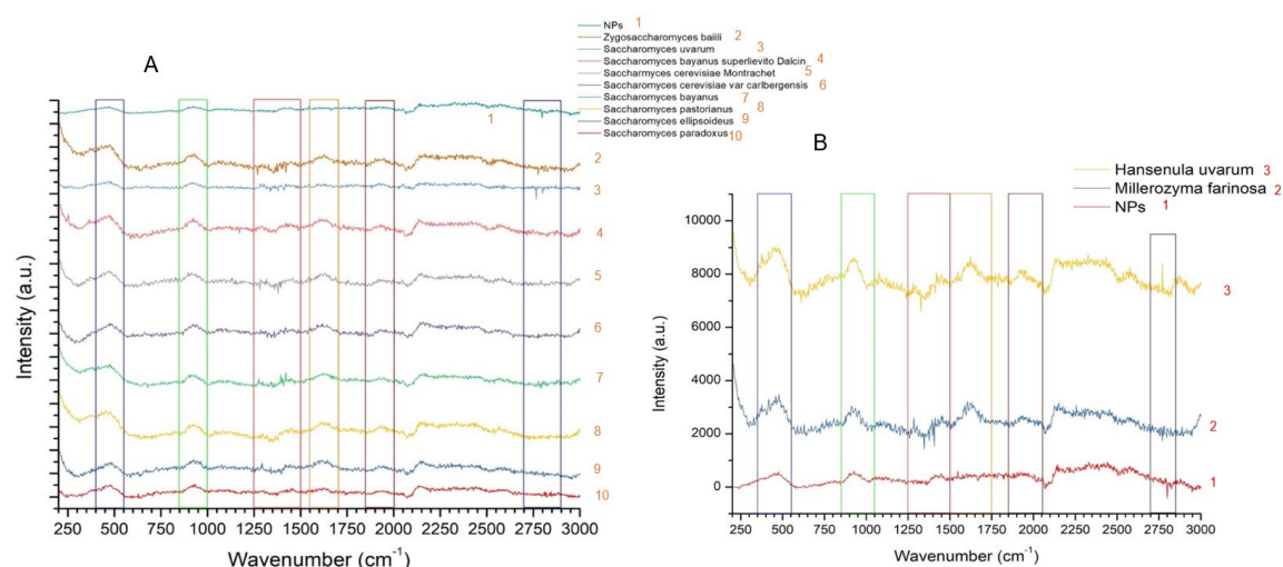
Figure 3. 15 SERS spectra of different microorganisms of Saccharomycetales (A), and Debaryomycetaceae ( Millerozyma farinosa ) and Saccharomycodaceae ( Hansenula uvarum ) (B), using an acquisition time 10 sec x 3 times with D0 filter and a drop (2 \mu L) was deposited on round AuNPs coverslip NPs, respectively.
