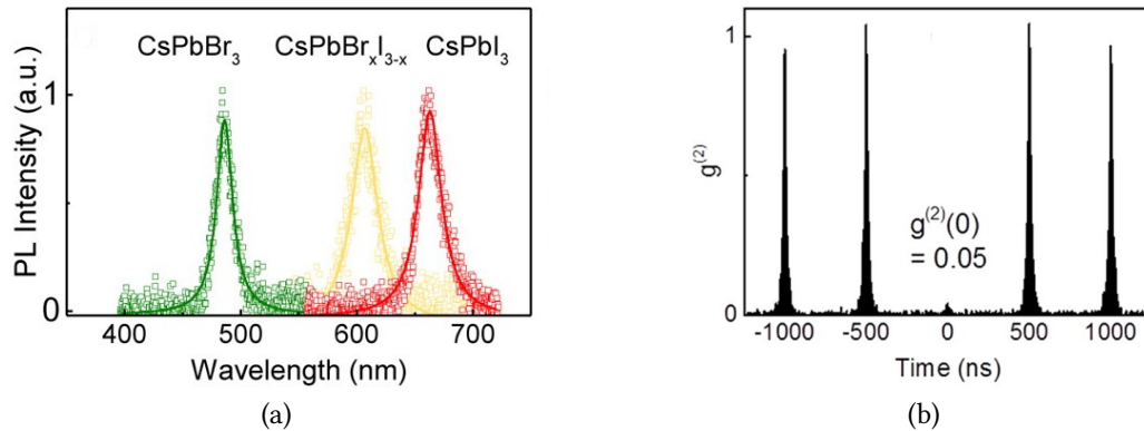
Figure 2.3 – (a) Different emission spectra with different composition of perovskite nanocrystals. (b) g^{(2)}(\tau) measurement of light emitted from a single perovskite nanocrystal, excited with a pulsed laser. (credits: Park et al. [4]).
