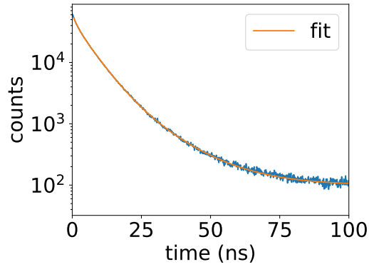
Figure 2.24 – Lifetime of a single perovskite nanocrystal, fitted with a triple exponential decay model. We obtain 1.4 ns, 6.1 ns and 14.7 ns, corresponding respectively to the lifetimes of the biexciton, grey and neutral emission states.
