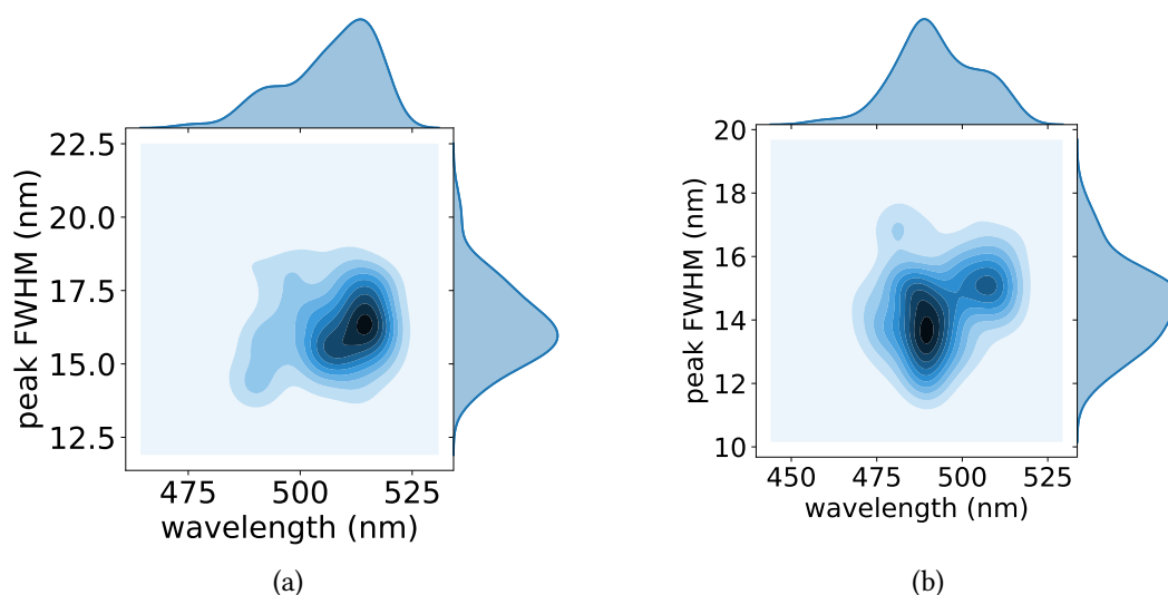
Figure 2.12 – Distribution of central wavelength emission and the peak Full Width Half Maximum (FWHM) for the samples A (a) (calculated on 135 emitters) and B (b) (calculated on 74 emitters).
