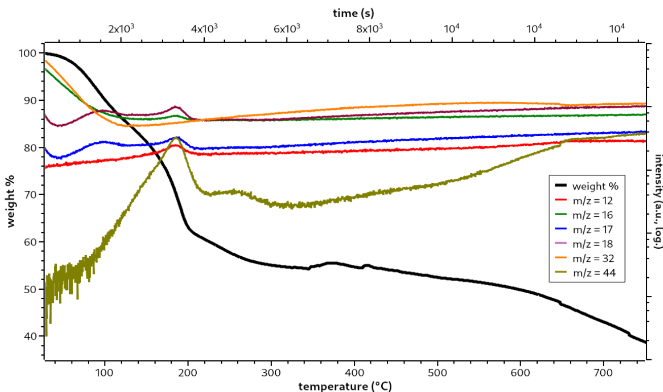
Figure 2.10: TG analysis of a GO sample under N 2 flow, coupled with mass spectrometry.
