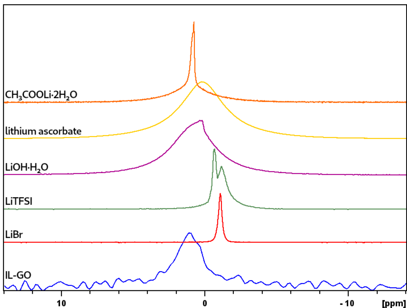
Figure 3.7: 7 Li NMR spectra of the functionalized binary material and the standards used for comparison (LiBr, LiTFSI, LiOH·H 2 O, lithium ascorbate and CH 3 COOLi·2H 2 O). The intensities of the signals have been normalized for the sake of comparison.
