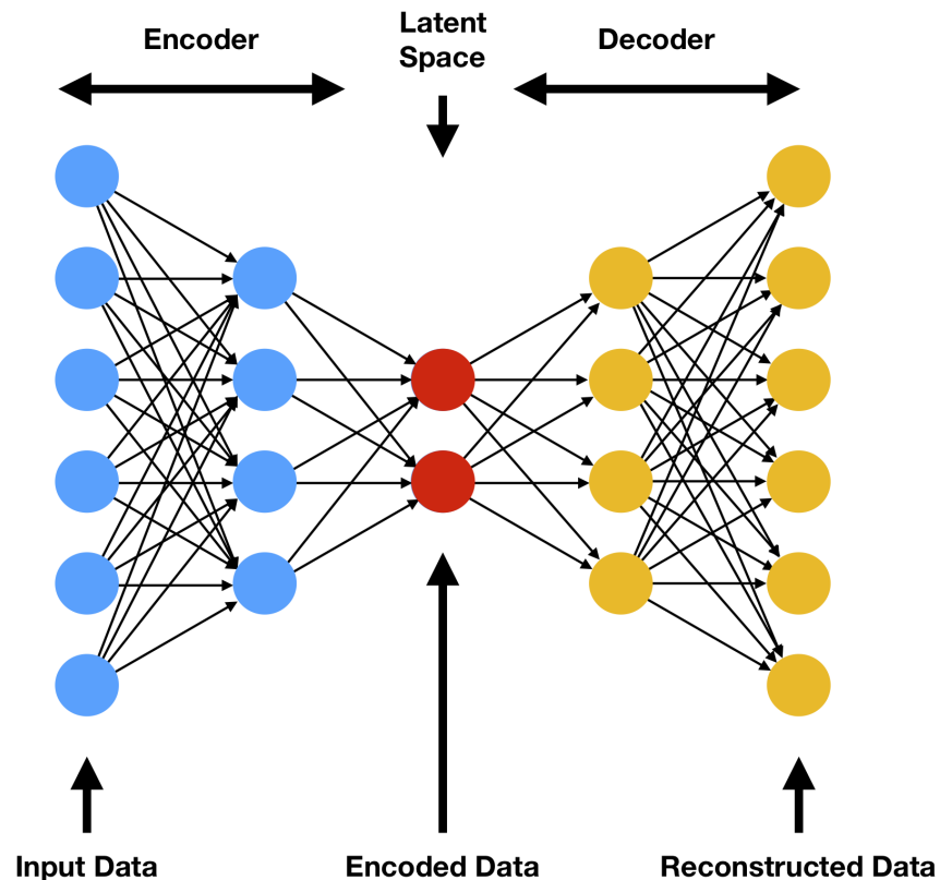
FIGURE 3.10: Autoencoder ; all layers are fully connected layers and latent Space is the bottleneck layer
