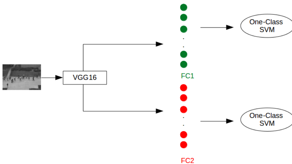
FIGURE 3.4: Feature extraction of shapes
