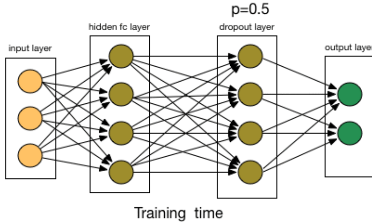
FIGURE 4.9: Dropout
