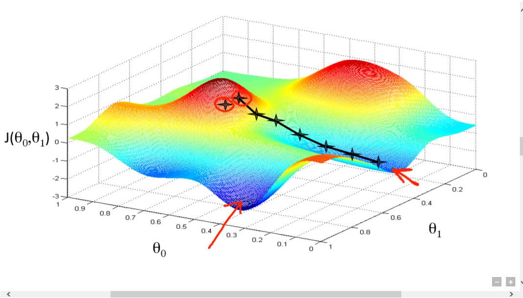
FIGURE 4.2: Gradient Descent
