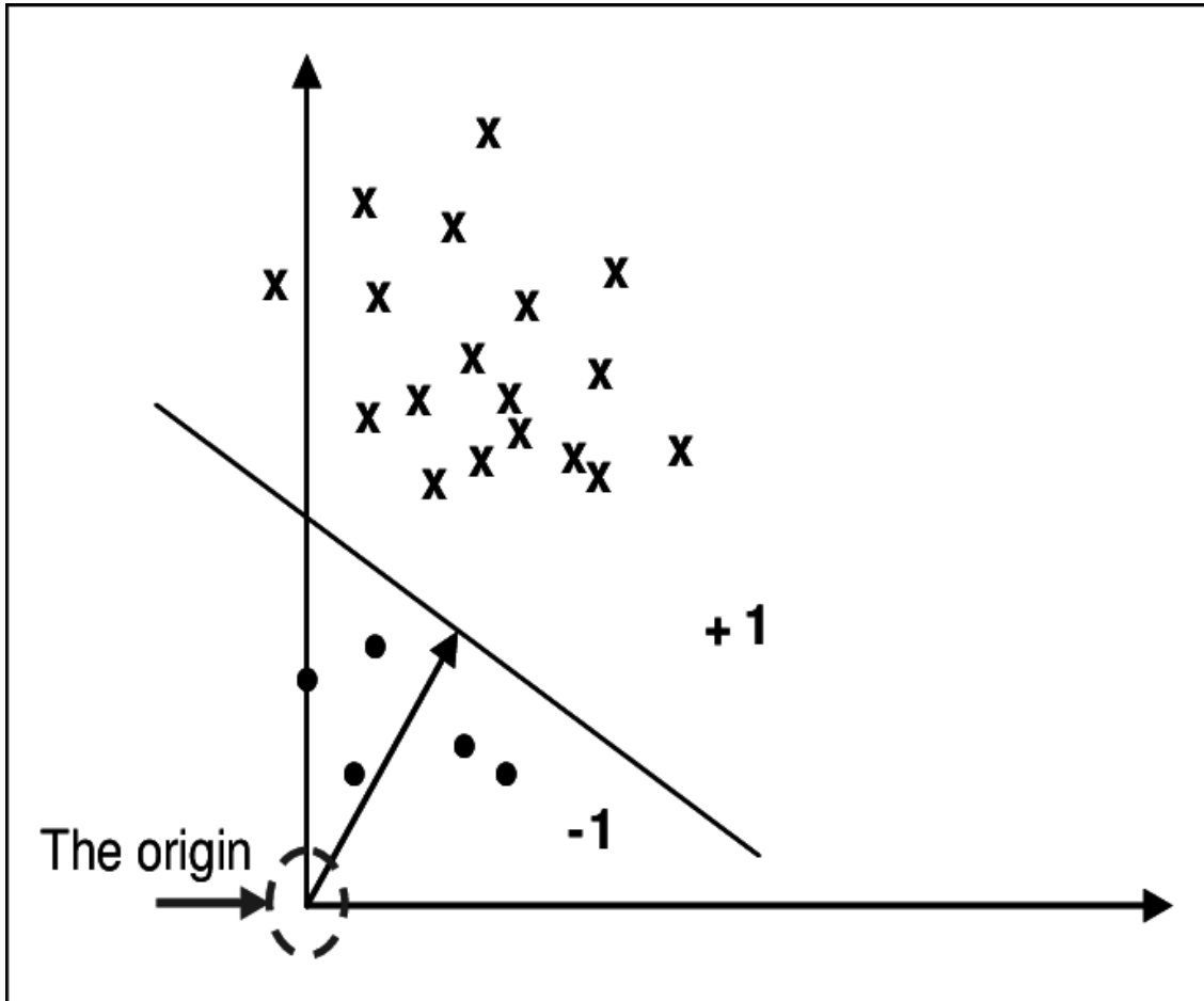
FIGURE 3.5: One-Class SVM
