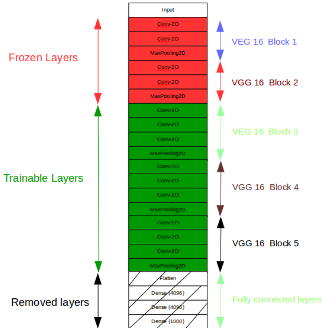
FIGURE 3.13: VGG 16 architecture used for fine-tuning one class objective
