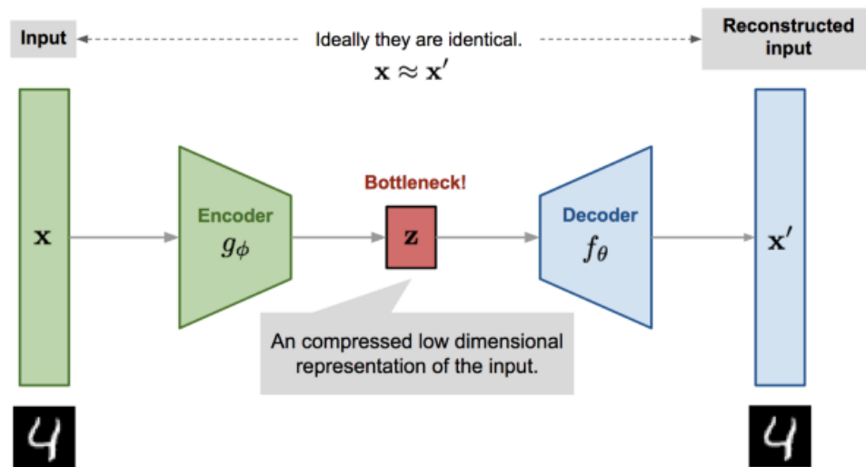
FIGURE 2.5: The building architecture for an auto-encoder
