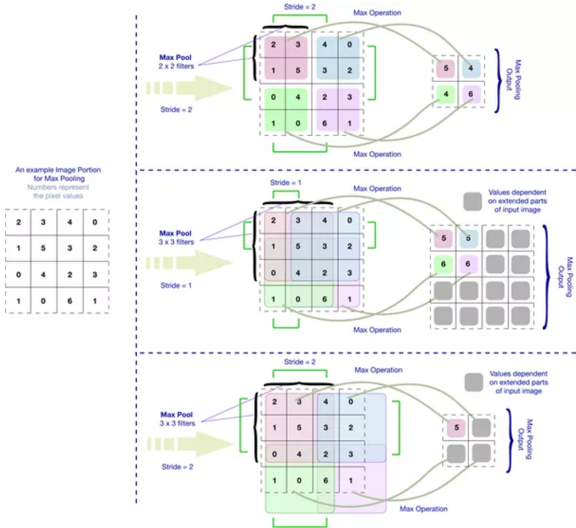
FIGURE 2.4: Example of pooling layers
