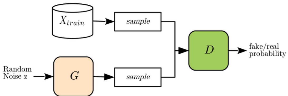
FIGURE 2.6: Generative Adversarial Network (GAN)
