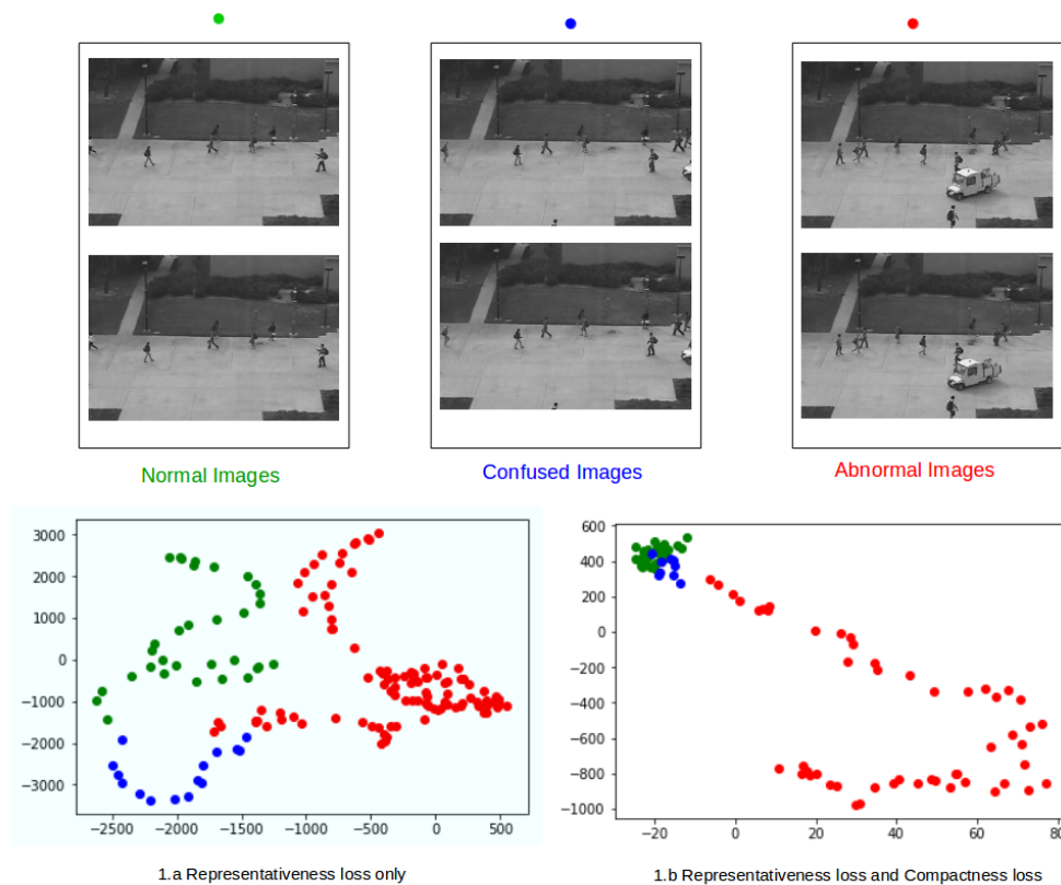
FIGURE 3.19: Compactness loss importance
