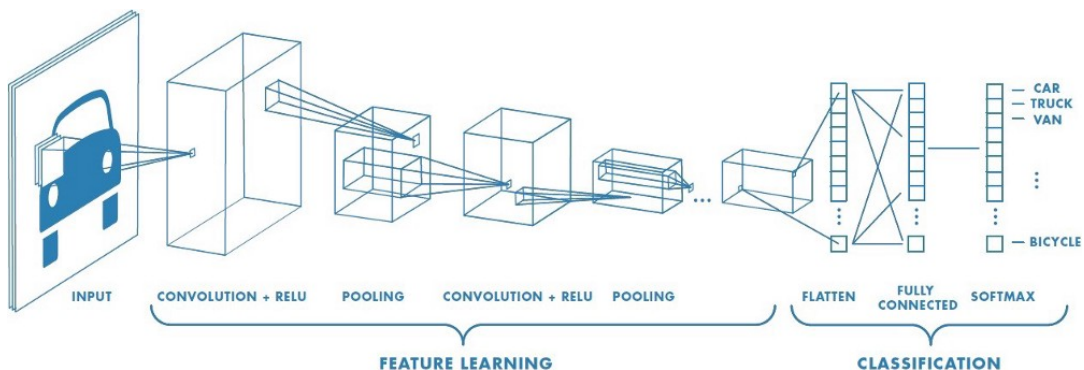
FIGURE 2.2: CNN
