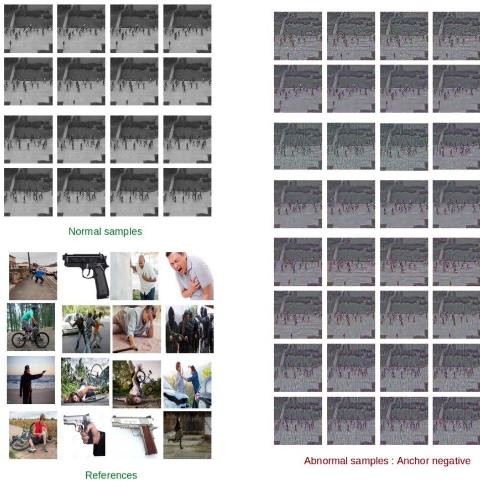
FIGURE 5.2: art transfer
