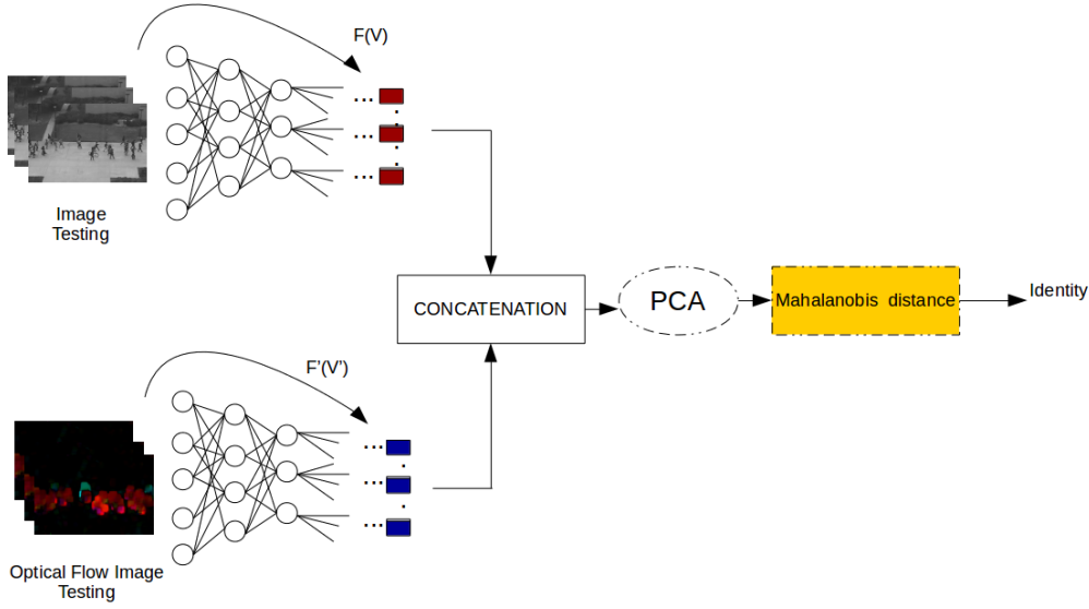
FIGURE 3.18: Classification flowcharts
