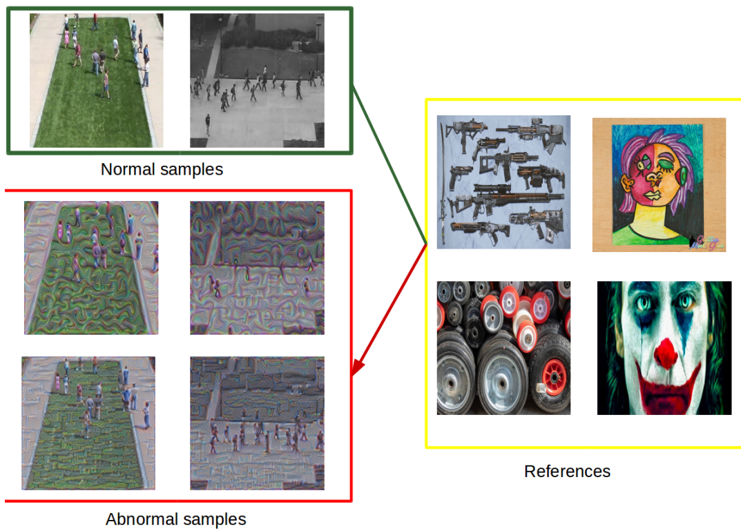
FIGURE 5.1: Art transfer
