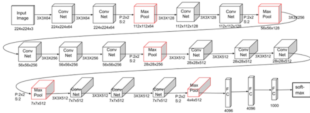
FIGURE 3.3: VGG16 Architecture
