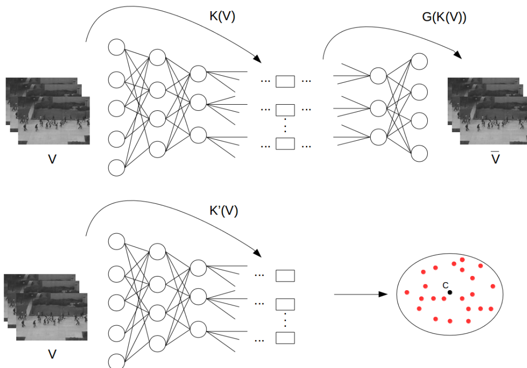
FIGURE 3.15: The first training method : Cascade objectives
