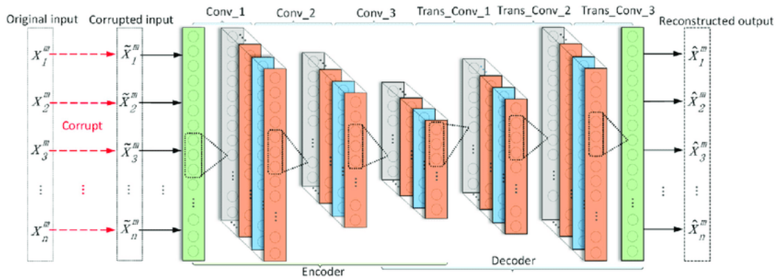
FIGURE 3.11: Structure of a 1-D denoising convolutional auto-encoder Liu et al., 2019.
