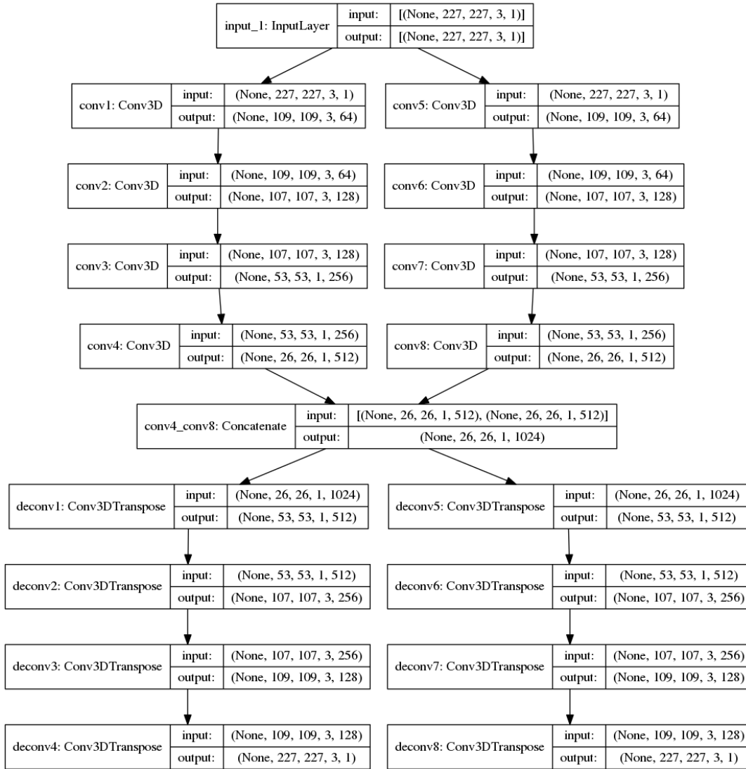
FIGURE 6.5: Notre architecture
