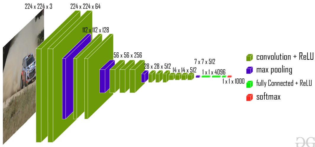
FIGURE 3.2: VGG16 Configuration
