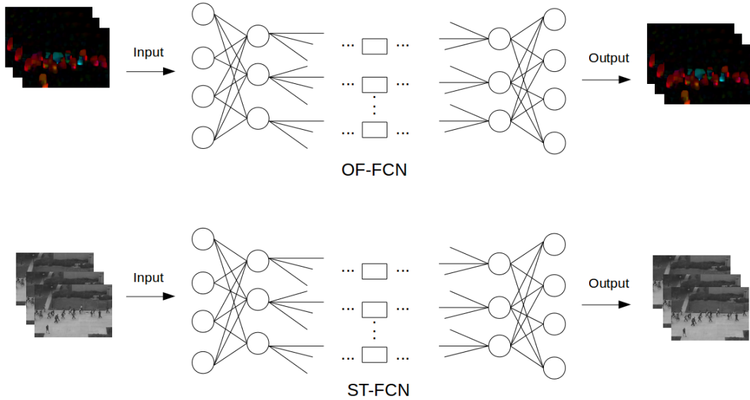
FIGURE 6.4: Architecture TS-FCN 1
