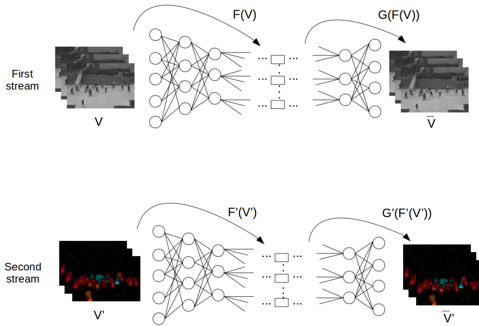
FIGURE 3.14: Two stream learning
