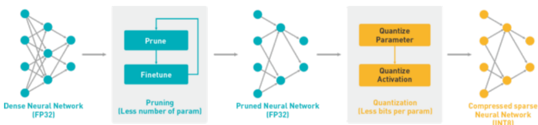
FIGURE 4.8: Deep Learning situations after trained a model
