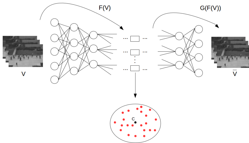
FIGURE 3.16: The second training method : pseudo-parallel objectives
