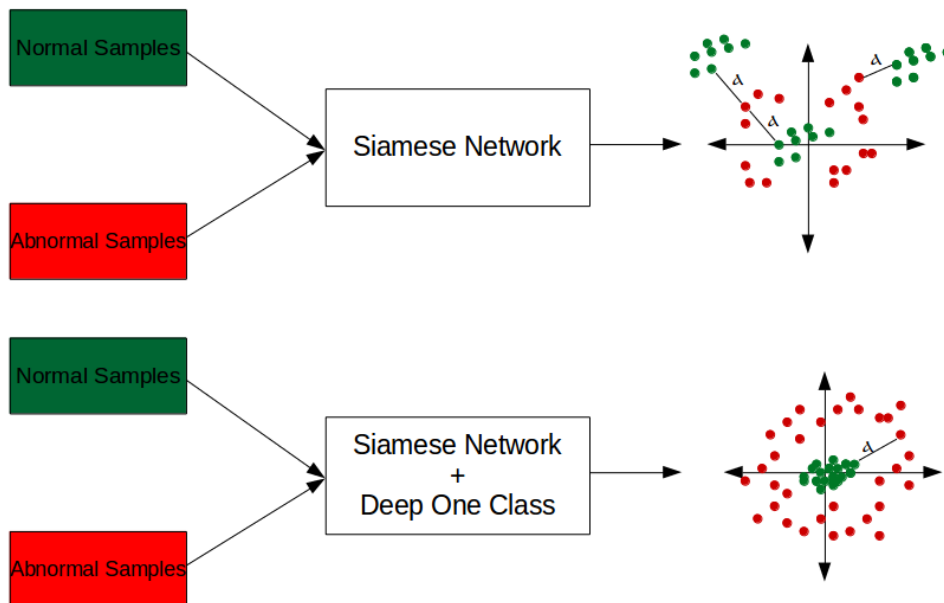
FIGURE 5.3: Deep One class
