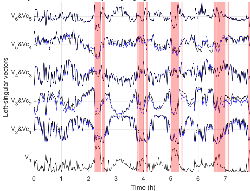
Figure 4.12: Illustration of the effect of mean-centring on K_{TS} left-singular vectors, which become shifted in the same way as eigenvectors in Figure (4.11). Representations here relate to the same target as Figure (4.11), and red areas correspond to target ground-truth REM.
