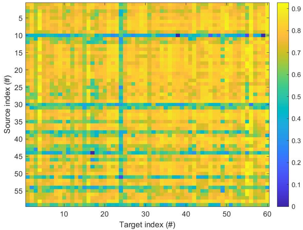
Figure 6.6: Prediction value for each (source, target) couple of recordings. The performance predictor is here the correlation between source detector output and KTATL.
