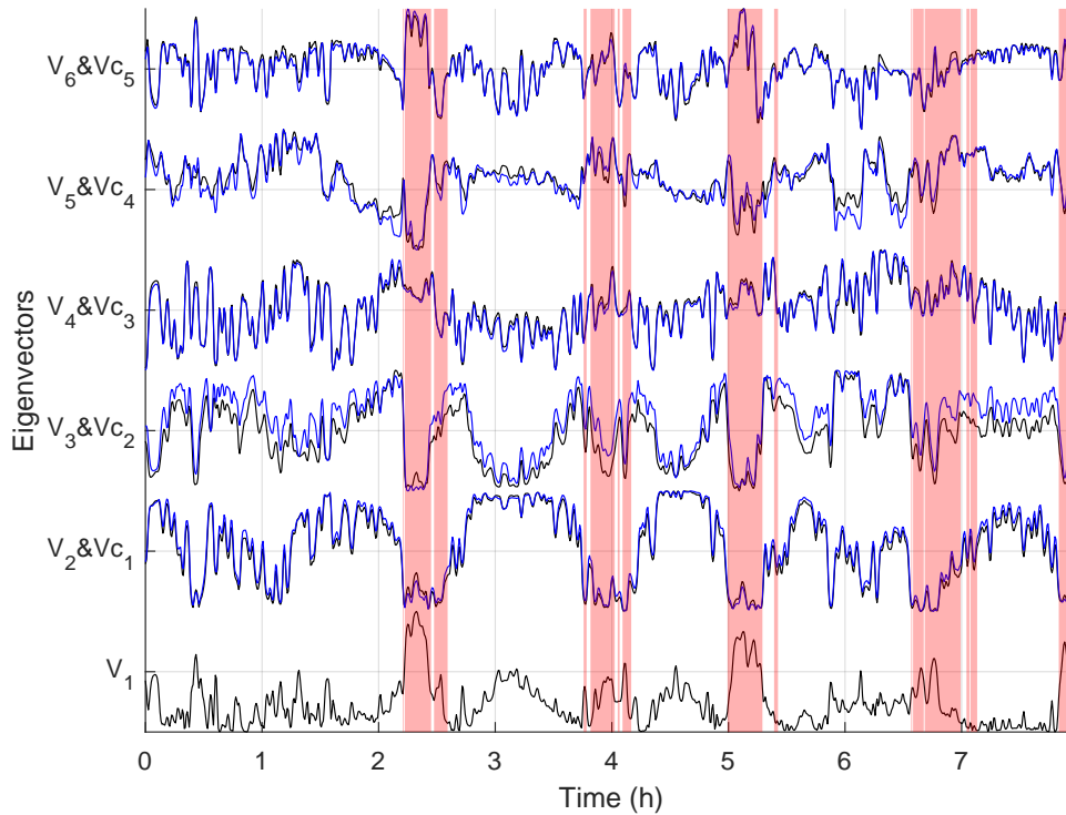
Figure 4.11: Illustration of the effect of mean-centring on K_{TT} eigenvectors, which become shifted: the second eigenvector of K_{TT} is similar to the first of K_{TTc} , the second to the third, and so on. This property is studied in [56]; red areas correspond to REM in the corresponding target ground-truth.
