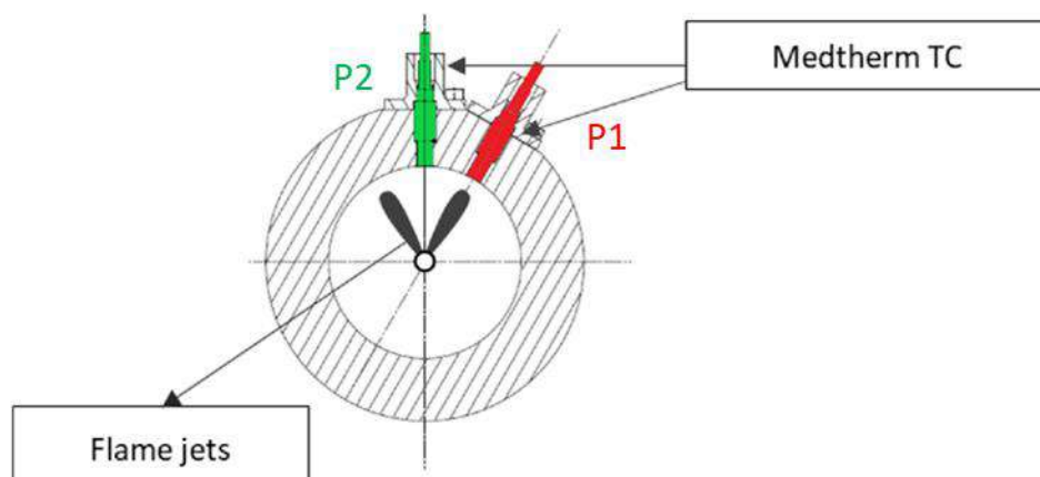
Figure 158: Two different locations of surface temperature measurement
