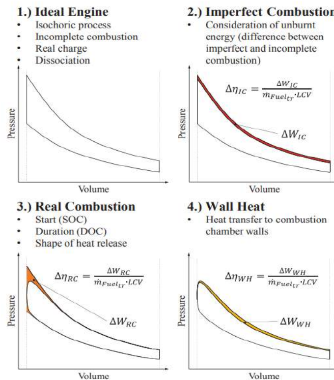
Figure 5: Some losses in constant volume heat addition combustion cycles [5]
