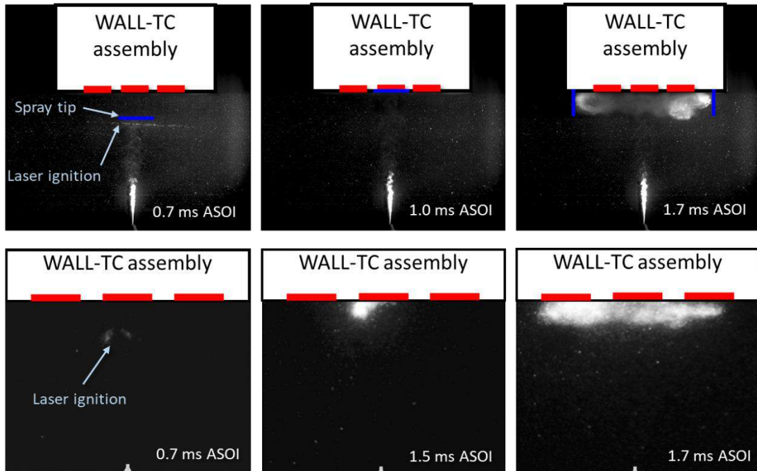
Figure 152: Simultaneous Mie-scattering images (Top) showing the spray (liquid and gaseous) and OH* images (Bottom) showing the reaction regions for modified reactive Spray A with laser ignition. t = 0 corresponds to the start of injection (SOI)
